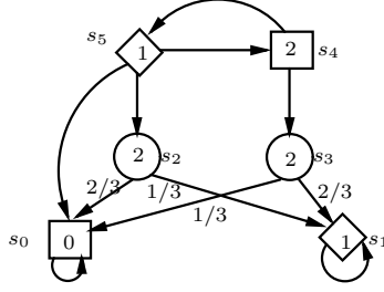
Figure 2: A 2\frac{1}{2} -player parity game.
