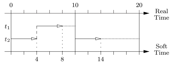
Figure 6: An execution trace of the S code of Figure 5
