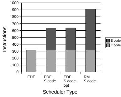
Figure 18: E and S code size for 100 tasks
