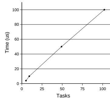
Figure 19: E code execution overhead
