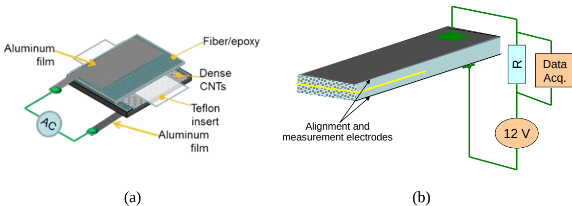
Figure 18. Method of manufacture (a) and electrical test (b) of interlaminar fracture toughness specimens with 0.125 wt% VGCNT/epoxy.
