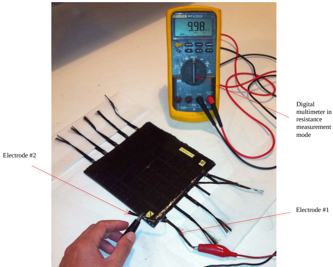
Figure 24. Resistance measurements of CB-filled glass/epoxy composite using carbon tows.
