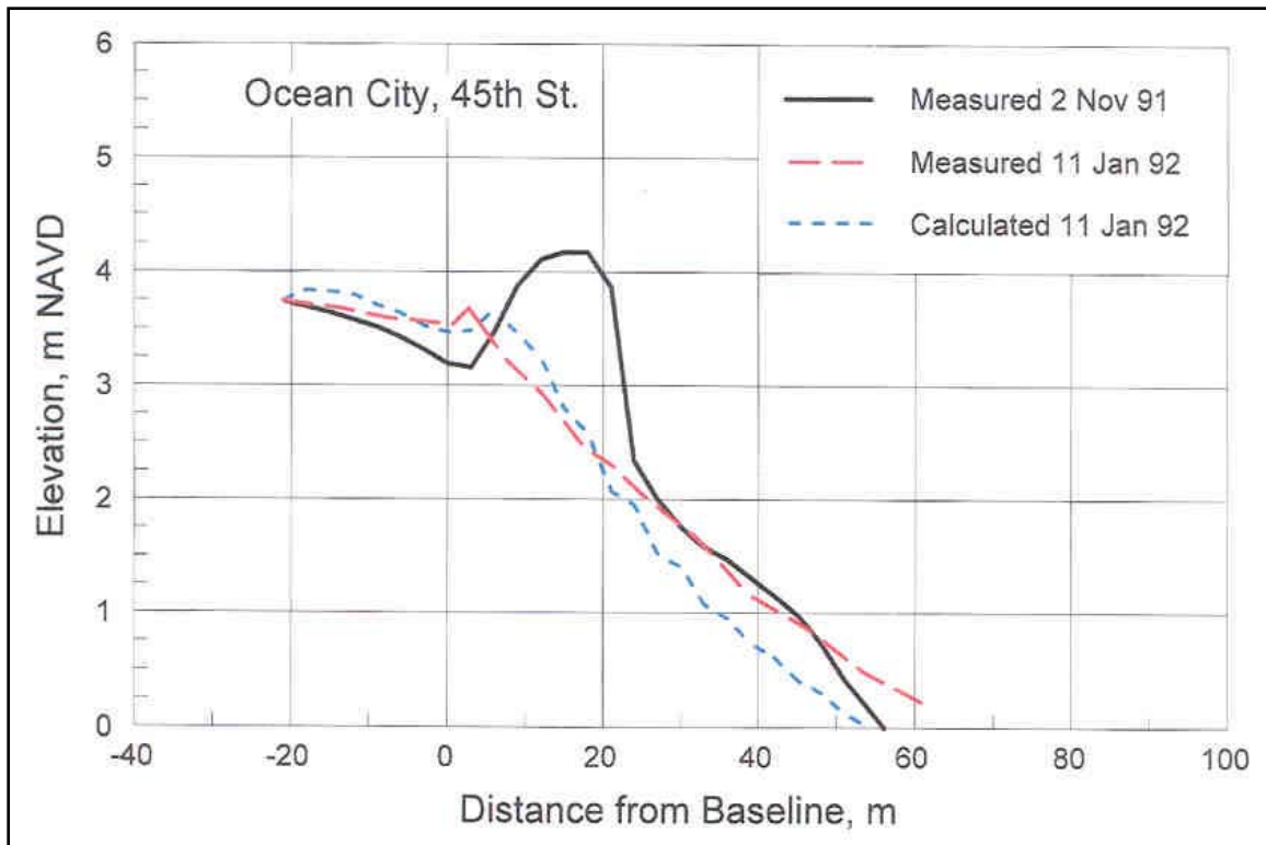
Figure 6. Calculation of dune erosion and overwash, 45 th Street (note: ocean is to right and bay is to left in this and all subsequent profile figures).
