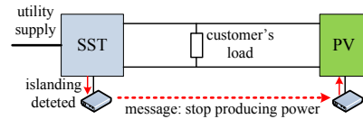
Fig. 7. Anti-islanding procedure in Green Hub.
