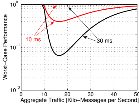
Fig. 5. Uncoordinated communication: worst-case \mathbb{P}(D_k > \sigma) versus \gamma_k with delay thresholds of 10ms and 30ms. ( N_f=10 , N_c=2 , T_L=1\text{ms} , \rho=0.1 , and \tau=1\mu\text{s} .)
