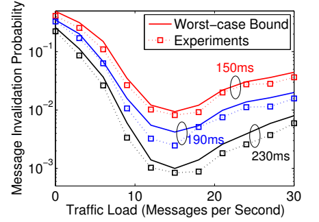
Fig. 11. Coordinated: Message invalidation probability with different delay thresholds.
