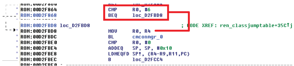
Figure 4.6: Connection Manager Object Class Test.
