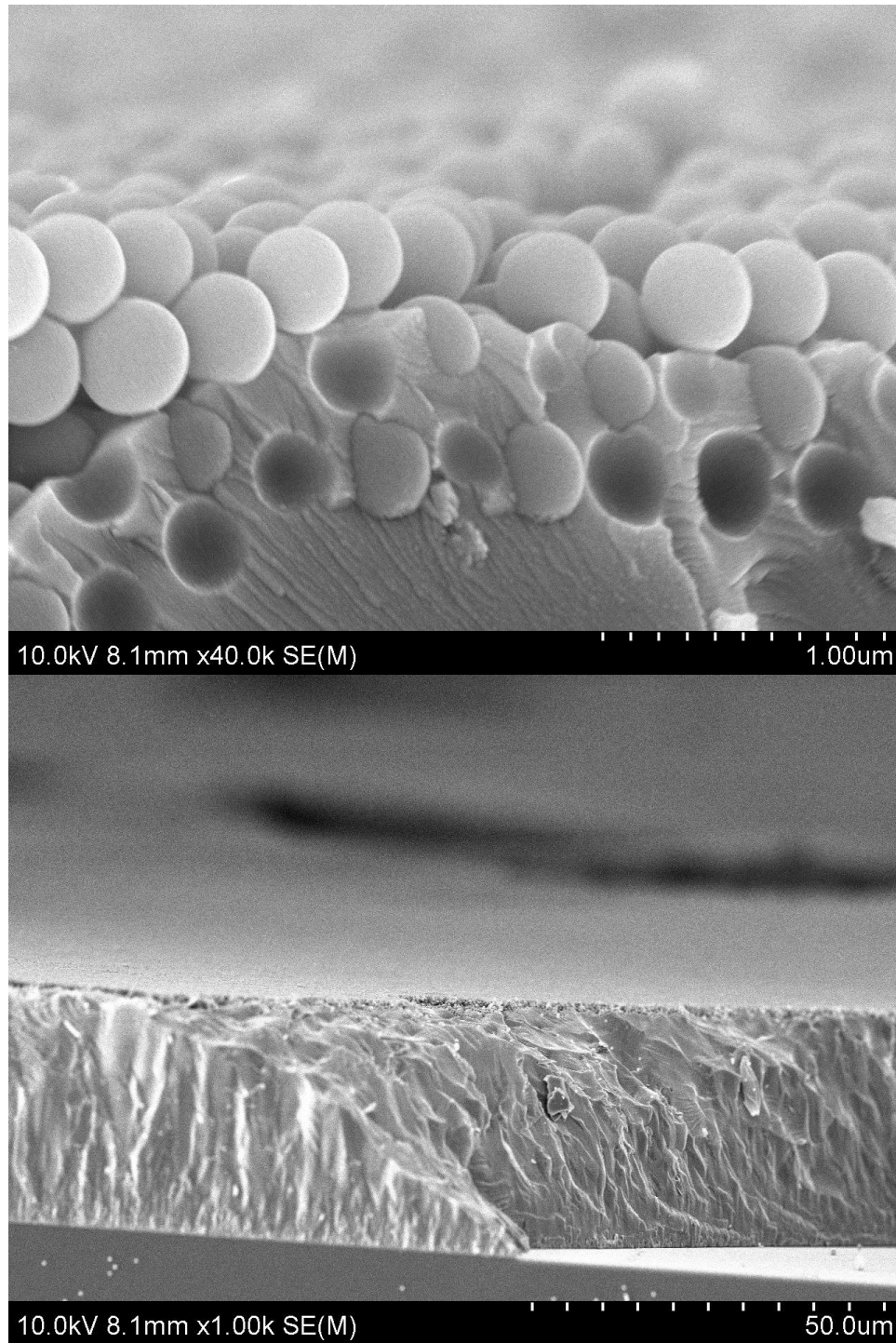
Figure 3.4 Cross-sectional SEM image of successful deposition of Cu 2 O inside the opal structure (TOP). The opal structures were grown onto cuprous oxide film deposited onto silicon before infilling the structure with electrodeposition. Bottom image is the SEM cross-sectional image of the Cu 2 O film on which the opal was grown.
