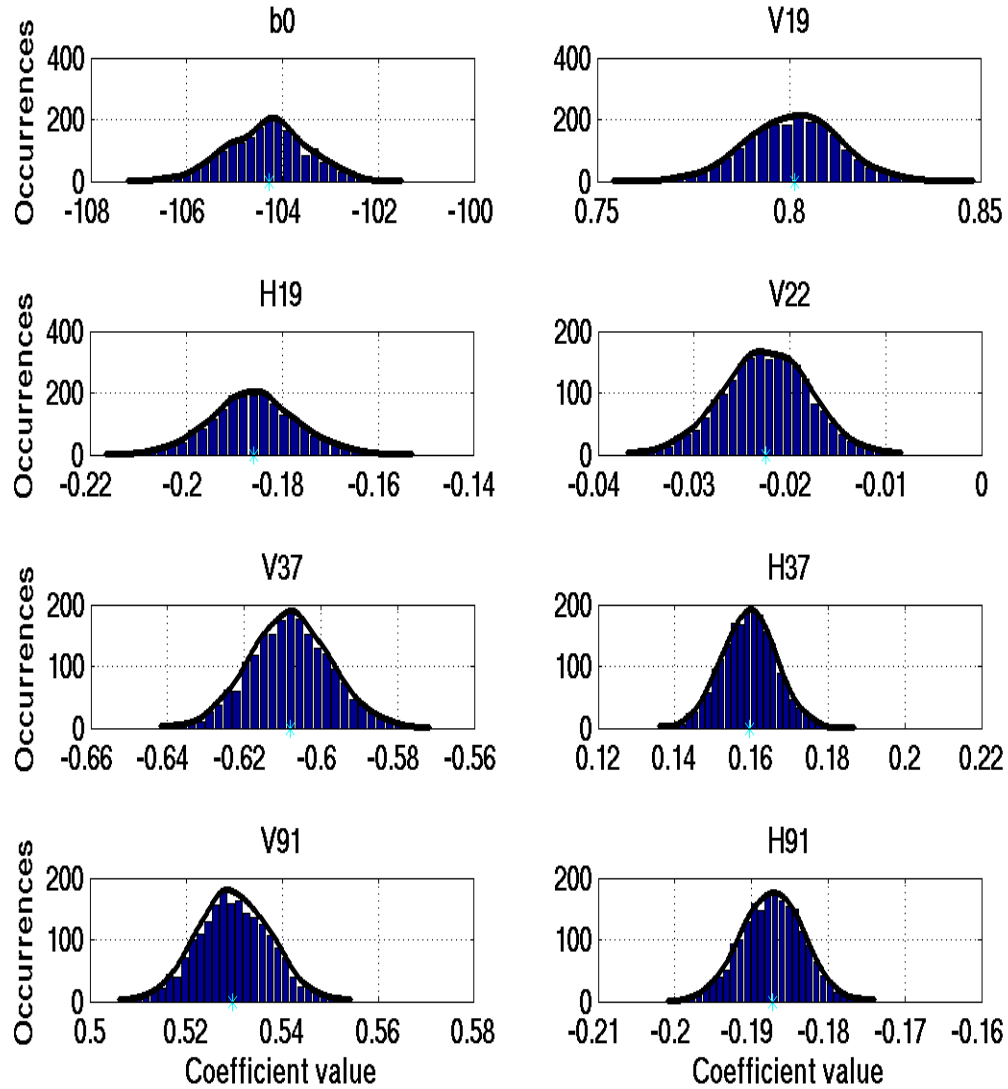
Figure 3- 1: Example of the bootstrapped MLR coefficients for the QA product from DMSP F18. 2000 sets of randomly-sampled MLR coefficients were used to selected the most-probable coefficient, as indicated by the “*” along the x-axis, for the particular satellite and channel.
