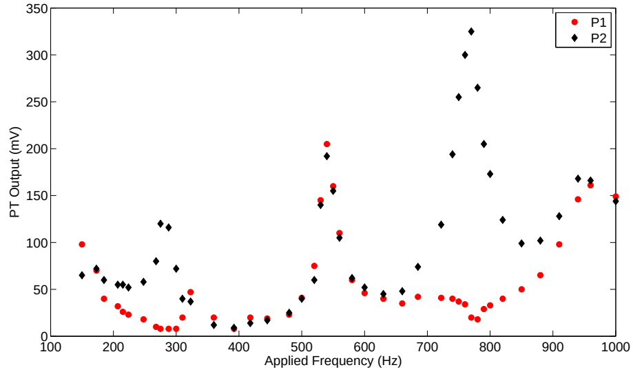
Figure 2.2: Acoustic characterization of the waveguide (S&R configuration) as measured by pressure transducers at P1 and P2. Local maxima for both pressure transducers corresponds to a pressure antinode location. A local minimum at P1 and maximum at P2 corresponds to a pressure node. The distance between the speaker and reflector is approximately 62 cm (Dattarajan, et. al [20])
