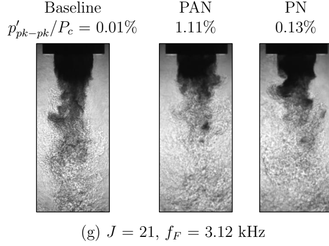
Figure 5.25: Back-lit images of the LAR-thin injector PAN flow at P_r = 1.05 and varying J . The image framing rate was 25 kHz. Table C.4 gives a summary of the acoustic forcing frequencies and amplitudes.
