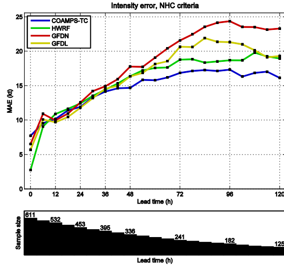
Figure 1. Wind speed mean absolute error (MAE) (knots; 1 \text{ knot} = 0.514 \text{ m s}^{-1} ) as a function of forecast time for the 2010 and 2011 seasons in the Atlantic basin for a homogeneous statistical sample. The numerical models included in this analysis are the Navy's COAMPS-TC, operational models run by NOAA (HWRF, GFDL), and the Navy's current operational limited area model (GFDN). The number of cases is shown at the bottom.
