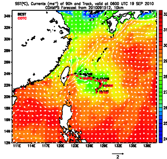
Figure 6. The COAMPS-TC predicted track (red) for Typhoon Fanapi from a 90 h real-time forecast valid at 0600 UTC 19 September 2010 and the observed best track (black). The sea surface temperature ( ^{\circ}\text{C} ) is shown in color shading and indicates significant cooling during the passage of Fanapi. The surface currents are shown by the white vectors.
