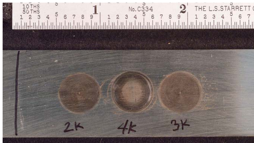
Figure 17. AISI 4340 plate tested for galling with electroactive polymer P3PPA coated buttons with embedded graphite, showing slight galling at a load of 4,000-lbs.
