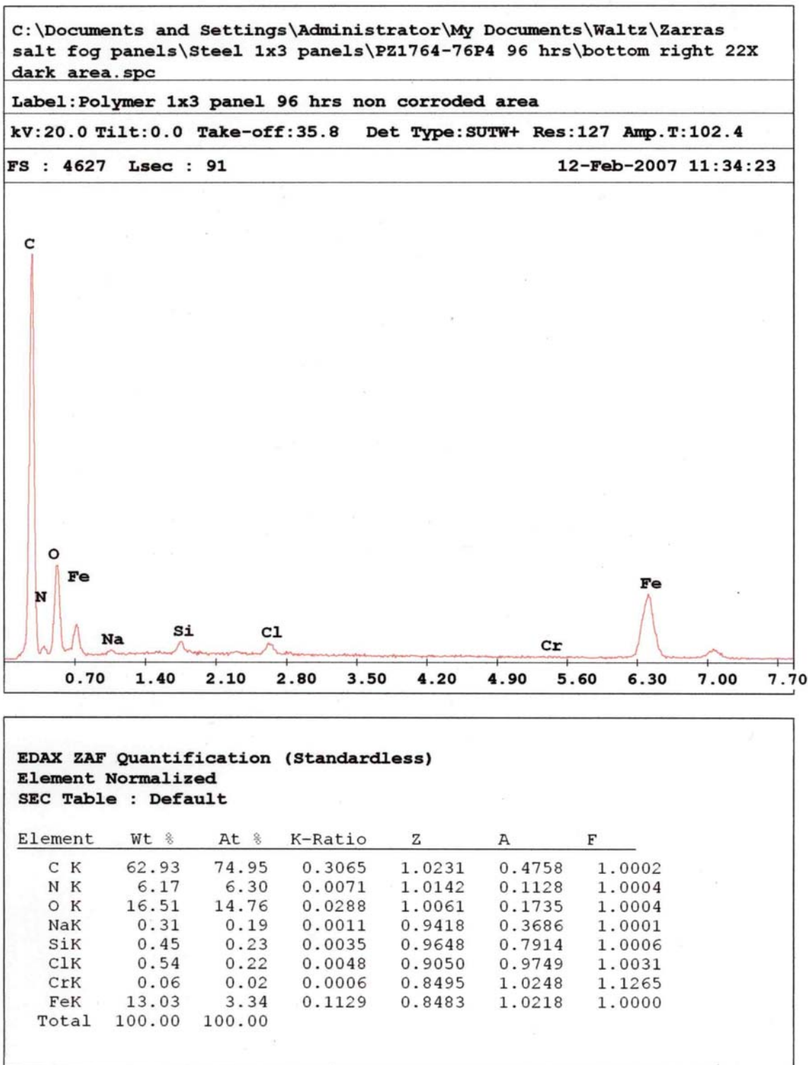
Figure 63: EDS Spectrum of P(7-PHA) Coated Panel After 96 Hours Neutral Salt Fog Exposure.
