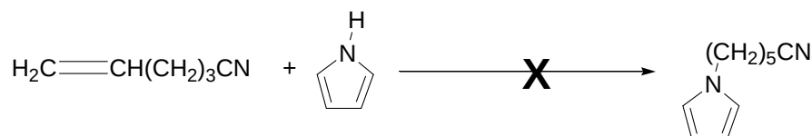
Figure 2: Synthesis of 6-pyrrol-1-yl-hexanitrile
