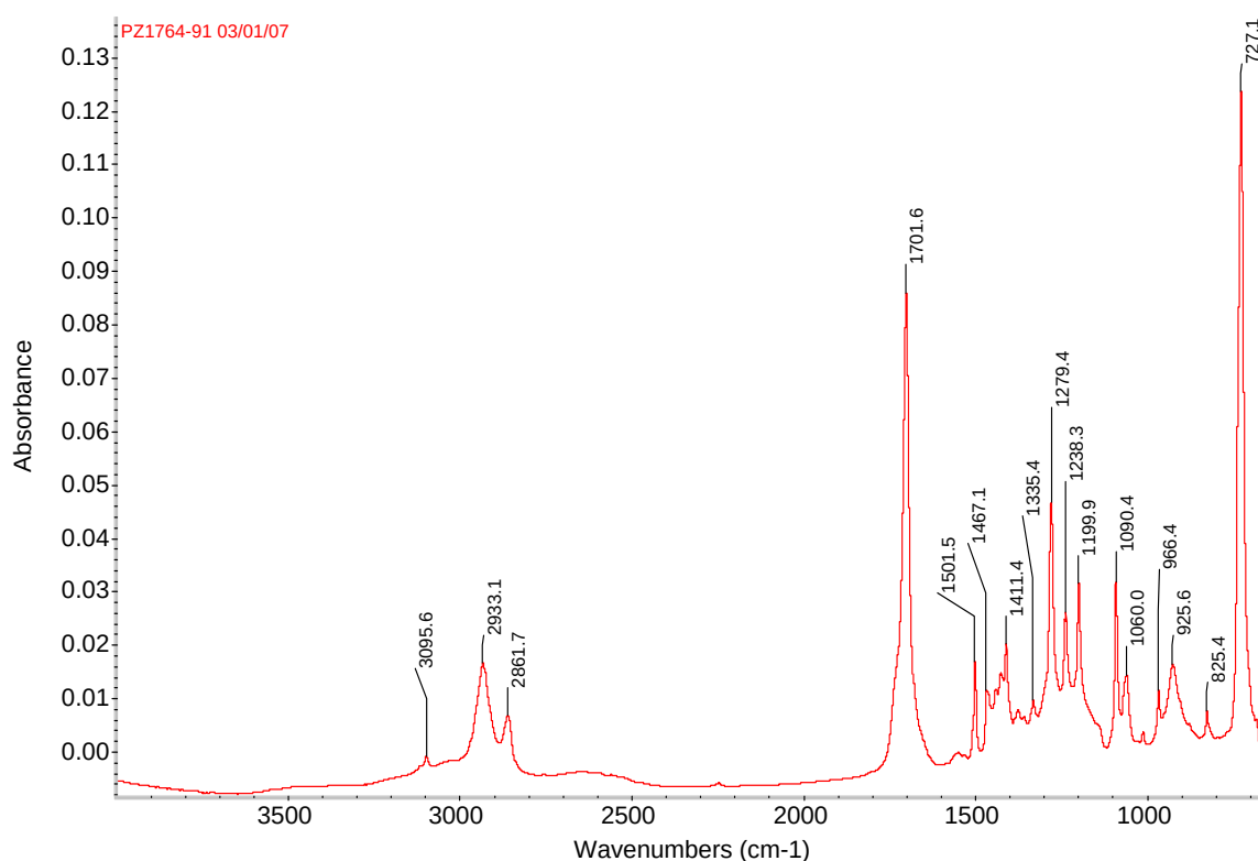
Figure 10: FTIR Spectrum of 7-PHA
