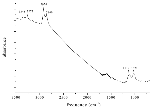
Figure 18: 3-aminopropyl trimethoxysilane on high strength steel button
