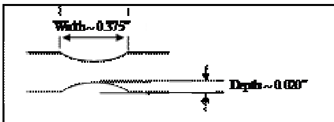
Figure 4-75 Defect Specifications for HS Test Specimens
