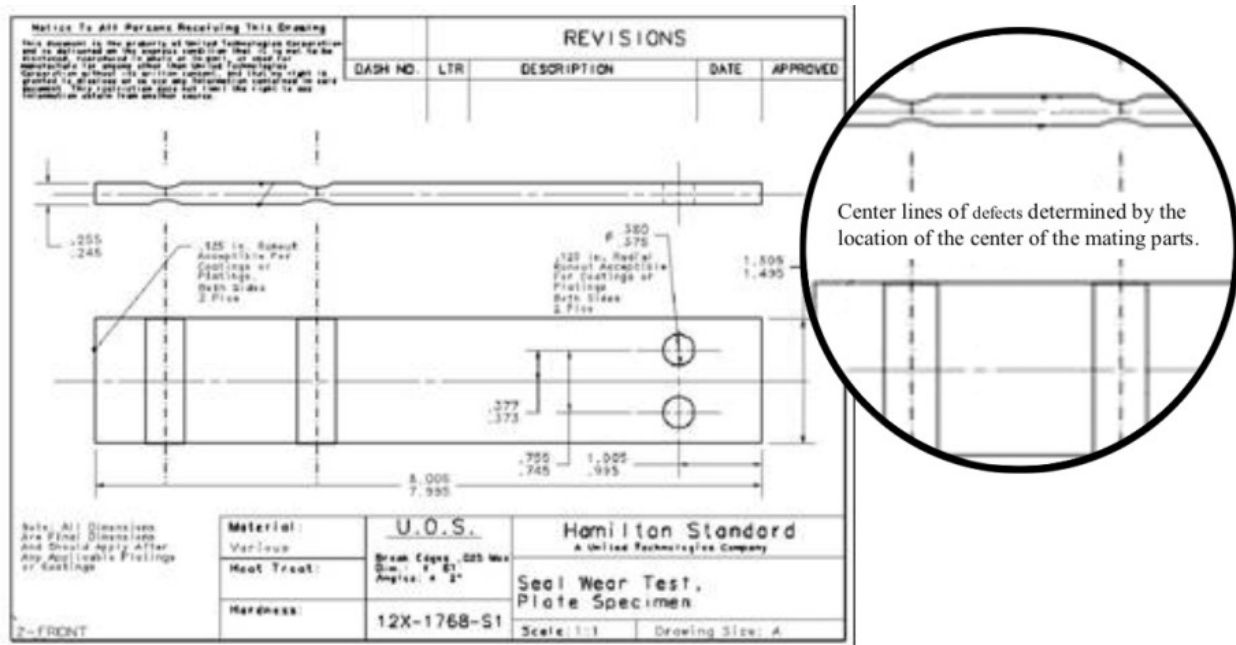
Figure 4-74 Hamilton Sundstrand Wear Specimen – With Defects
