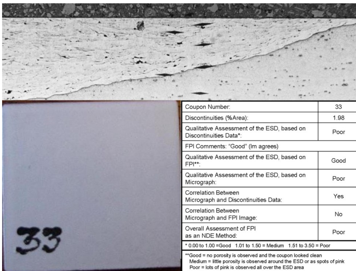
Figure 4-24 Coupon #33. FPI Indicates Good Quality. However, Discontinuities Data and Micrograph Report Poor Quality.
