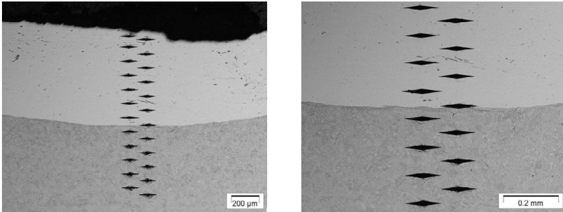
Figure 5-9 Micrographs of Knoop Microhardness Indents Through the ESD Deposit into the Base Metal
