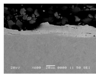
Condition 6 ESD Repair Micrograph.
