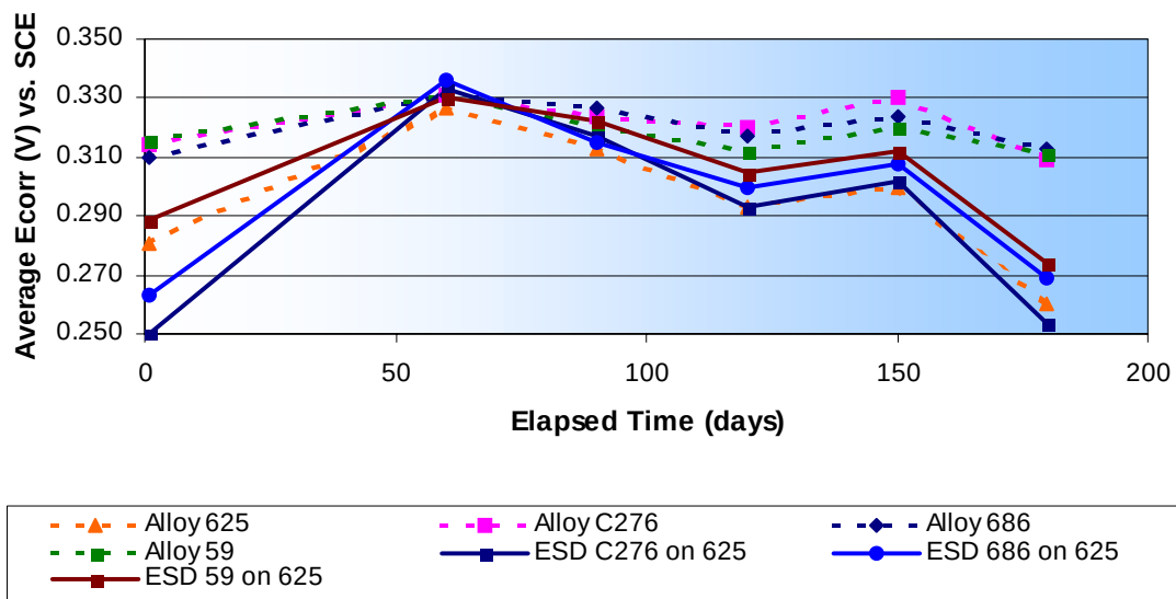
Figure 6-19 Corrosion Potential Versus Time Measurements Made on ESD-Coated and Ni-Cr-Mo Alloy Control Crevice Corrosion Test Specimens
