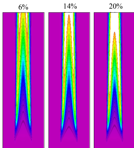
Figure 3.2.8-1. Soot Distribution in a Jet Diffusion Flame with Different Levels of Nitromethane Added to Heptane Fuel Jet. Each image represents 120 mm height. Excess soot is marked in white.
