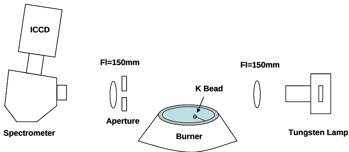
Figure 2.1.3-3. Schematic of Line Reversal Technique. The potassium (K) at 770 nm is seeded in the flame.
