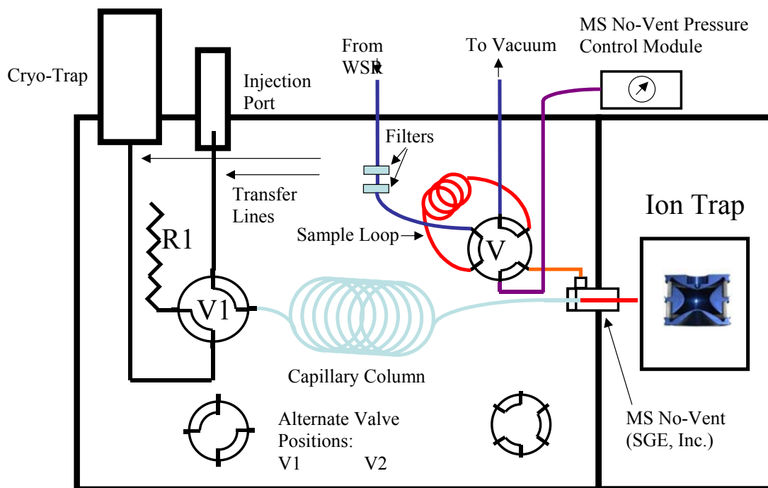
Figure 2.1.2-12. Plumbing Diagram of Saturn GC/MS Configured for Direct Sampling of Gases from WSR.
