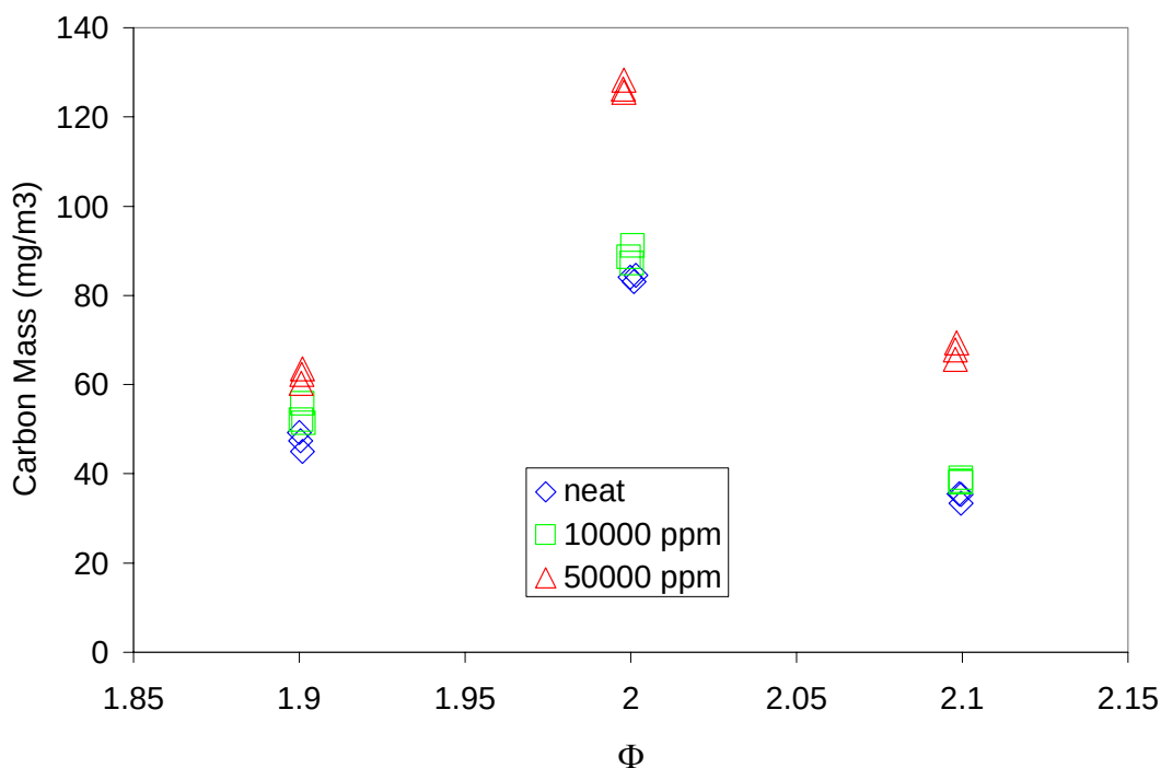
Figure 3.4.3-10. Carbonaceous Carbon Content Measured in the WSR for Quinoline Additive Tests.
