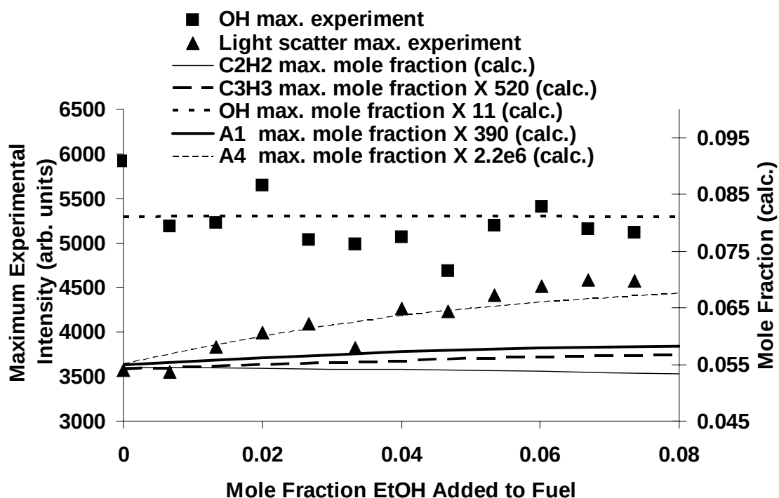
Figure 3.1.6-8. Graph of Experimental Measurements and Predictions Based Upon Calculations for OH, Soot and Soot Precursors, for Fuel Side Addition of Ethanol.
