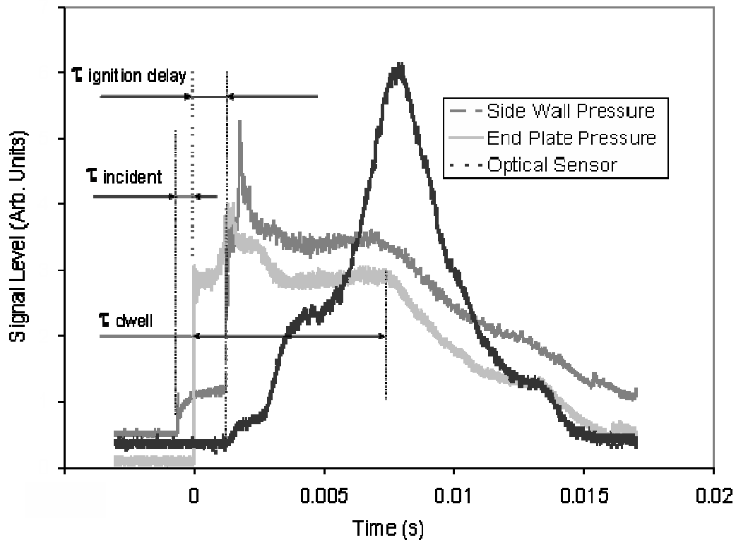
Figure 2.1.1-4. Example Oscilloscope Traces from Combustion of Heptane/Toluene Experiments Showing Pressure Transducers and Optical Sensor Data.
