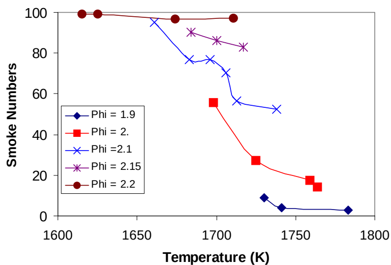
Figure 3.1.3-11. Measured Smoke Number as a Function of the Experimental Temperature.
