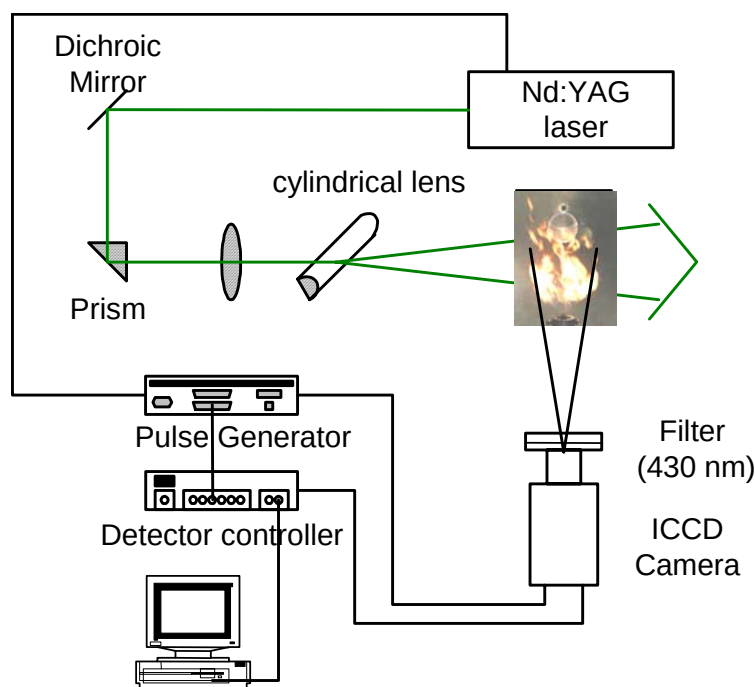
Figure 2.1.7-4. Optical Setup for LII Measurements for Turbulent Spray Flame.
