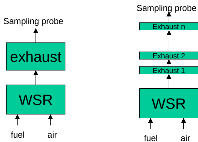
Figure 3.1.3-15. Construction of Reactors to Simulate the Coupled Stirred Reactor and Exhaust.
