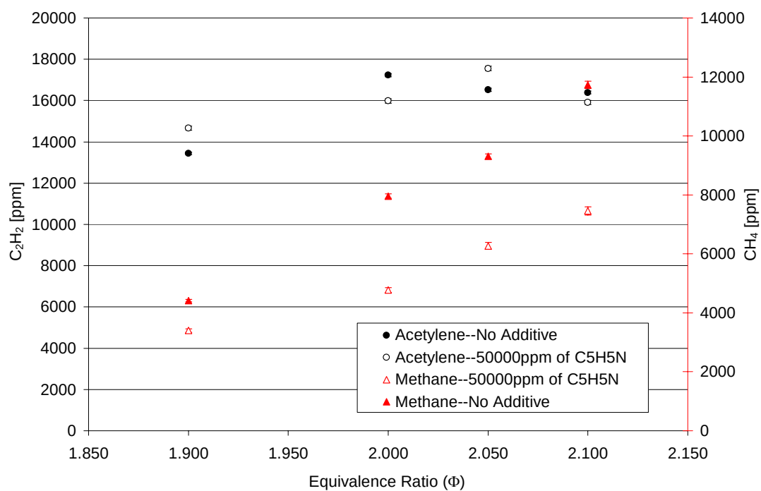
Figure 3.4.3-6. Effect of Pyridine on the Acetylene Concentrations.
