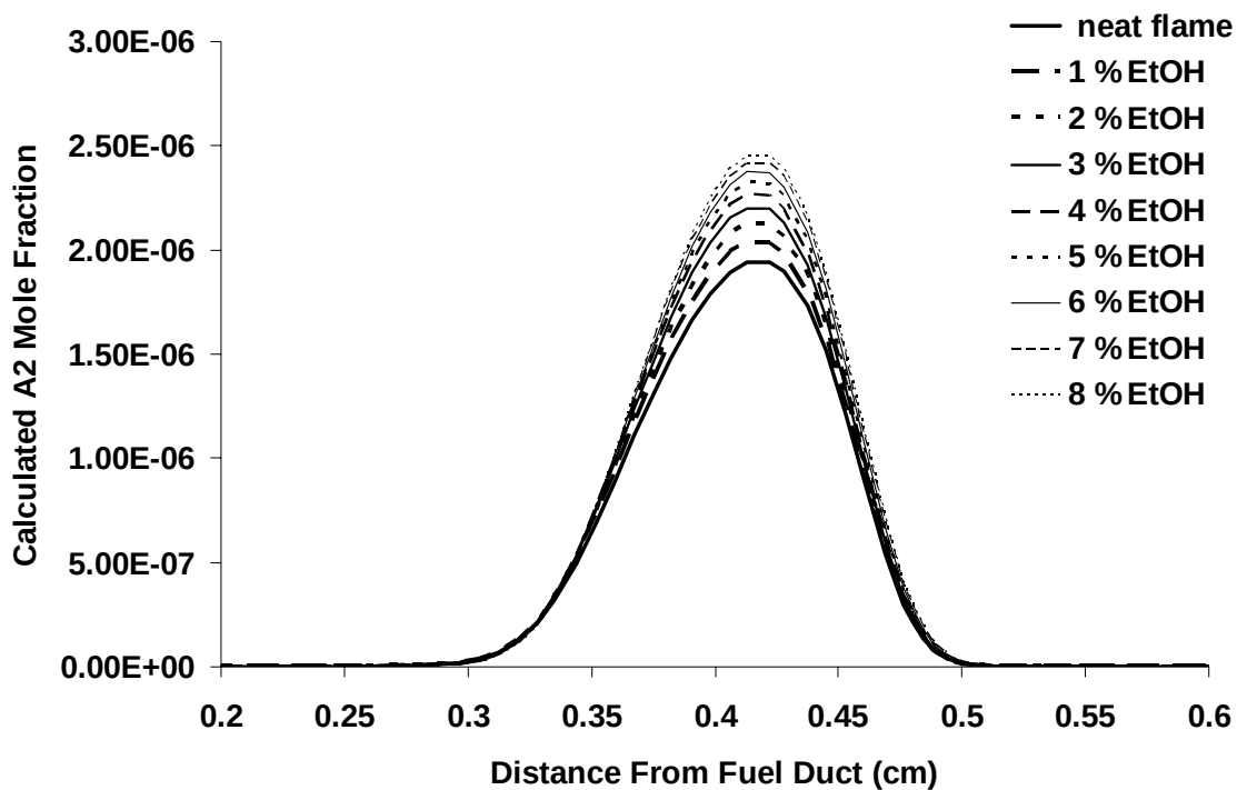
Figure 3.1.6-10. Calculated A2 Mole Fraction Profile for Increasing Amounts of Ethanol Vapor Added to the Fuel Stream.
