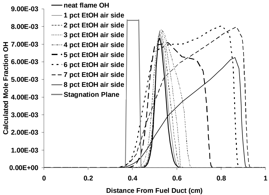
Figure 3.1.6-6. Calculated OH Profiles for Air Side Addition of Ethanol. Also shown is estimated position of stagnation plane.
