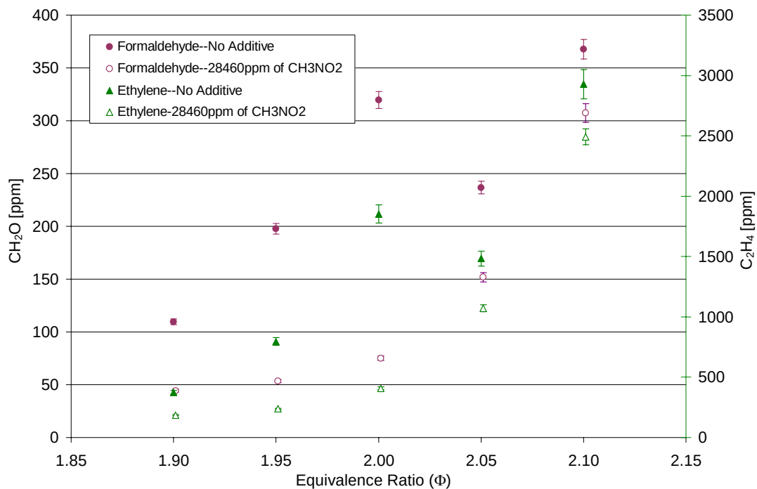
Figure 3.2.3-4. Effect of Nitromethane on Formaldehyde and Ethylene Emissions from the WSR.
