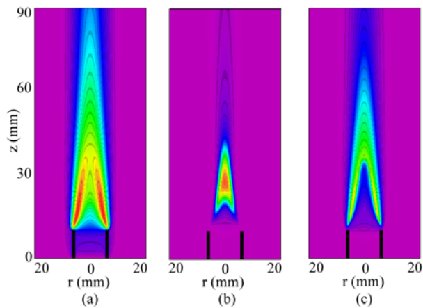
Figure 3.5.8-4. Heptane Jet Diffusion Flame. Distributions of (a) temperature, (b) soot volume fraction and (c) NO concentration.
