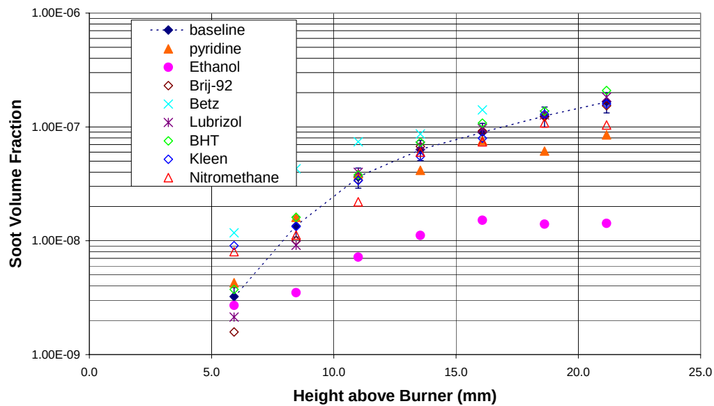
Figure 3.1.4-3. Soot Volume Fractions from Premixed, Laminar Flames. Base flame is 10% toluene and 90% heptane.
