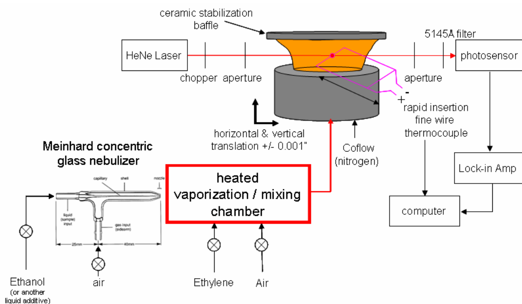
Figure 2.1.4-6. Experimental Setup for the Ethanol/Ethylene Flame Experiments.
