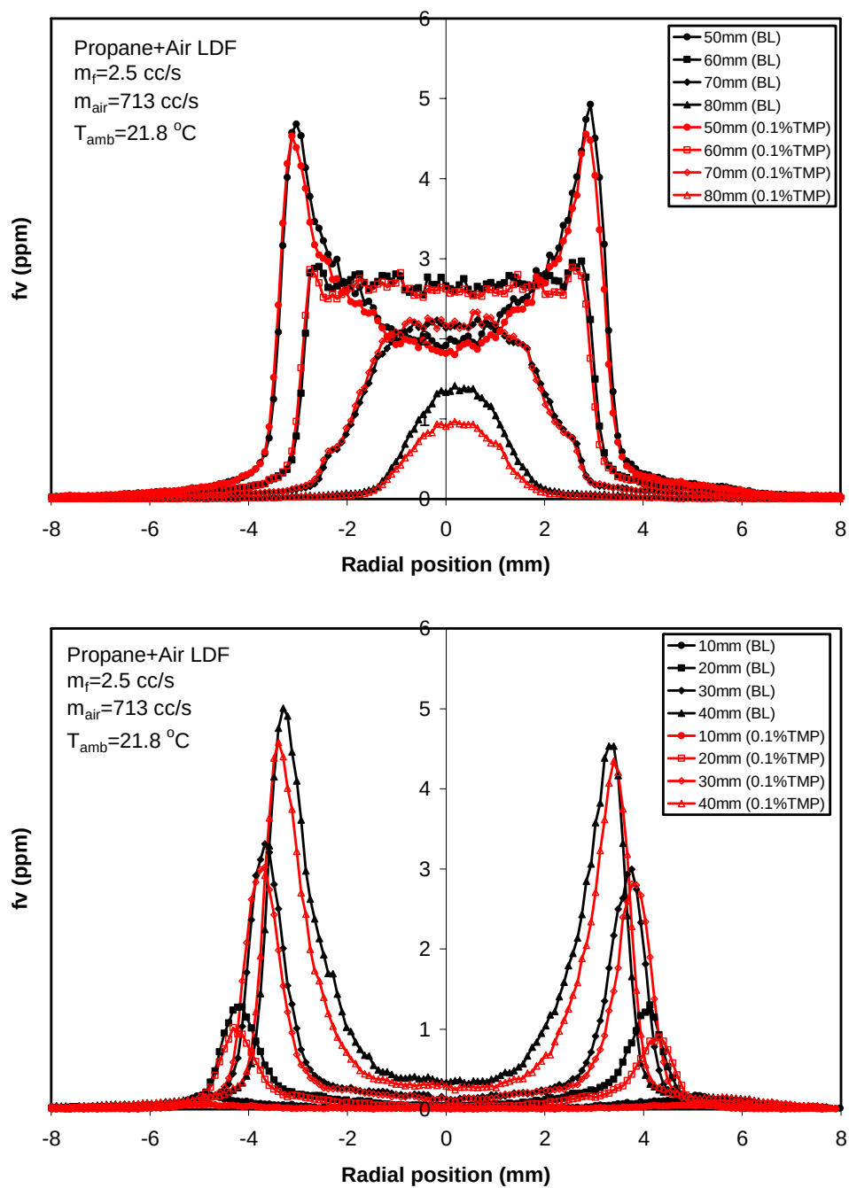
Figure 3.5.5-3. Soot Volume Fraction Profiles for Propane Flame with Baseline and TMP Addition.
