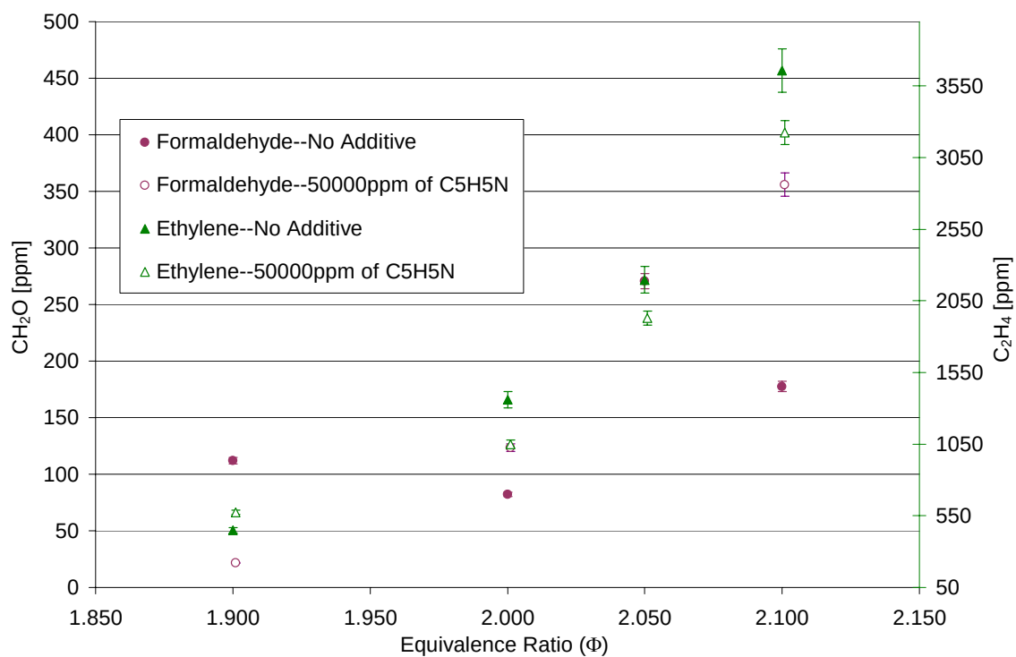
Figure 3.4.3-7. Effect of Pyridine on Formaldehyde and Ethylene Concentrations.
