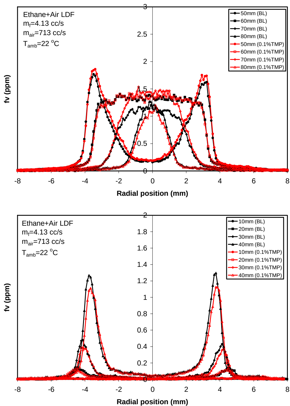
Figure 3.5.5-4. Soot Volume Fraction Profiles for Ethane Flame with Baseline and TMP Addition.
