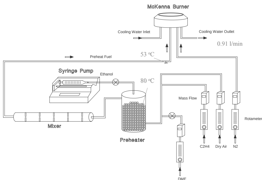
Figure 2.1.3-1. Schematic of Fuel, Additive, and Air Delivery Systems for Premixed Flame Experiments at Penn State.
