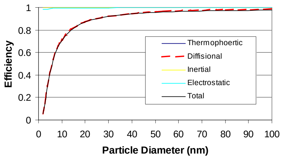
Figure 3.1.3-14. Computed Penetration Efficiencies of Particles through Sampling Lines.
