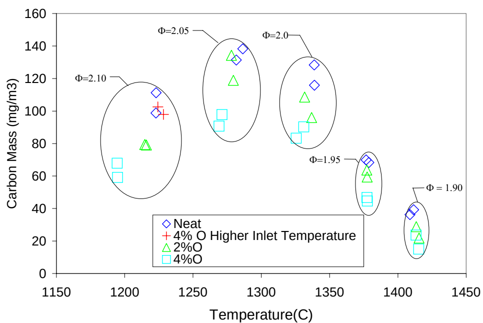
Figure 3.1.3-18. Total Carbon Mass for Cyclohexanone Additive.
