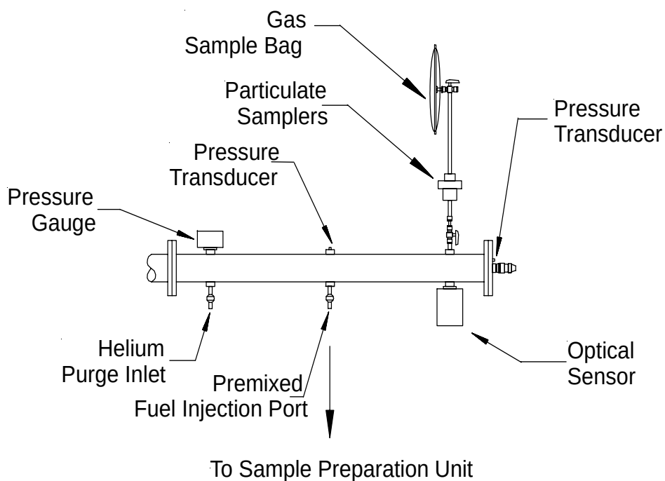
Figure 2.1.1-2. Shock Tube Test Section Configured for Homogeneous Combustion Particulate Sampling and Gas/Liquid Phase Fuel Injection.
