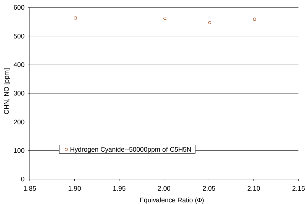
Figure 3.4.3-8. Hydrogen Cyanide Concentration with Pyridine as an Additive (neat concentrations were below detectable limits).
