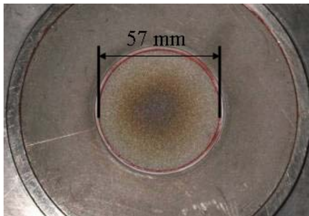
Figure 2.1.4-4. Photograph of the Porous Plug Burner Used from 2002 to September 2005.
