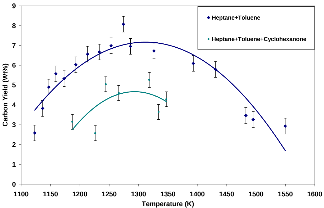
Figure 3.1.2-2. The Effect of Cyclohexanone on Soot Yield.
