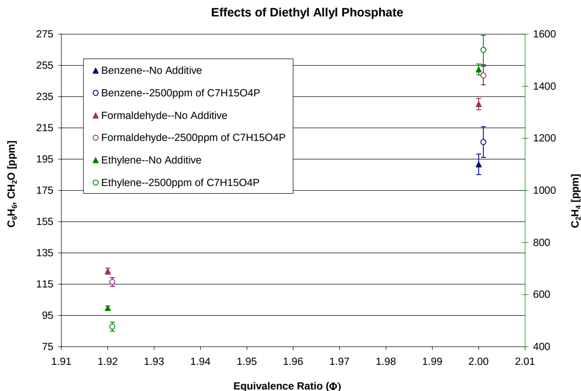
Figure 3.5.3-5. Gas Analysis of Light Hydrocarbons from WSR.
