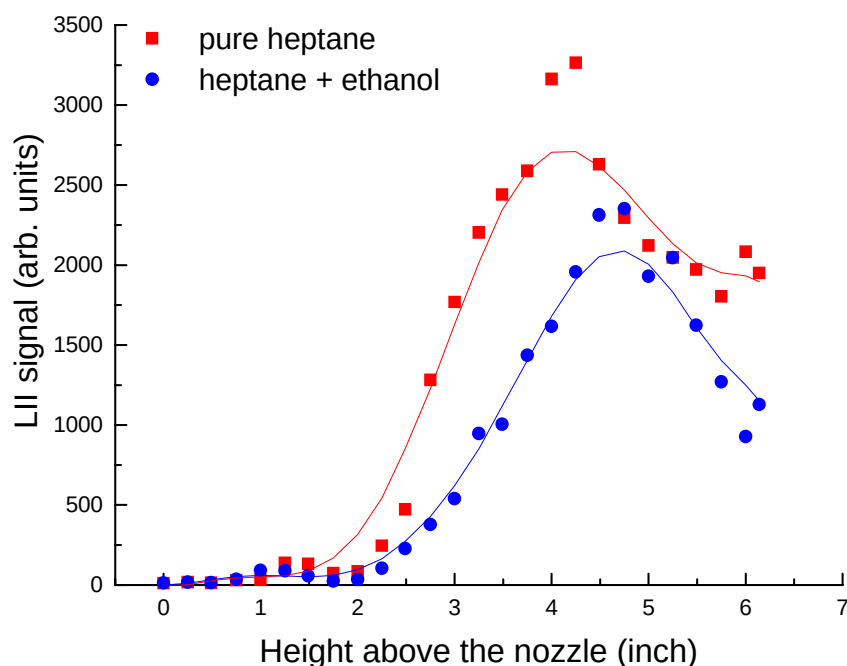
Figure 3.1.7-5. Effects of Ethanol Addition on Soot.
