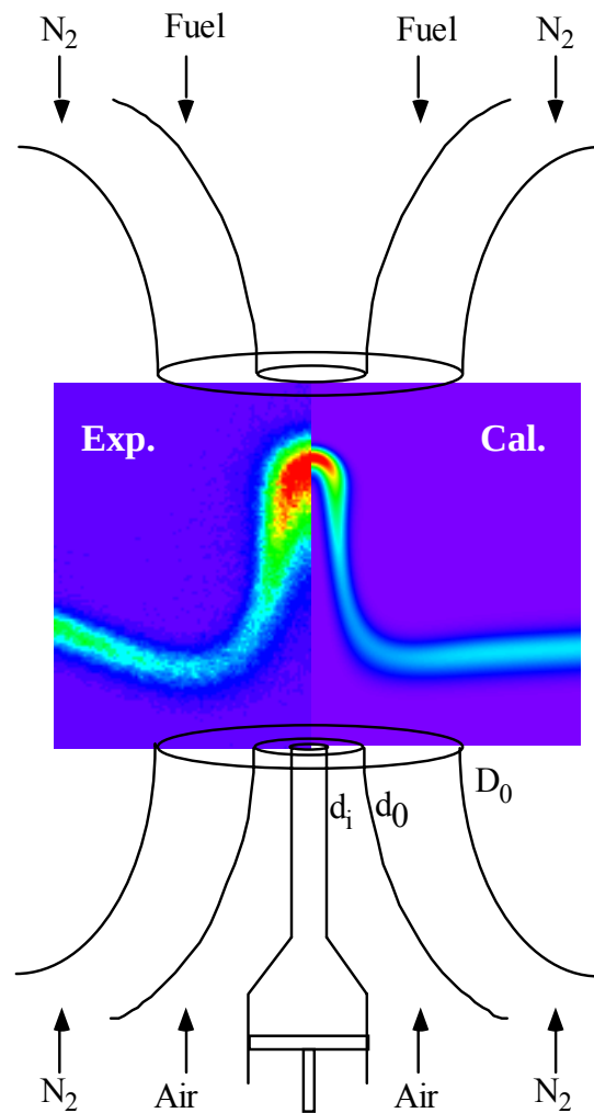
Figure 2.2.3-2. Schematic Diagram of Opposing-Jet Burner Used in the Studies of Vortex-Flame Interactions. Inserted images (measured and computed on the left and right halves, respectively) are that of a typical protruded flame obtained with a micro airside vortex showing an increase in the concentration of OH at the tip.
