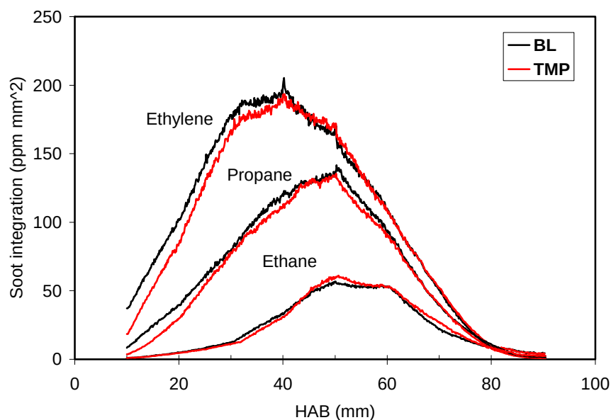
Figure 3.5.5-5. Integrated Soot Volume Fraction as a Height of the Flame
