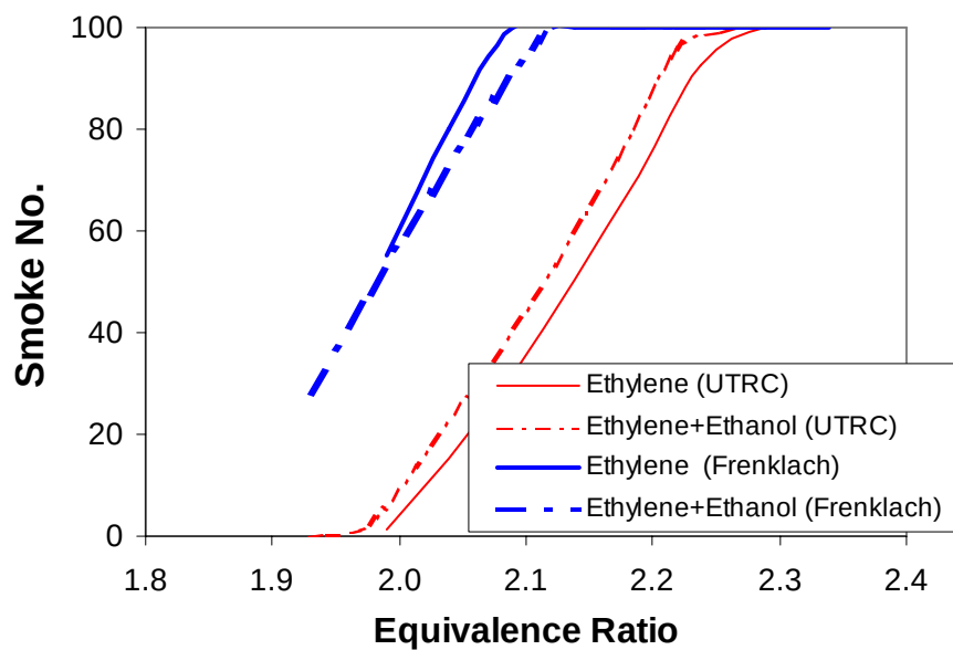
Figure 3.1.3-9. Predicted Smoke Numbers in PSR Using Two Kinetic Mechanisms for Ethylene and Ethylene with Ethanol Additive.
