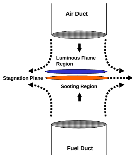
Figure 2.1.5-1. A Schematic of an Opposed Flow Burner with Flame.
