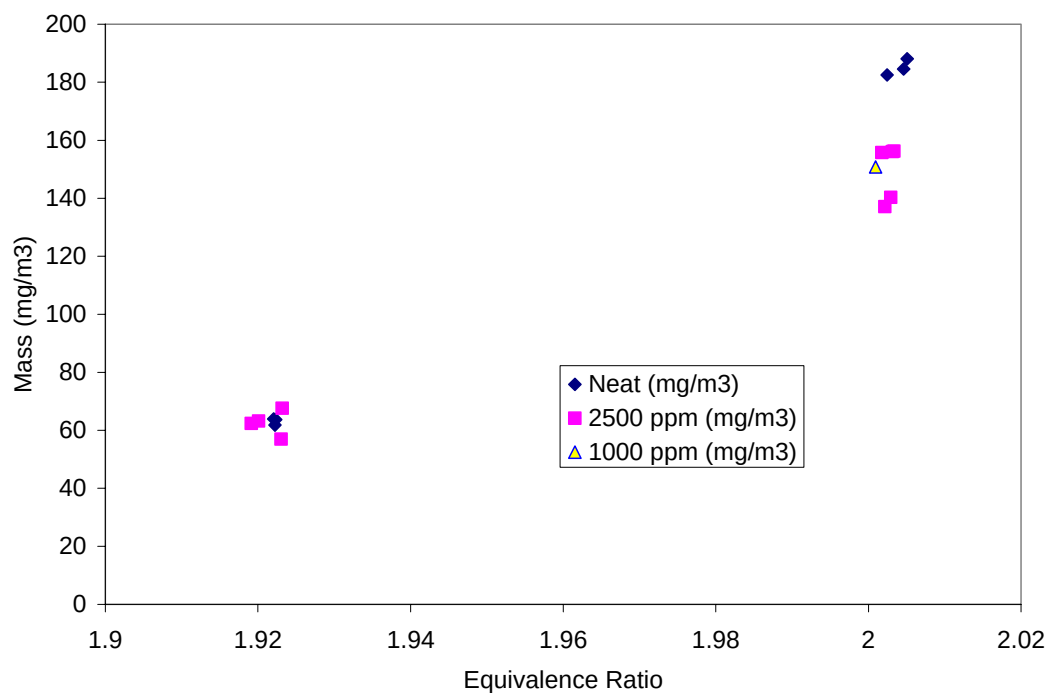
Figure 3.5.3-1. The Effect of Diethyl Allyl Phosphate on Measured Carbon Mass from Samples in the WSR.
