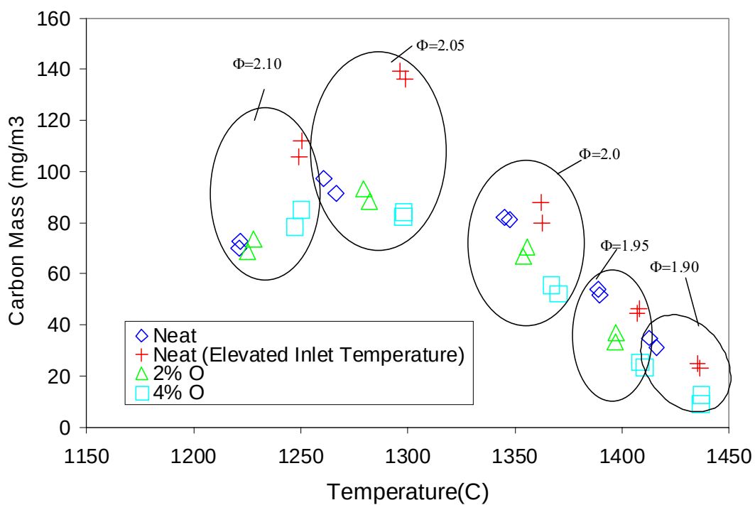
Figure 3.2.3-7. Carbonaceous Carbon Mass for the Nitroethane Additive Cases Studied in the WSR.
