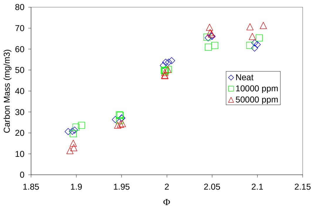
Figure 3.4.3-3. Volatile Carbon Mass for Pyridine in the WSR.
