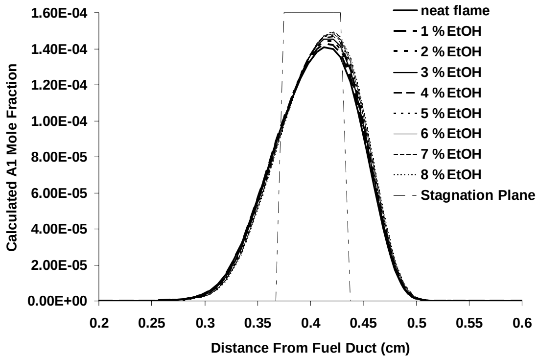
Figure 3.1.6-9. Calculated A1 Mole Fraction Profile for Increasing Amounts of Ethanol Vapor Added to the Fuel Stream.
