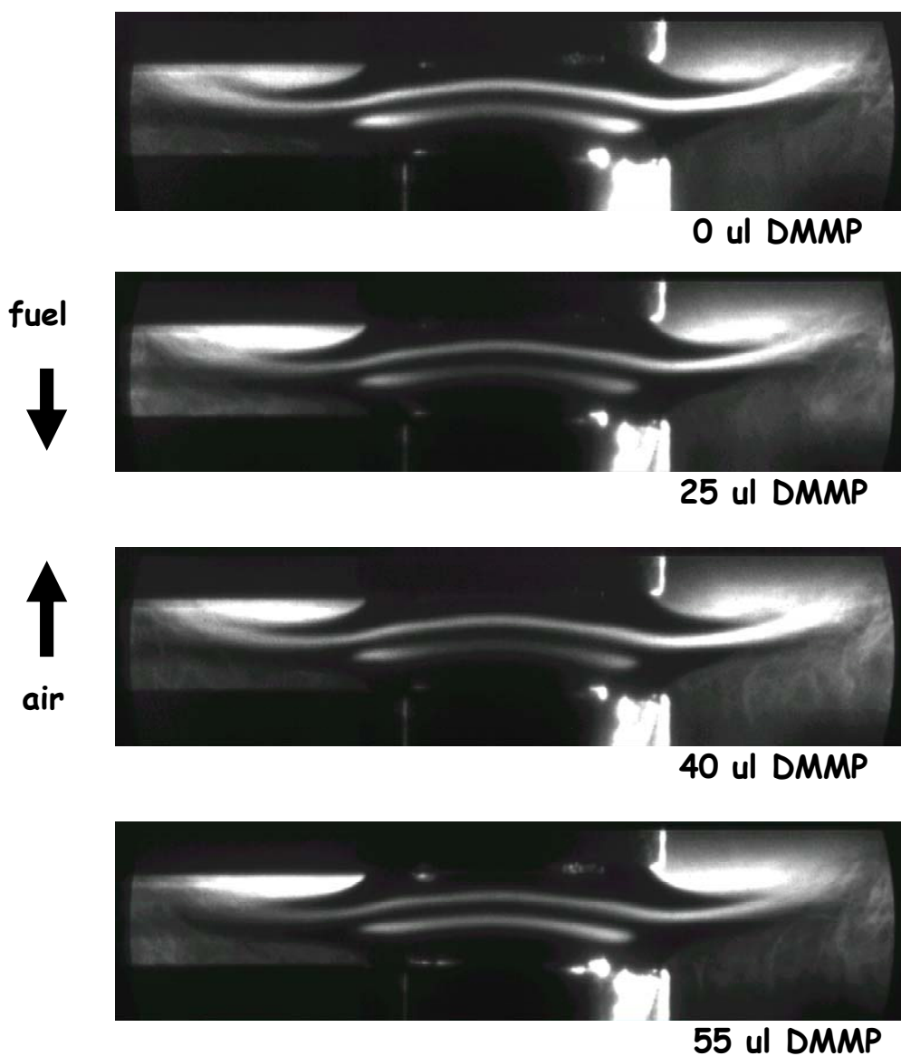
Figure 3.5.6-4. PLIF Images of Opposed Flow Ethylene/Air Flames to which DMMP has been Added to the Fuel (ethylene) Stream. Note the fuel stream enters the flame from above.
