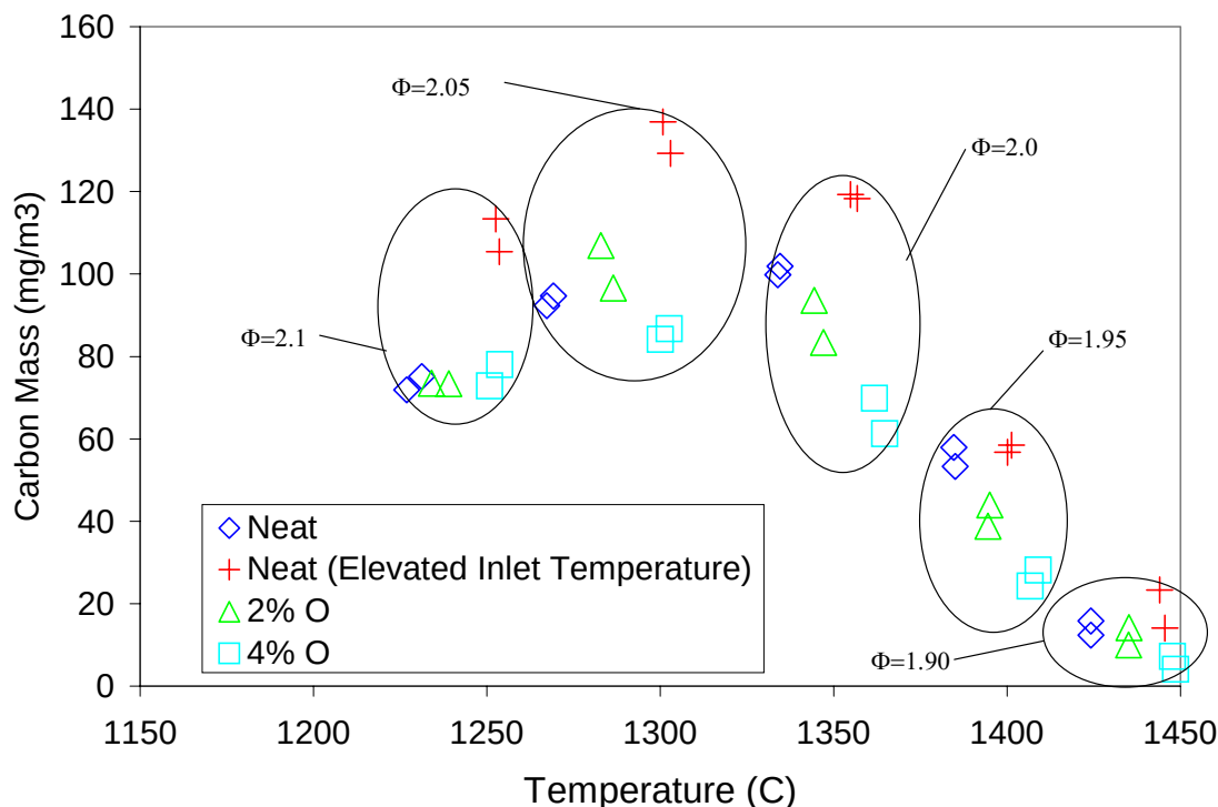
Figure 3.2.3-9. Carbonaceous Carbon Mass for the Nitroethane Additive Cases Studied in the WSR.
