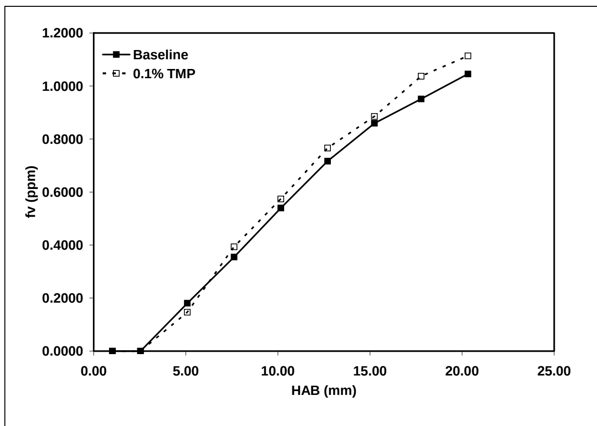
Figure 3.5.4-2. Effect of TMP on Soot Volume Fractions for \Phi = 2.64 Premixed C_2H_4 Flame.
