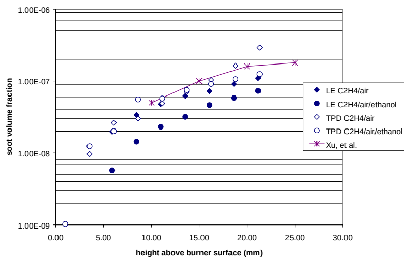
Figure 3.1.4-2. Soot Volume Fraction via Laser Extinction (LE) and Thermocouple Particle Densitometry (TPD) for Flame 1 and 2.
