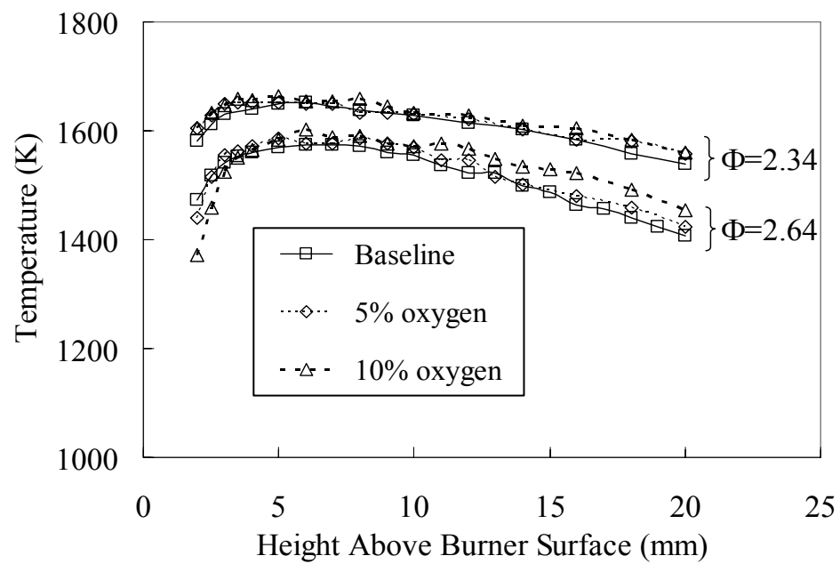
Figure 3.1.5-5. Measured Flame Temperature Profiles for \Phi = 2.34 and 2.64.
