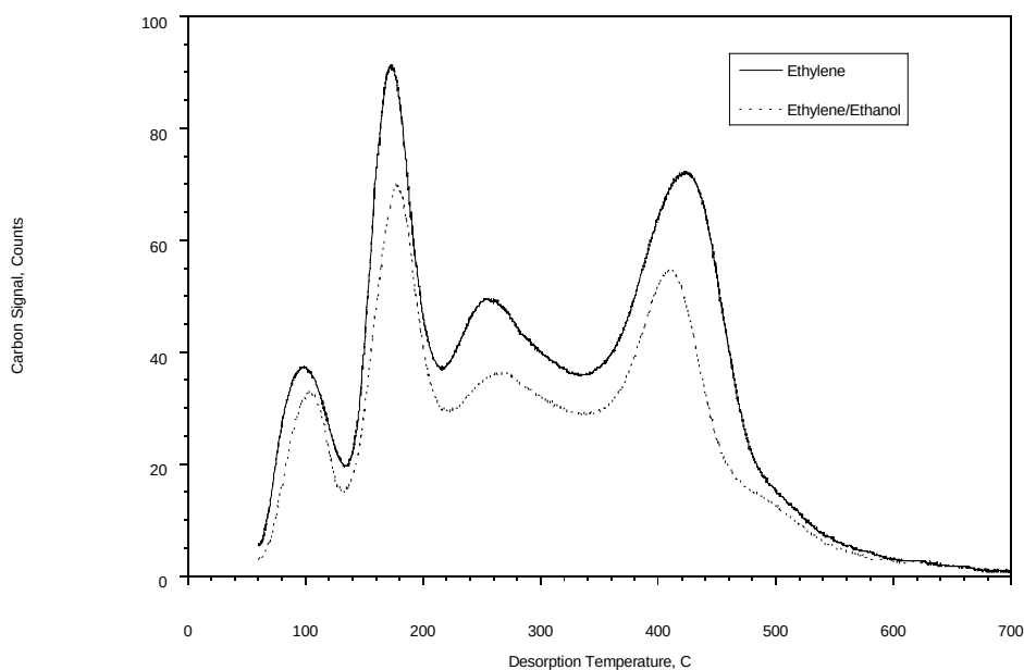
Figure 3.1.2-1. Averaged Carbon Signal Obtained by Desorbing Soot Samples Collected from Ethylene and Ethylene+Ethanol Experiments Listed in Table.
