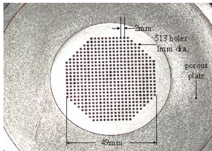
Figure 2.1.4-1. Photograph of the Burner Surface.
