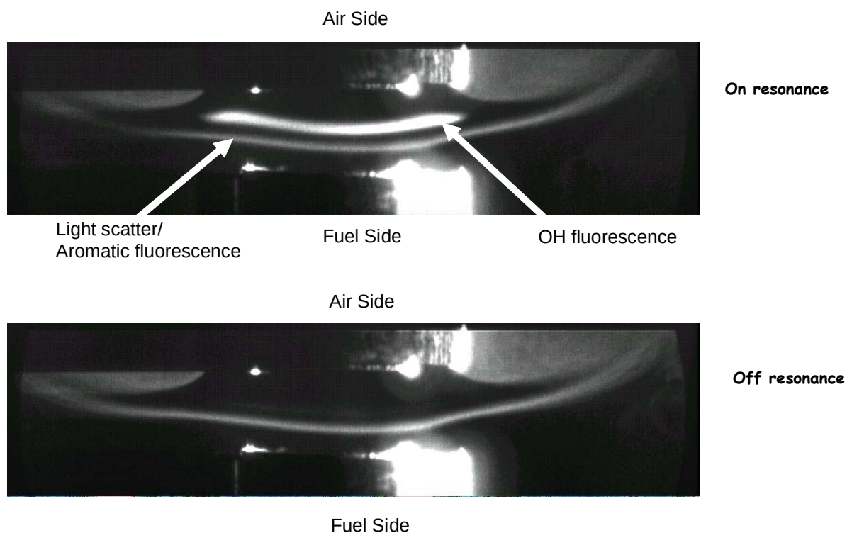
Figure 2.1.5-6. On and Off Resonance Images Showing the Sooting and OH Regions in an Opposed Flow Ethylene/Air Flame.
