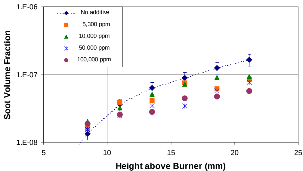
Figure 3.4.4-1. Reduction of Soot in Premixed Flame with Various Levels of Added Pyridine (as ppm in fuel).
