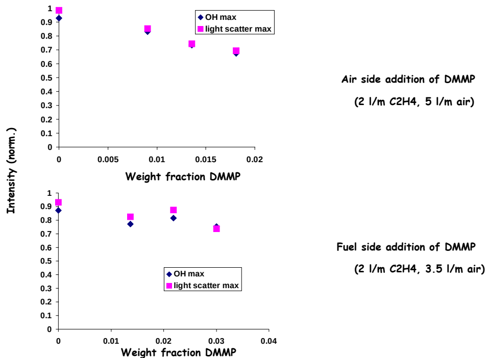
Figure 3.5.6-5. A Summary of Experimental Measurements of DMMP to Fuel and Oxidizer Streams for the Opposed Flow Ethylene/Air Flames.
