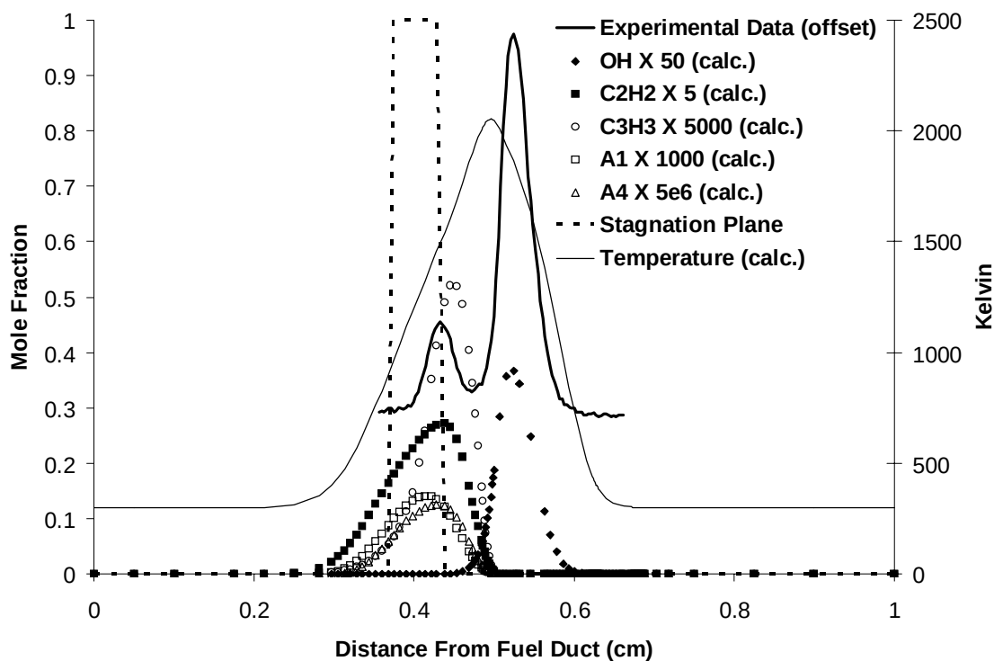
Figure 3.1.6-1. Results of Calculations Showing Temperature Profile and Separation of Soot Forming and Flame Radical Regions for an Undoped Ethylene/Air Opposed Flow Flame, with Overlay of Measured Centerline Pixel Intensities for Similar Flame. Also shown is calculated position of stagnation plane.
