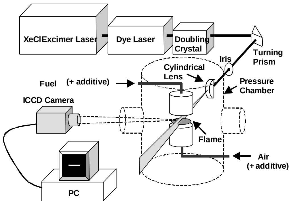
Figure 2.1.5-2. A Schematic of the Experimental Apparatus, Including Optics.
