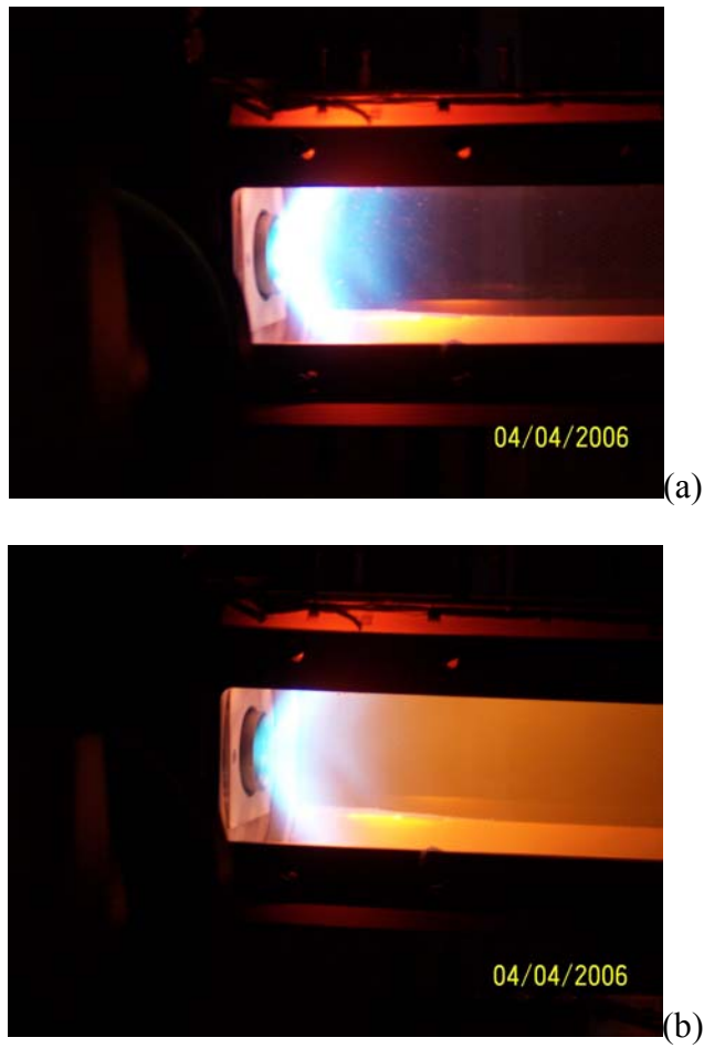
Figure 3.5.7-3. Photographs of Combustor Burning Heptane/Toluene at \Phi=0.7 : (top) no additive, (bottom) 1000 ppm.
