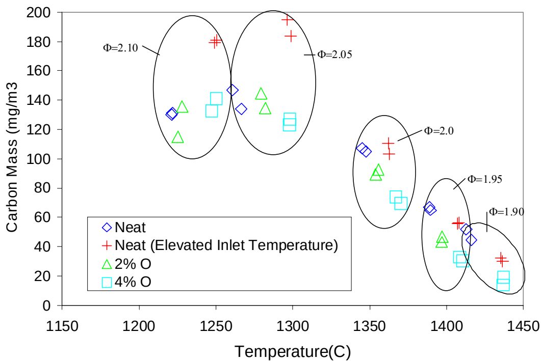
Figure 3.2.3-6. Total Carbon Mass for Nitroethane Additive Cases Studied in the WSR.
