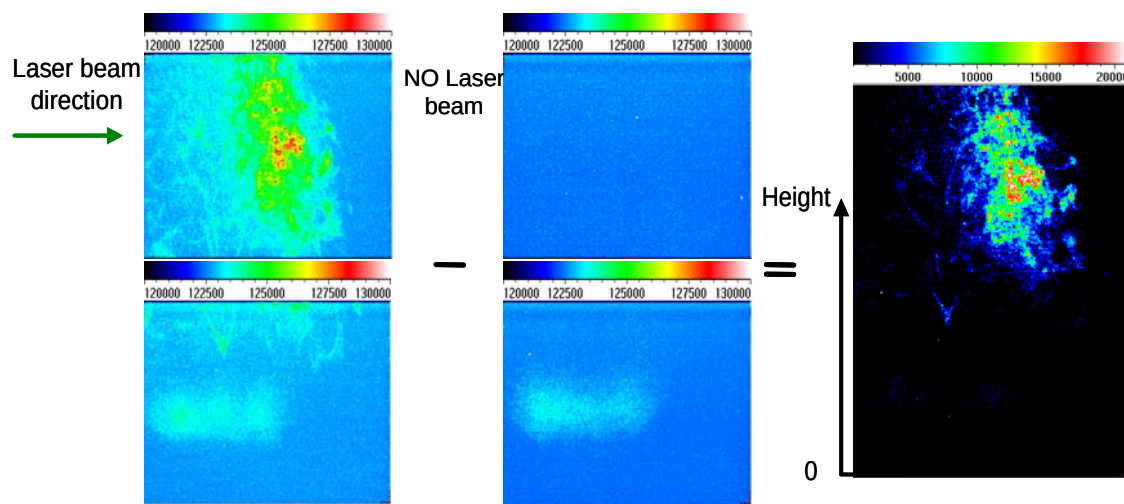
Figure 3.1.7-3. Comparison of LII images Before and After Background Correction.
