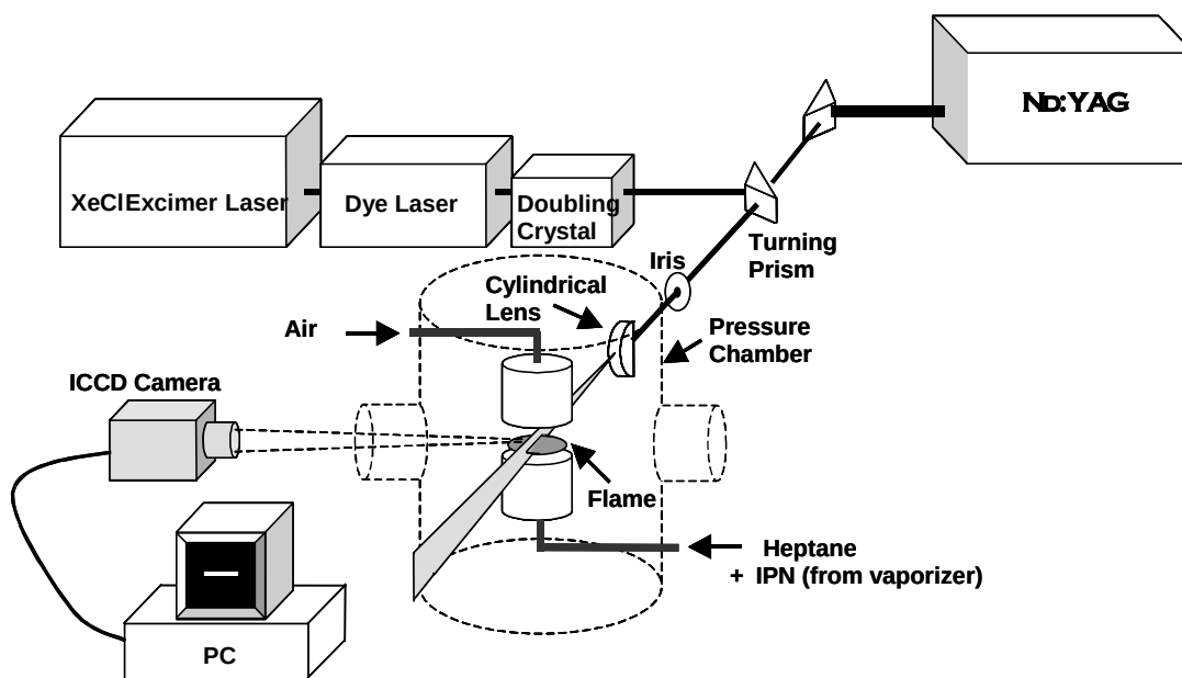
Figure 2.1.5-7. A Schematic of the Experimental Apparatus Used for Measuring PLII and PLIF.
