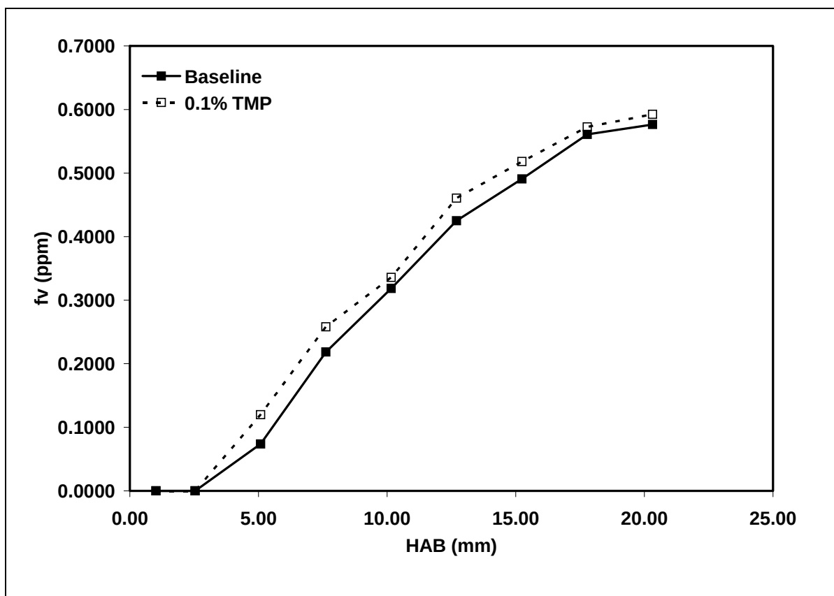
Figure 3.5.4-1. Effect of TMP on Soot Volume Fractions for Phi = 2.34 Premixed C 2 H 4 Flame.
