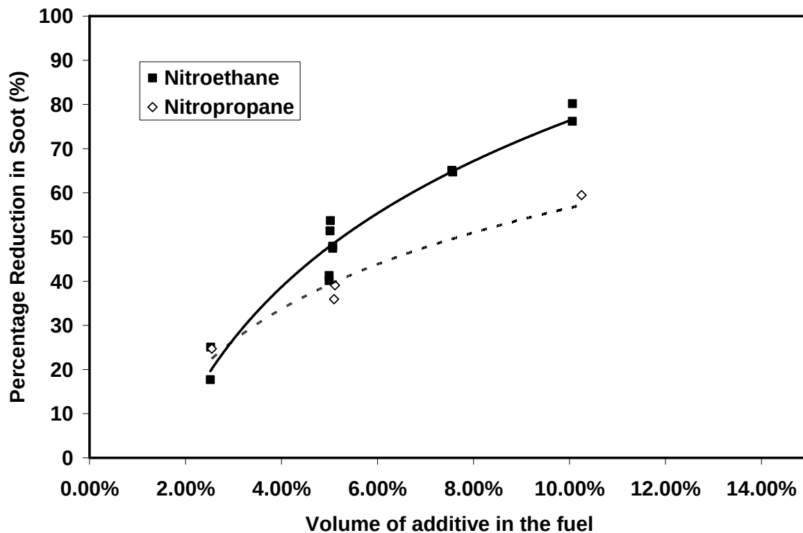
Figure 3.2.7-1. Effect of Nitroalkanes on Soot Formation in the Dump Combustor with JP-8.
