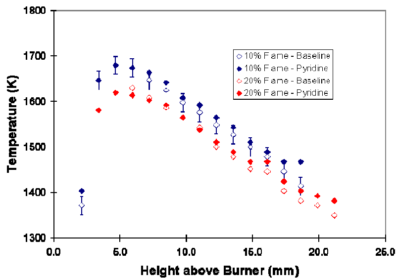
Figure 3.4.4-2. Measured Temperature Profiles for Several Premixed Flames.
