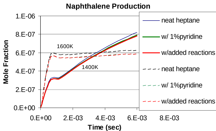
Figure 3.4.4-4. Comparison of Predicted Naphthalene With and Without Added Pyridine.
