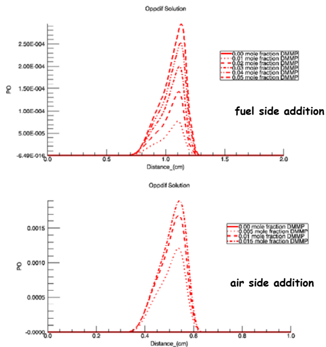
Figure 3.5.6-11. Calculated PO Concentration vs Flame Position (centerline) for Fuel and Oxidizer Side Addition to Ethylene/Air Opposed Flow Flames.
