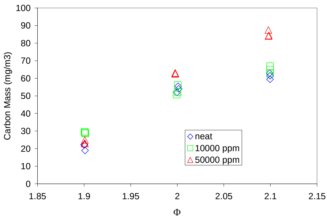
Figure 3.4.3-9. Volatile Carbon Mass for Quinoline Additive Tests in the WSR.
