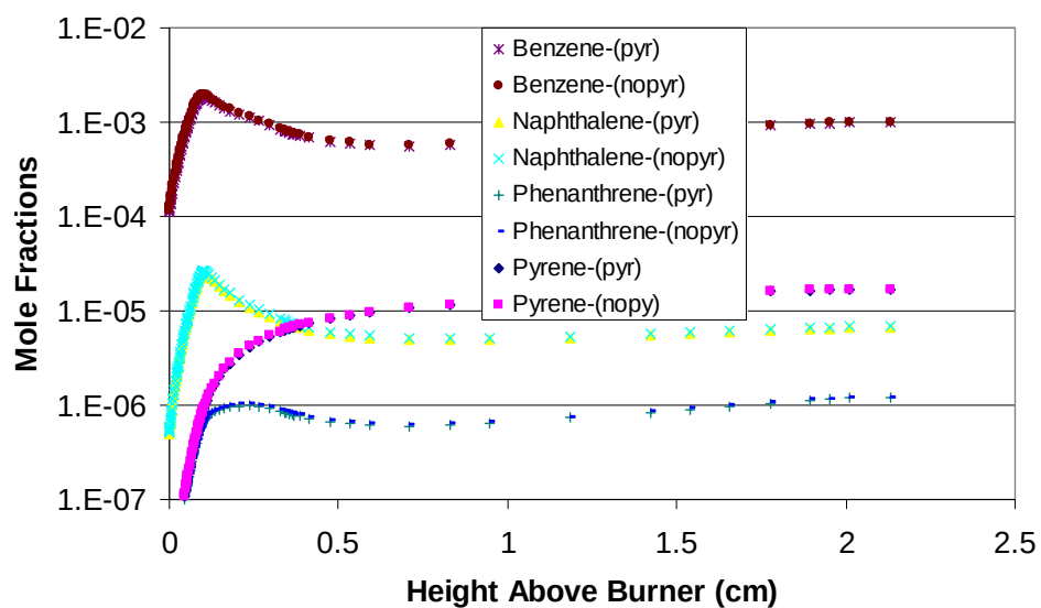
Figure 3.4.4-5. Comparison of Computed Mole Fractions for Several Species as a Function of Height Above the Burner for Fuel-Rich, Premixed Flames With and Without Added Pyridine.
