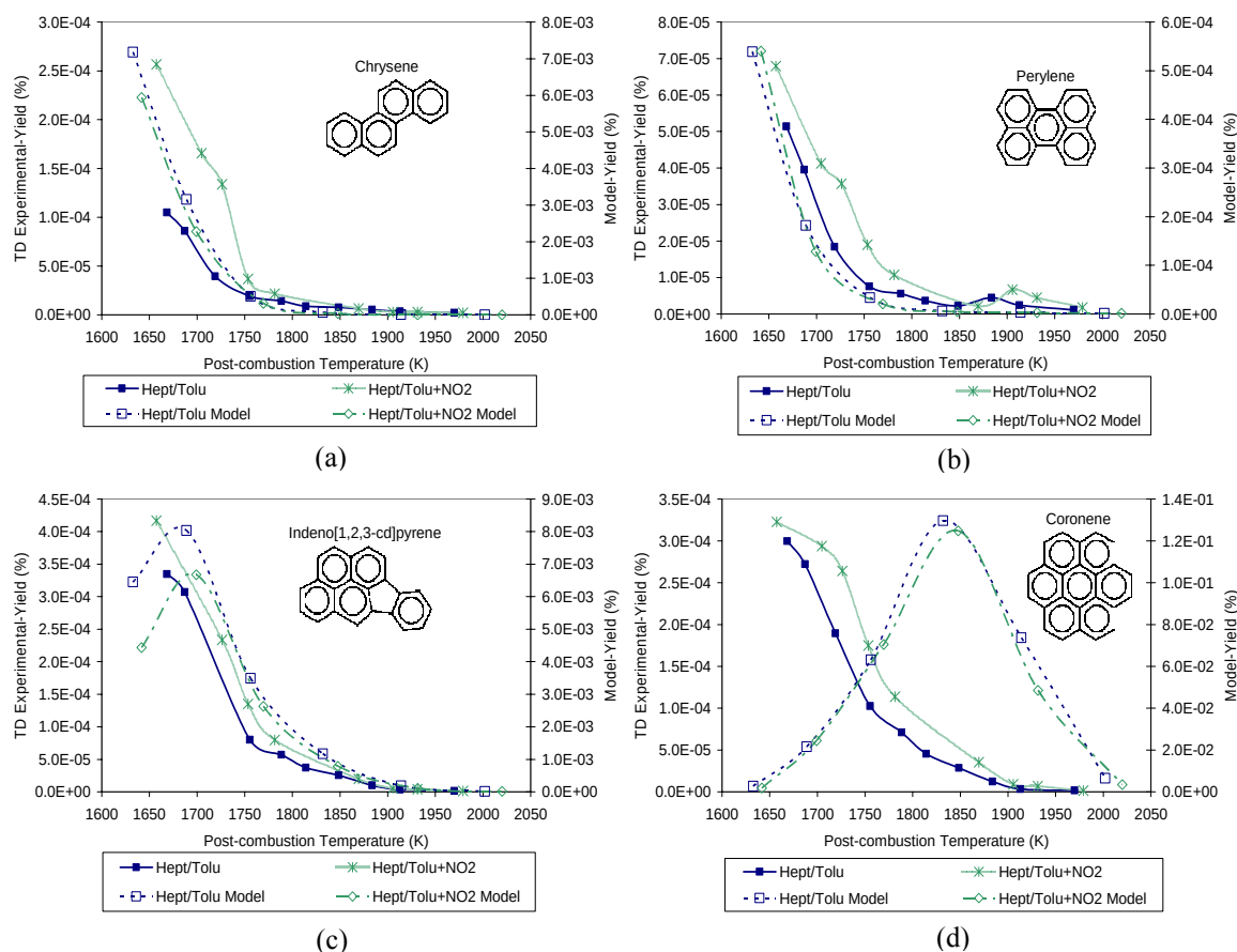
Figure 3.3.2-3. Yields of (a) Chrysene, (b) Perylene, (c) Indeno[1,2,3-cd]Pyrene, and (d) Coronene from Combustion of n-Heptane/Toluene and n-Heptane/Toluene + NO 2 at 21 atm.
