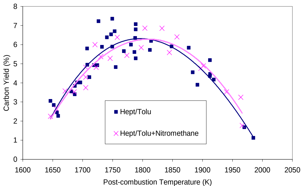
Figure 3.2.2-1. Carbon Yield from Combustion ( \Phi = 3 ) of n-Heptane/Toluene and n-Heptane/Toluene + Nitromethane at 21 atm.
