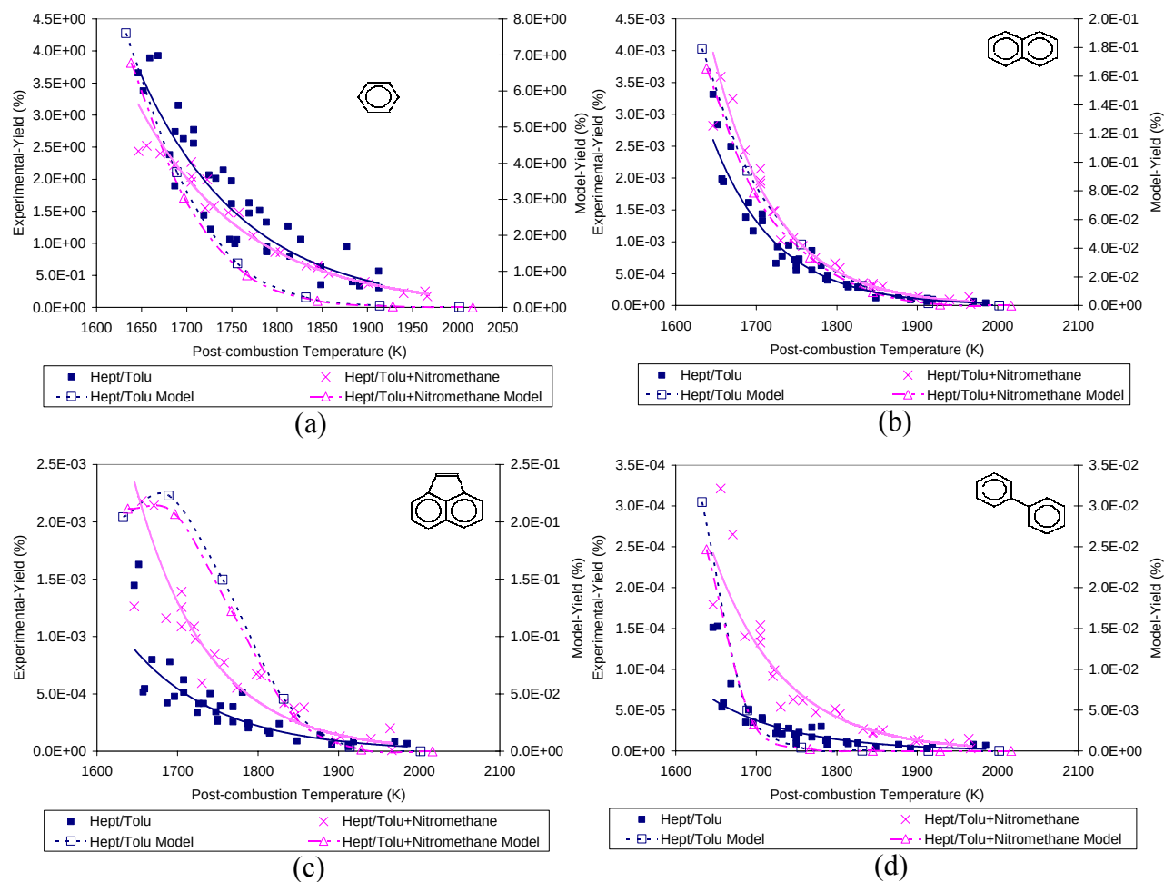
Figure 3.2.2-2. Yields of (a) Benzene, (b) Naphthalene, (c) Acenaphthylene, and (d) Biphenyl from Combustion of n-Heptane/Toluene and n-Heptane/Toluene + Nitromethane at 21 atm.
