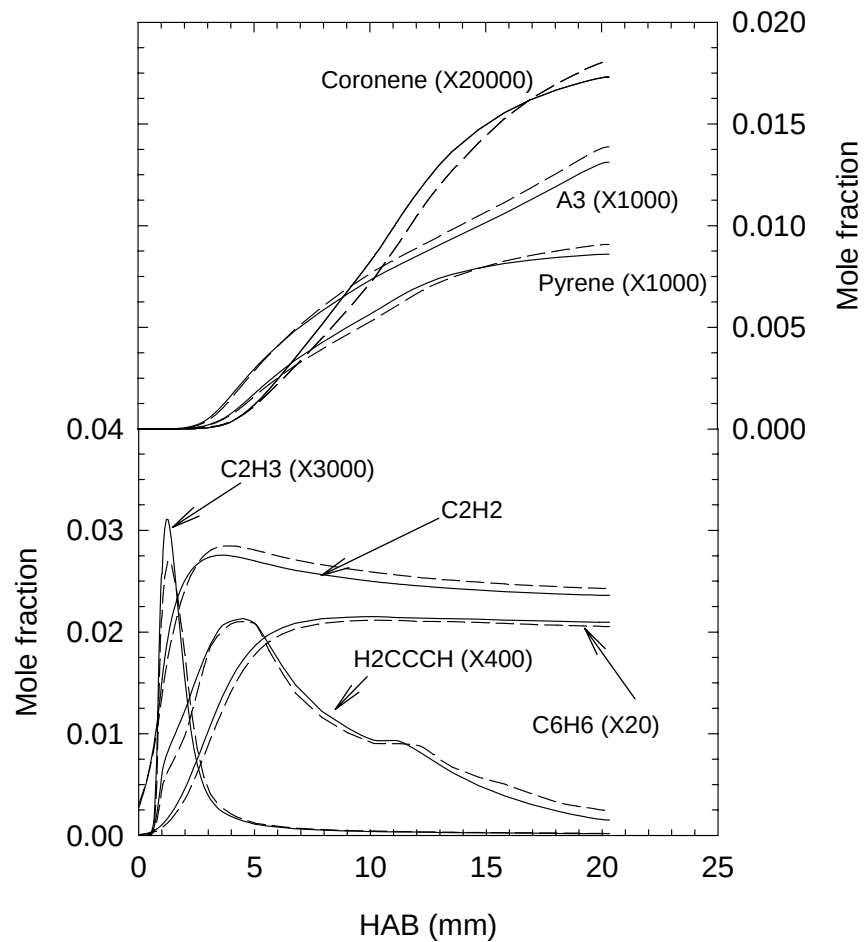
Figure 3.3.3-5. Carbon Species (bottom) and Aromatic Species (top).
