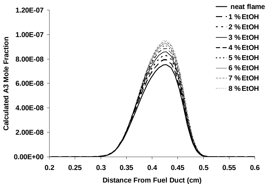
Figure 3.1.6-11. Calculated A3 Mole Fraction Profile for Increasing Amounts of Ethanol Vapor Added to the Fuel Stream.
