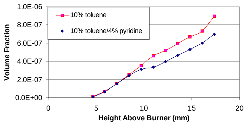
Figure 3.4.4-3. Comparison of Soot Volume Fractions (laser extinction) for Heptane/10% Toluene Flames.
