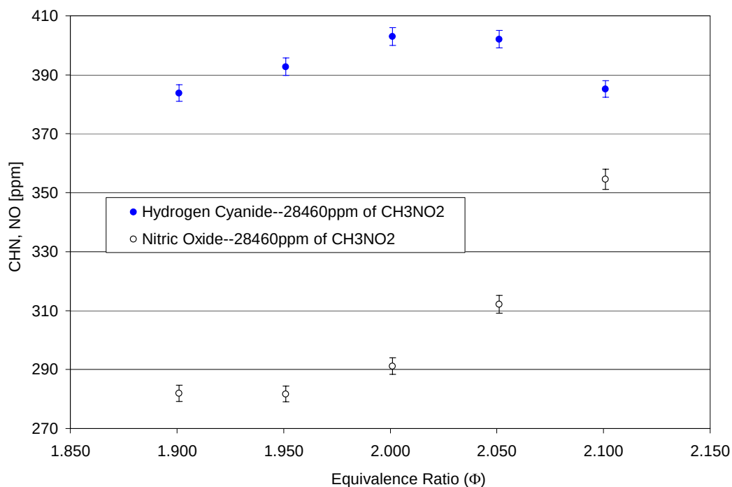
Figure 3.2.3-5. HCN and NO Emissions with Nitromethane Additive. (Neat case emissions were below detectable limits.)
