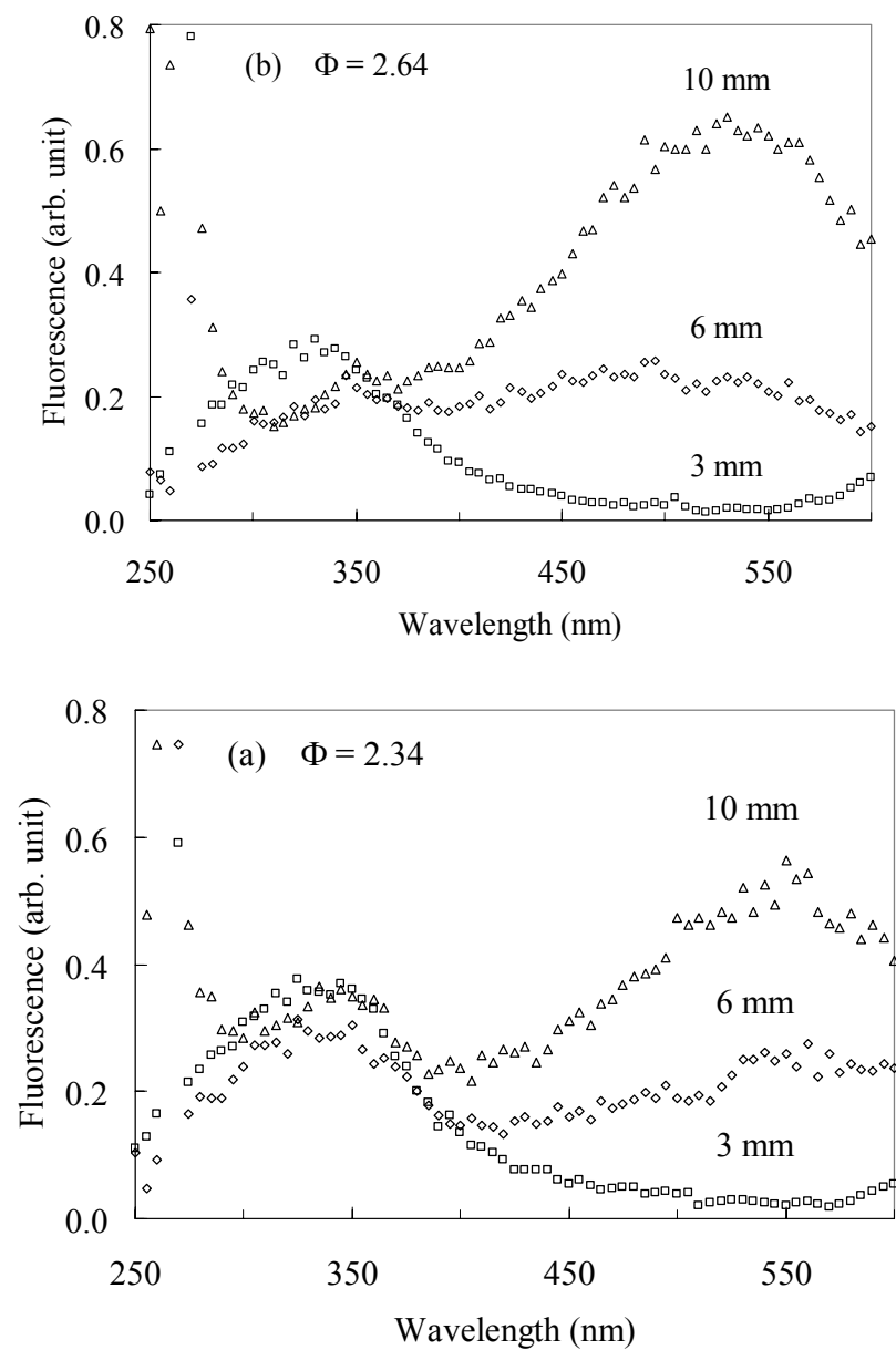
Figure 3.1.5-1. Fluorescence Spectra (a) \Phi = 2.34 ; (b) \Phi = 2.64 .
