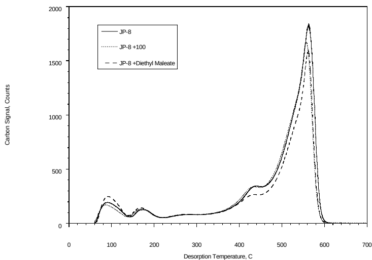
Figure 3.1.2-3. Averaged Carbon Signal Obtained by Desorbing Soot Samples Collected from JP-8 and Additized JP-8 Experiments Listed in Table 2.
