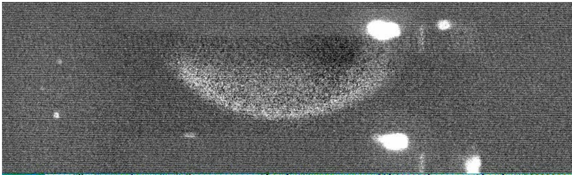
Figure 3.2.5-1. A PLII Image of a Heptane/Air Flame.
