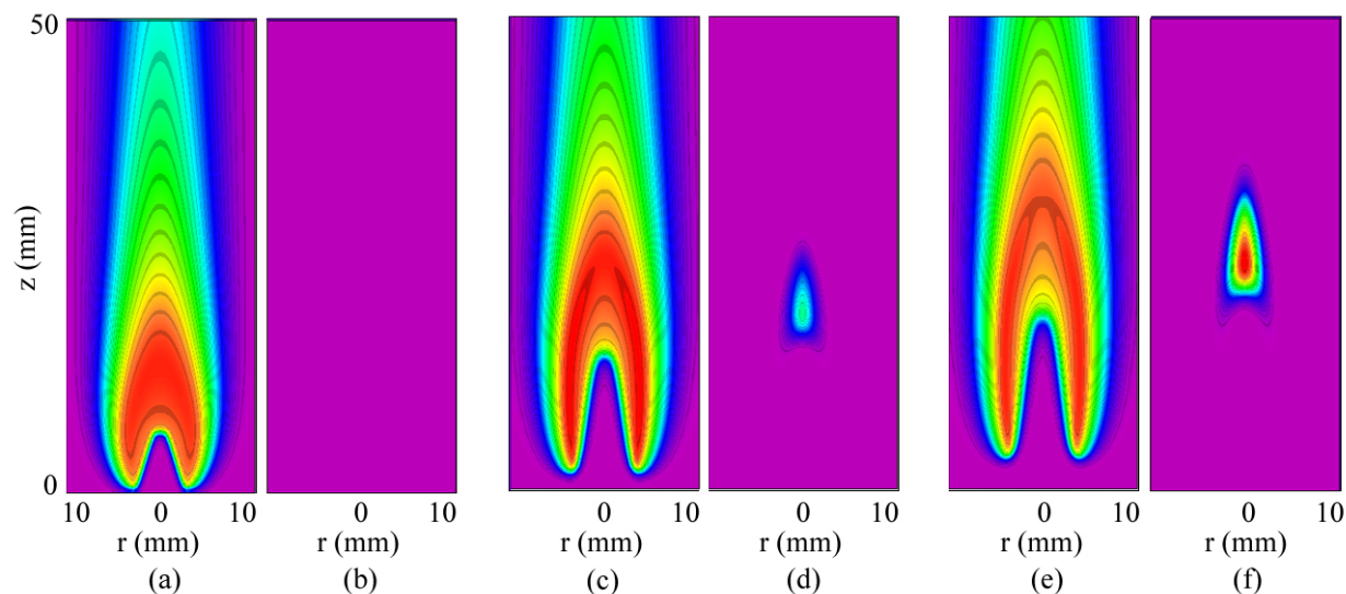
Figure 3.5.8-1. Effect of TMP on Premixed Propane Flame. Mixture of propane, air and TMP with \phi = 1.5 is issued from a 6 mm tube at 0.5 m/s. Distributions of (a) temperature and (b) soot volume fraction for base flame with 0% TMP, (c) and (d) for the flame with 0.1% TMP and (e) and (f) are for the flame with 1% TMP.
