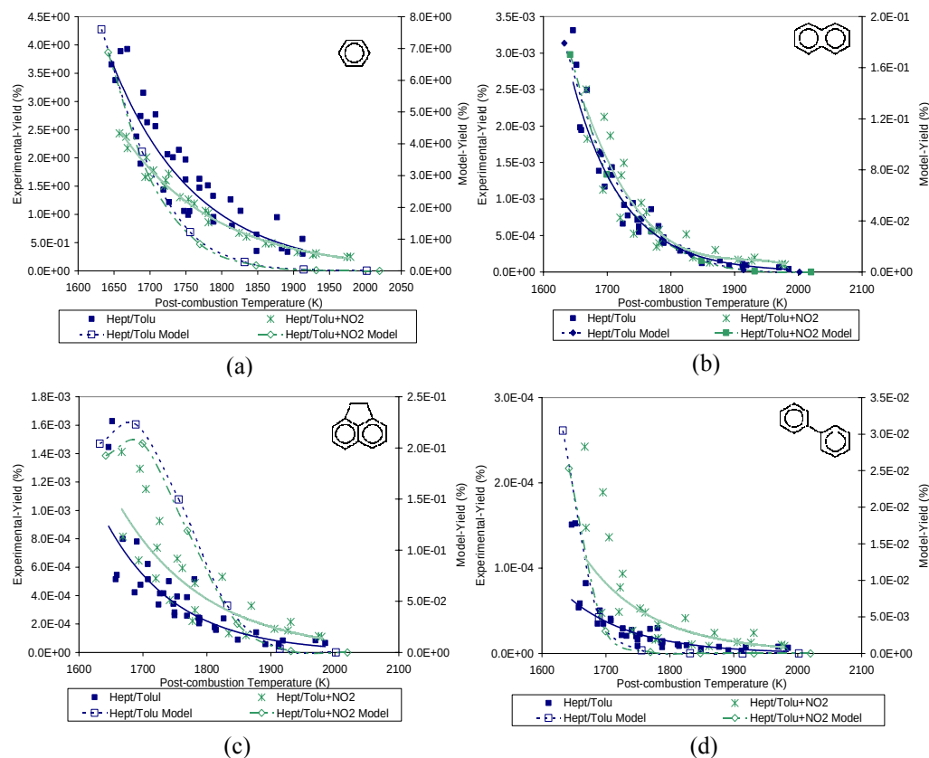
Figure 3.3.2-2. Yields of (a) Benzene, (b) Naphthalene, (c) Acenaphthylene, and (d) Biphenyl from Combustion of n-Heptane/Toluene and n-Heptane/Toluene + NO 2 at 21 atm.
