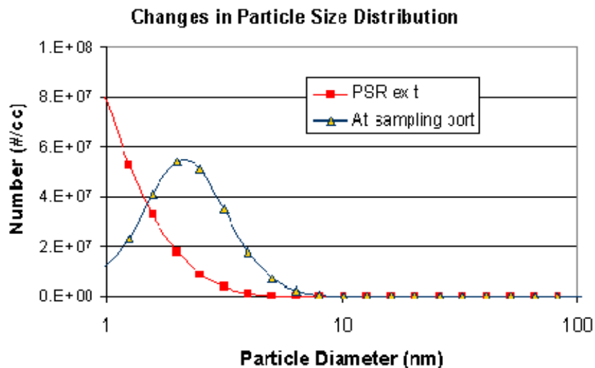
Figure 3.1.3-17. Comparison of Predicted Particle Size Distribution at Reactor Exit with that at the Sampling Port.
