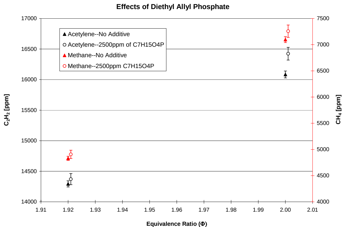
Figure 3.5.3-4. Effect of Diethyl Allyl Phosphate on Acetylene and Methane.
