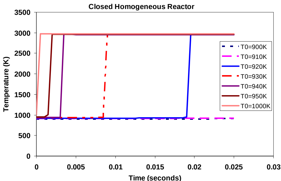
Figure 3.2.5-12. Results of Calculations (closed homogeneous reactor) that Predict Ignition Delay when the IPN Decomposition Products Encounter Oxygen. These calculations were performed to investigate whether an additive could be used to provide decomposition products that could be temperature programmed to react in different combustor zones.
