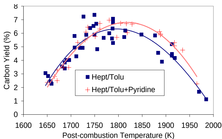
Figure 3.4.2-1. Carbon Yield from Combustion of n-Heptane/Toluene and n-Heptane/Toluene + Pyridine at 21 atm.
