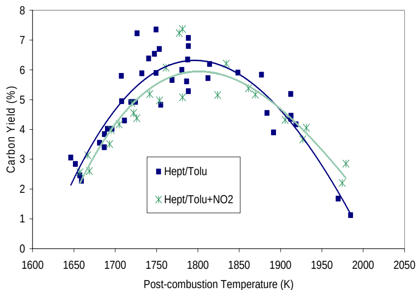
Figure 3.3.2-1. Carbon Yield from Combustion of n-Heptane/Toluene and n-Heptane/Toluene + \text{NO}_2 at 21 atm.
