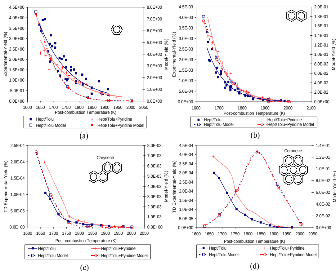
Figure 3.4.2-2. Modeling and Experimental Yields of Volatile, Semivolatile, Nonvolatile Compounds from Combustion of n-Heptane/Toluene and n-Heptane/Toluene + Pyridine at 21 atm.
