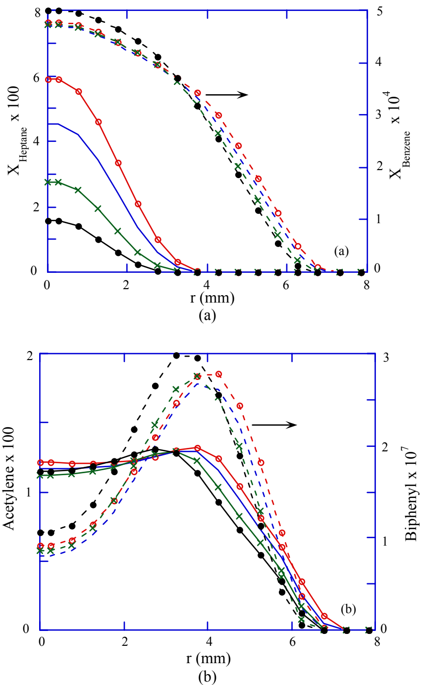
Figure 3.2.8-3. Concentration Distributions of (a) Heptane and Benzene and (b) Acetylene and Biphenyl at a Height of 60 mm Above the Burner.
