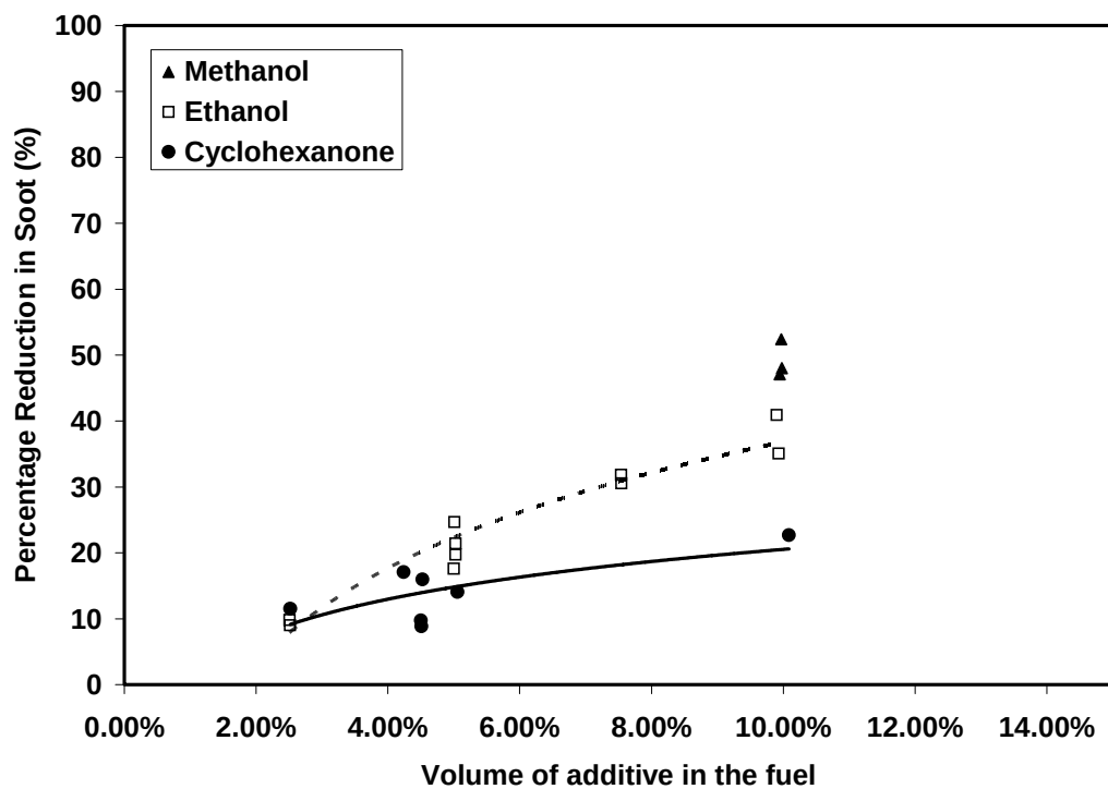
Figure 3.1.8-1. Effect of Oxygenated Additives on Soot Formation with JP-8.
