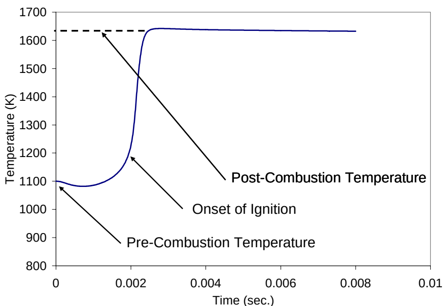
Figure 2.2.1-1. Model Temperature Profile for Heptane/Toluene at 1100 K, 21 atm.
