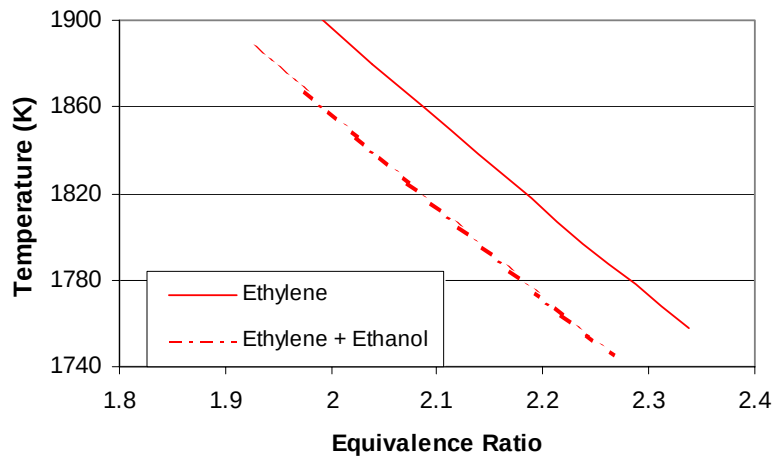
Figure 3.1.3-10. Predicted Temperatures in PSR for Ethylene and Ethylene with Ethanol Additive Using the UTRC Kinetic Mechanism.
