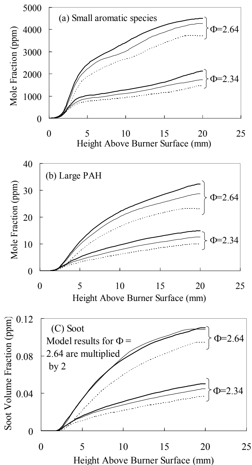
Figure 3.1.5-7. Model Predictions for Effects of Ethanol on (a) Small Aromatic Species, (b) Large PAH, and (c) Soot. Thick solid lines represent baseline, thin solid lines represent 5% oxygen and dotted lines represent 10% oxygen. (Note that model predictions of soot for \Phi=2.64 case are multiplied by a factor of 2 to separate them from the \Phi=2.34 results.)
