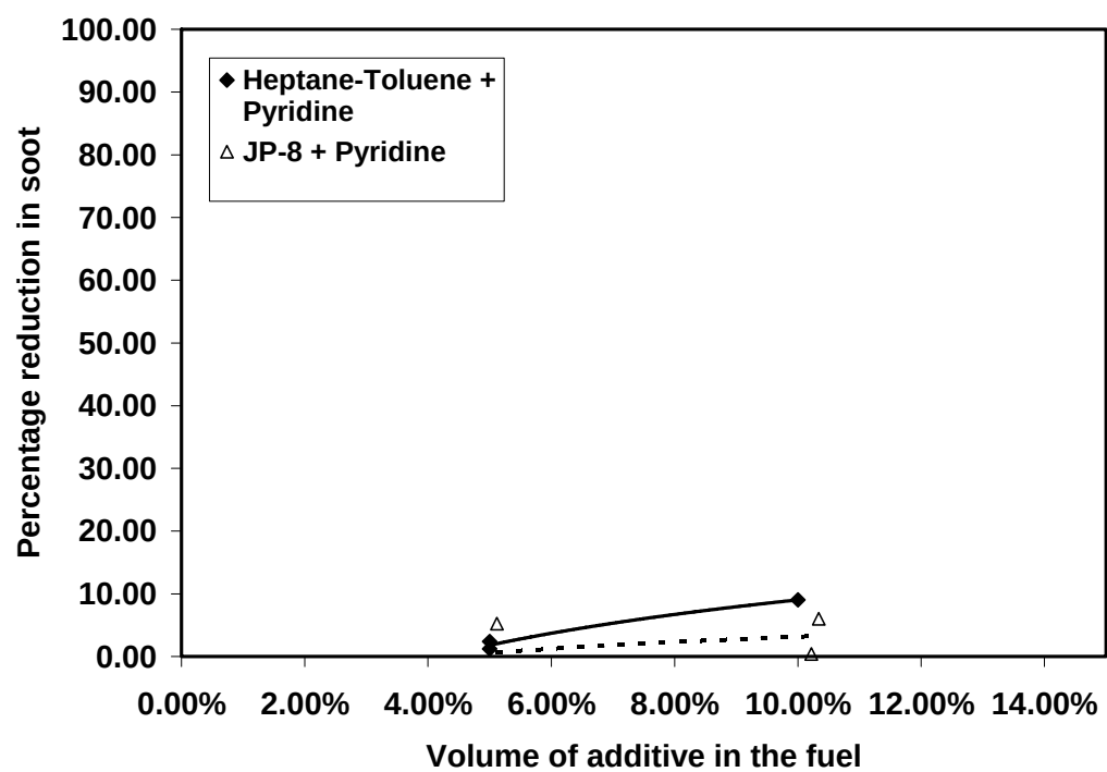
Figure 3.4.6-1. Effect of Pyridine on Soot Formation in the Dump Combustor with JP-8.
