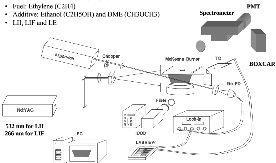
Figure 2.1.3-2. Experimental Setup for Measurements of Soot and PAH.
