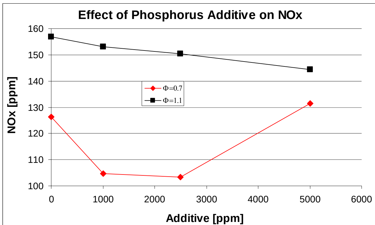
Figure 3.5.7-5. The Effect of the Phosphorus Additive on NO x Emissions.
