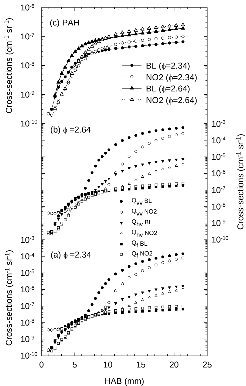
Figure 3.3.3-2. Polarized ( Q_{vv} ), Depolarized ( Q_{hv} ) Scattering and Fluorescence ( Q_f ) Signals for (a) \Phi=2.34 , (b) \Phi=2.64 and (c) PAH vs HAB. Solid symbol: baseline; open symbol: \text{NO}_2 addition.
