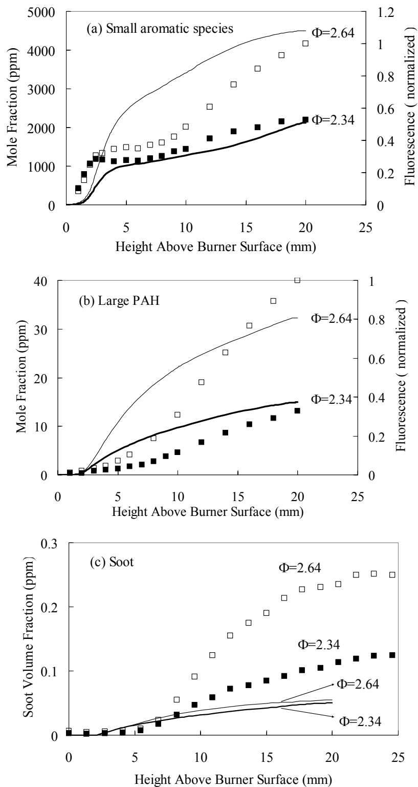
Figure 3.1.5-6. Comparison of Experiments (square symbols) and Model (solid lines) for (a) Small Aromatic Species, (b) Large PAH, and (c) Soot at Base Flames. (LIF data normalized by the maximum signal observed at \Phi=2.64 .)
