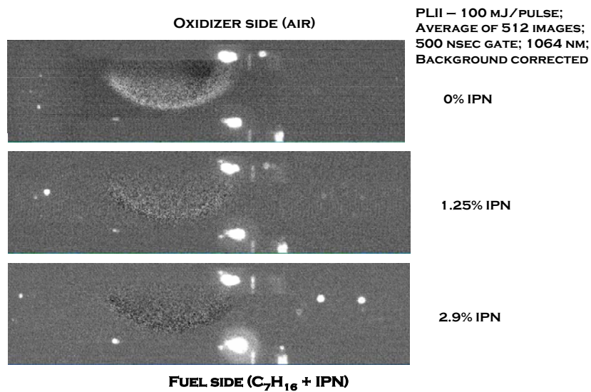
Figure 3.2.5-6. PLII Images of Heptane/Air Flames to which Isopropylnitrate has been Added on the Fuel Side.
