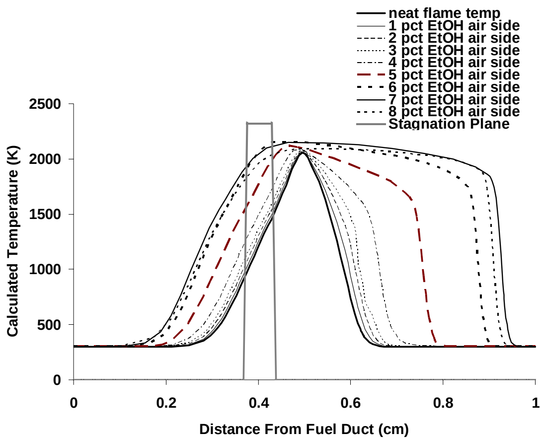
Figure 3.1.6-5. Calculated Temperature Profiles for Air Side Addition of Ethanol. Also shown is calculated position of stagnation plane.
