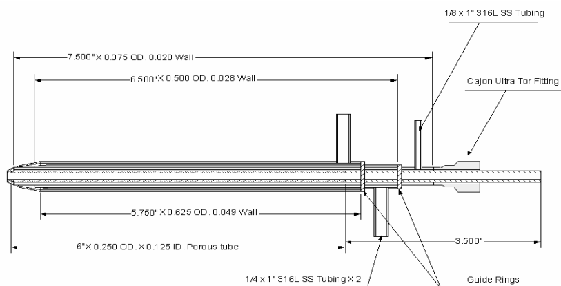
Figure 2.1.4-8. UTRC Porous-Wall Particle Sampling Probe.
