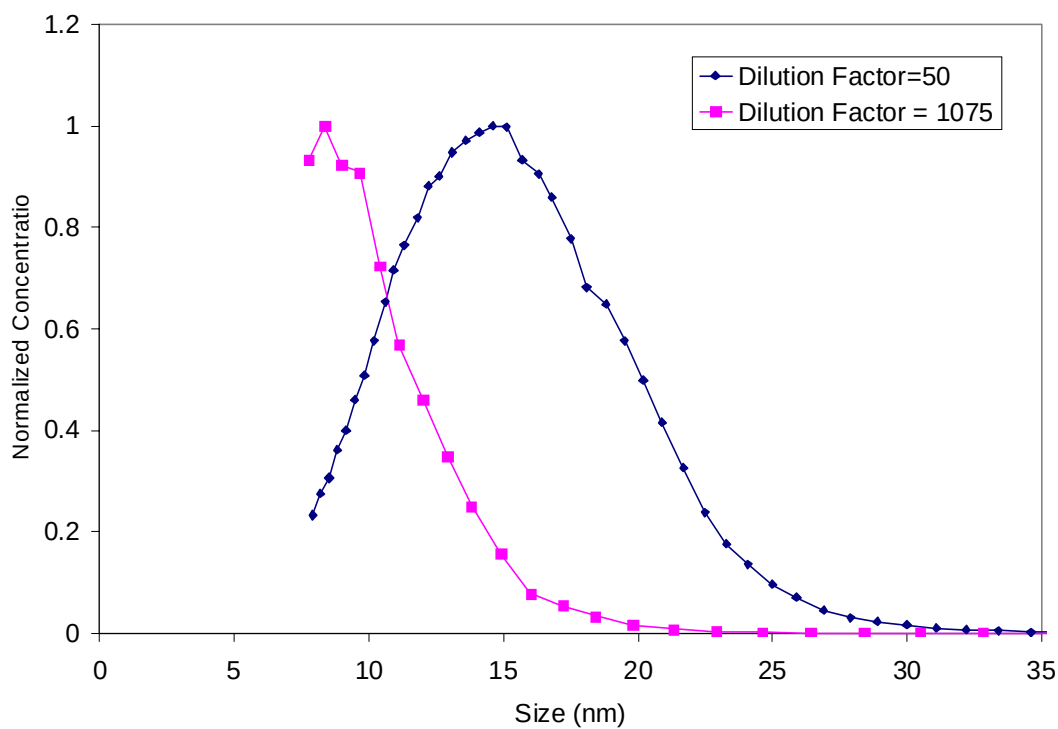
Figure 2.1.2-11. The Effect of Dilution Ratio on the Normalized Particle Size Distribution for the WSR (Fuel: 80%Heptane/20%Toluene).
