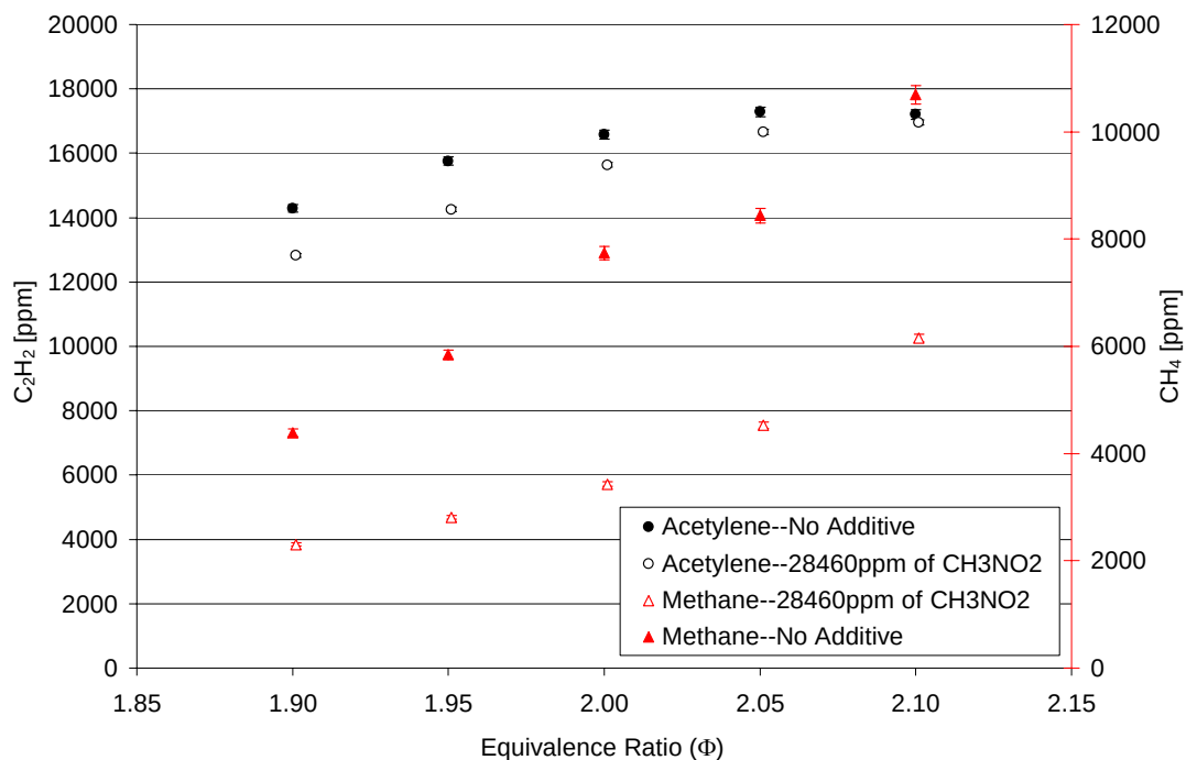
Figure 3.2.3-3. Effect of Nitromethane on Methane and Acetylene Emissions from the WSR.
