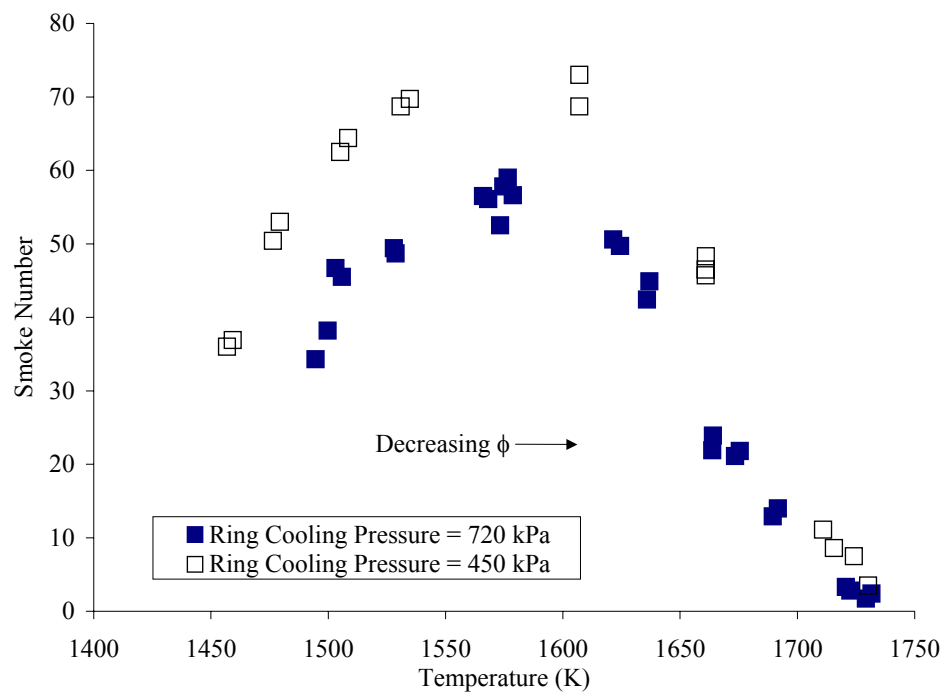
Figure 3.1.3-4. Smoke Number vs Temperature for Ethylene Air Cases Effect of Ring Cooling.
