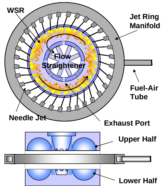
Figure 2.1.2-1. Schematic of Toroidal WSR.
