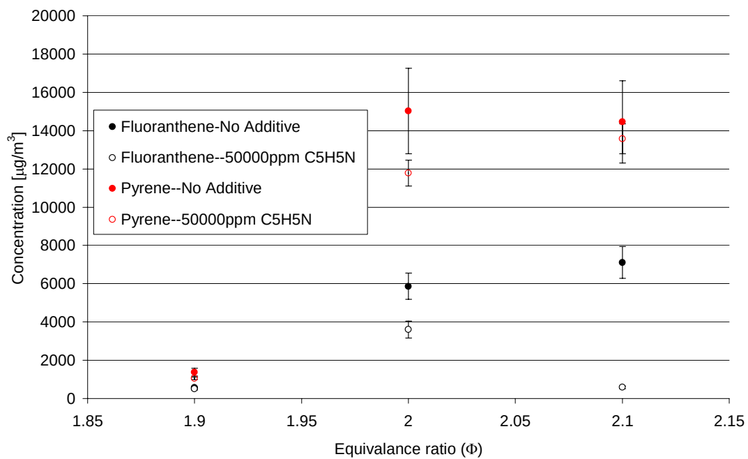
Figure 3.4.3-5. Effect of Pyridine on Fluoranthene and Pyrene.
