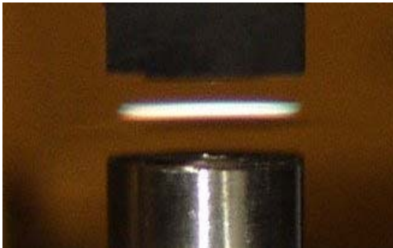
Figure 2.1.5-5. Detail of an Ethylene/Air Opposed Flow Flame.
