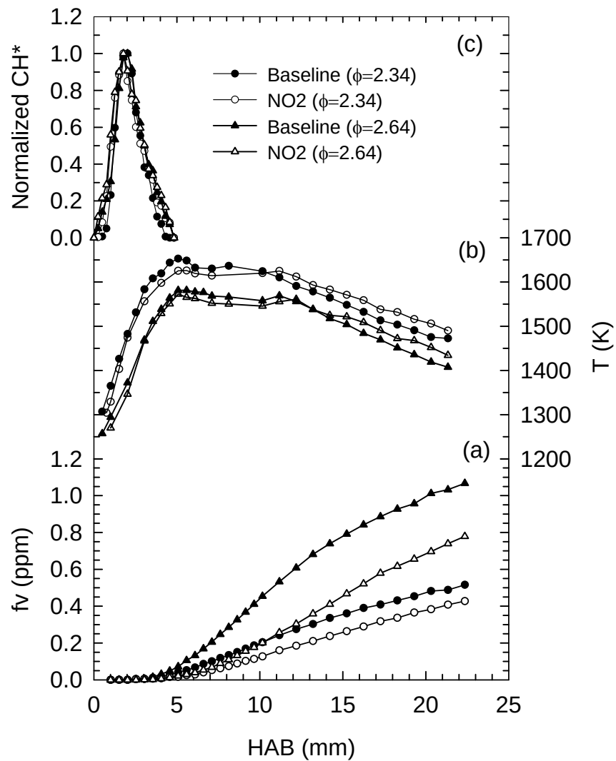
Figure 3.3.3-1. The Axial Profiles of (a) f_v , (b) Temperature and (c) Normalized CH* Emissions for Two Equivalence Ratio of 2.34 and 2.64. Solid symbol: baseline; open symbol: NO 2 addition.
