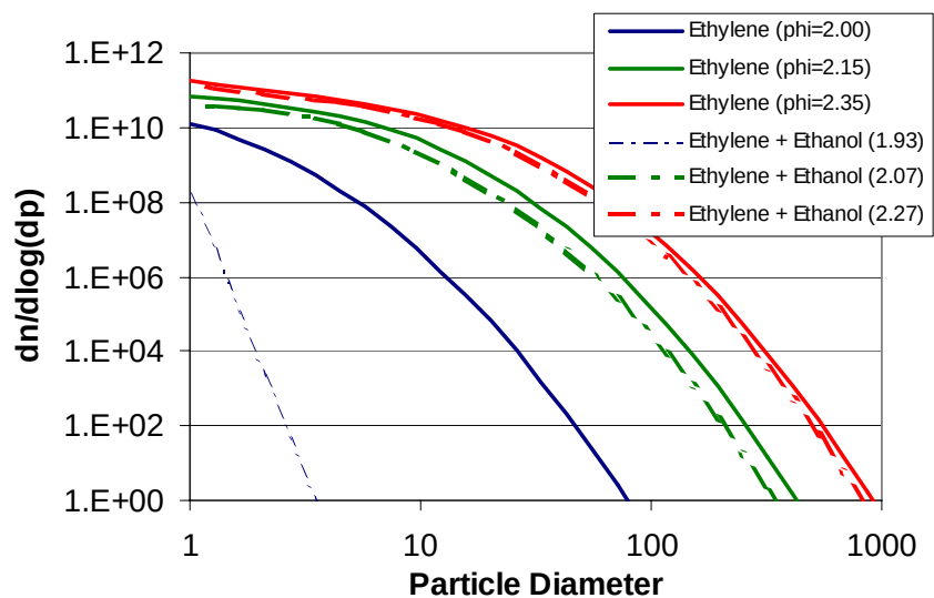
Figure 3.1.3-12. Predicted Particle Size Distributions for PSR Using UTRC Mechanism.
