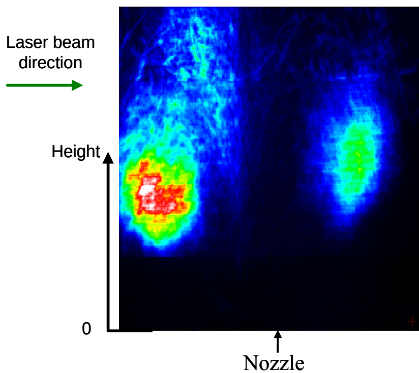
Figure 3.1.7-1. Sample Averaged LII Image from Heptane Spray Flame.
