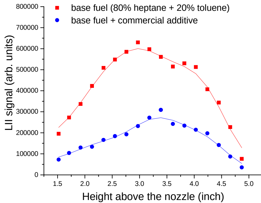
Figure 3.2.6-2. Effects of Commercial Additive on Soot.
