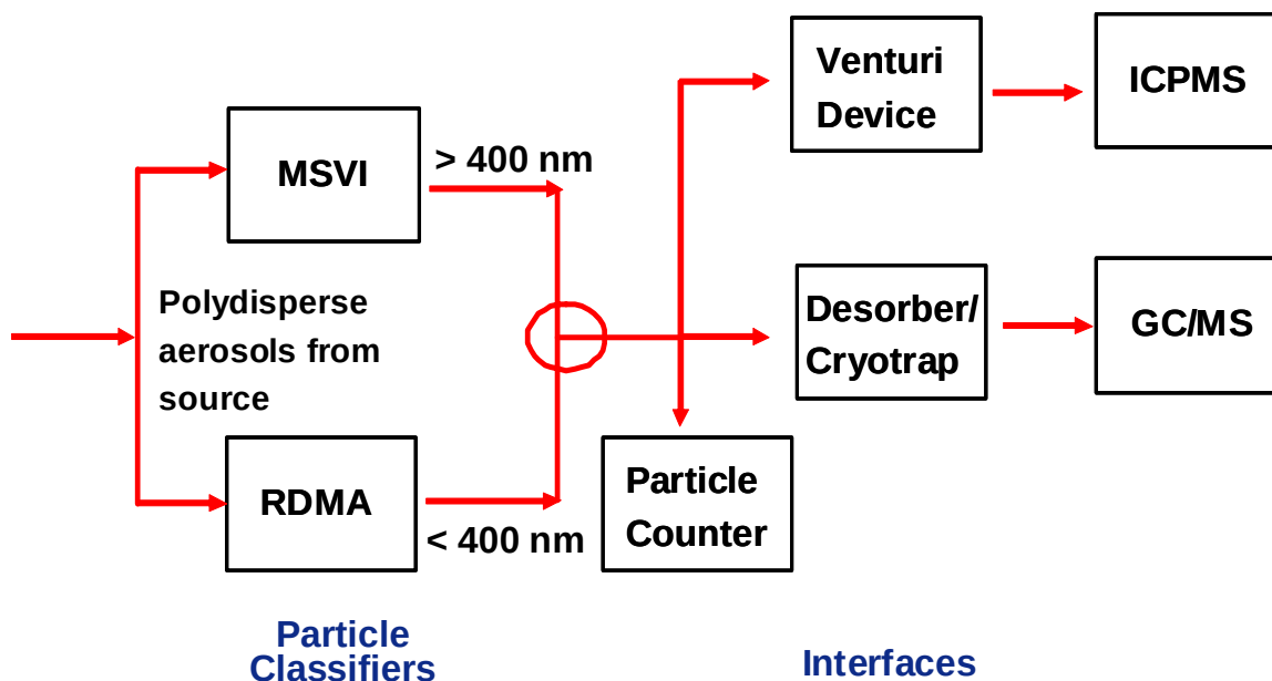
Figure 2.1.2-8. Diagram of Major PMCMS Subsystems.
