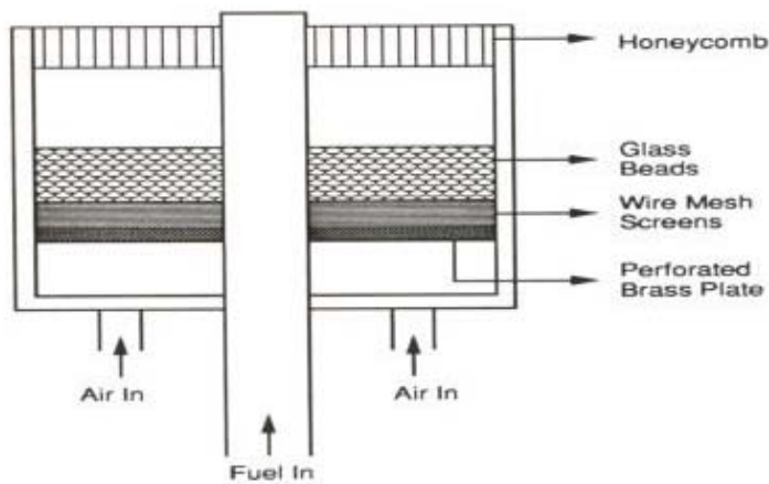
Figure 2.1.6-1. Schematic of Coflow Diffusion Flame Burner.
