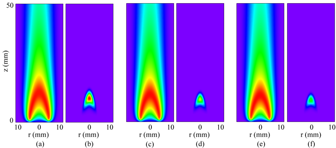
Figure 3.5.8-3. Effect of TMP on Methane Jet Diffusion Flame. Distributions of (a) temperature and (b) soot volume fraction for base flame with 0% TMP, (c) and (d) for the flame with 0.1% TMP, and (e) and (f) are for the flame with 1% TMP.
