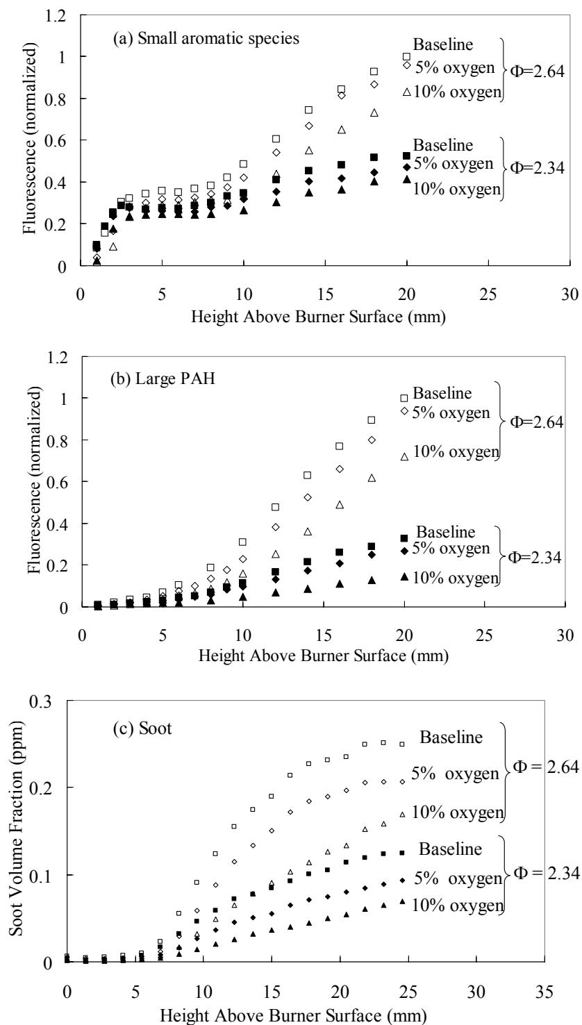
Figure 3.1.5-4. Effects of Ethanol on (a) Small Aromatic Species, (b) Large PAH, and (c) Soot for Ethylene-Air Flames. (Note that the PAH data are normalized by the maximum signal observed at \phi=2.64 ).
