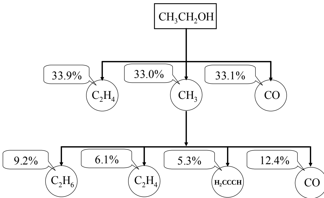
Figure 3.1.5-9. Carbon Flux Diagram for Ethanol at \Phi=2.34 . (Percentage indicates the fraction of carbon from ethanol passing through the species shown.)
