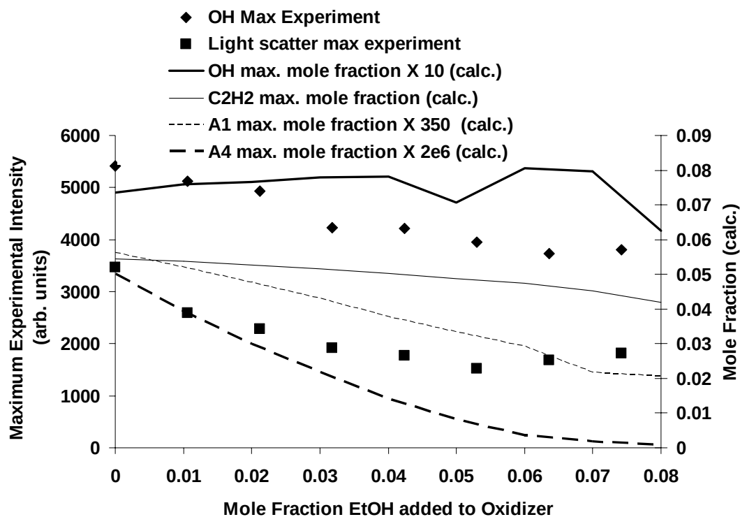
Figure 3.1.6-3. Graph of Experimental Measurements and Predictions Based Upon Calculations for OH, Soot and Soot Precursors, for Air Side Addition of Ethanol.
