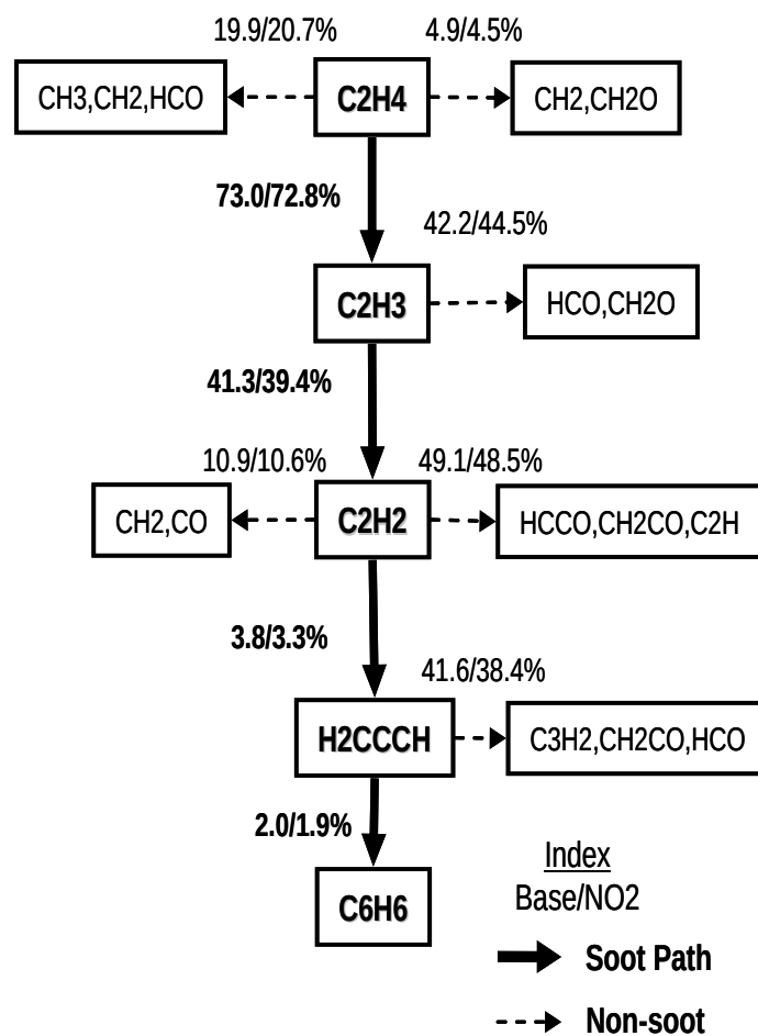
Figure 3.3.3-3. Absolute Carbon Flux Map Comparing Baseline and NO 2 Addition for \Phi=2.64 .
