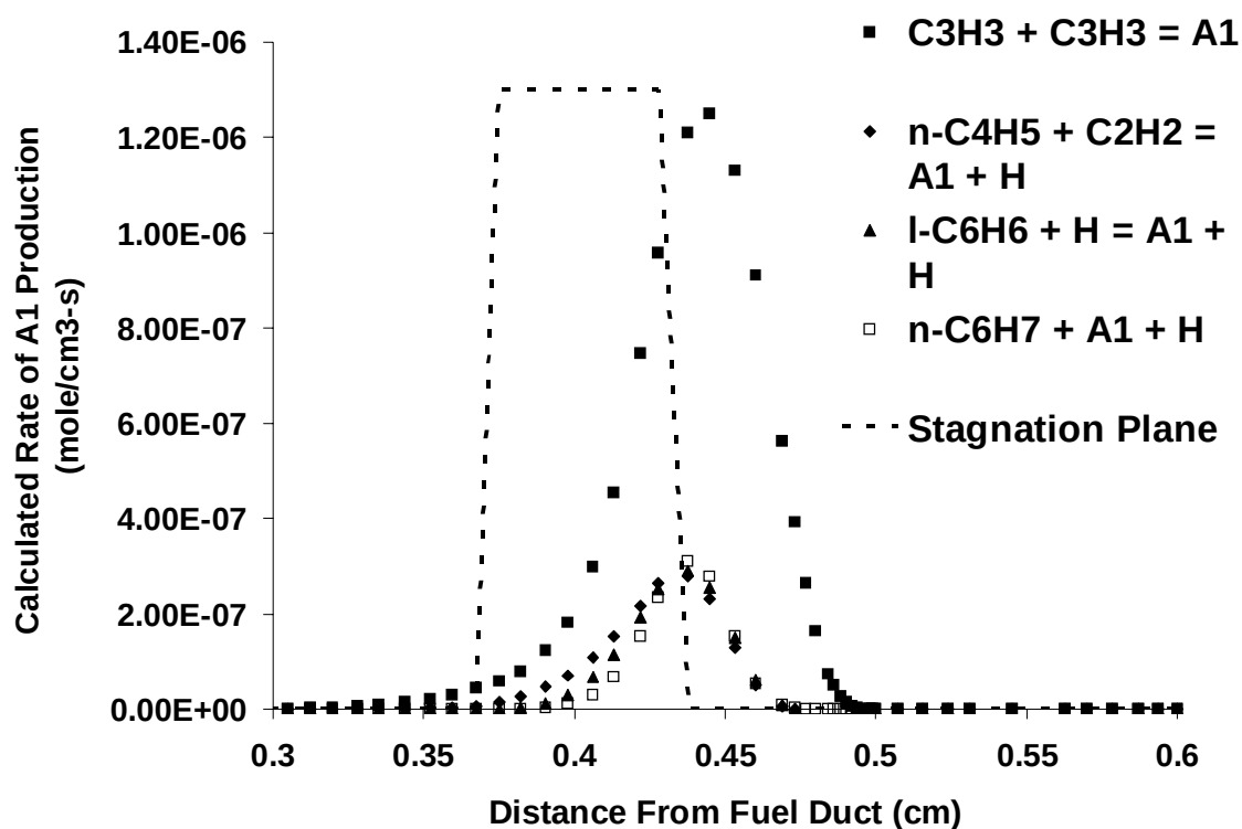
Figure 3.1.6-2. Calculated Rates of Production of A1 vs Distance from the Fuel Duct for the Top Four Contributing Reactions in the Mechanism (out of 15 reactions in the mechanism involving A1). Calculation is for the neat ethylene/air opposed flow diffusion flame. Also shown is calculated position of stagnation plane.
