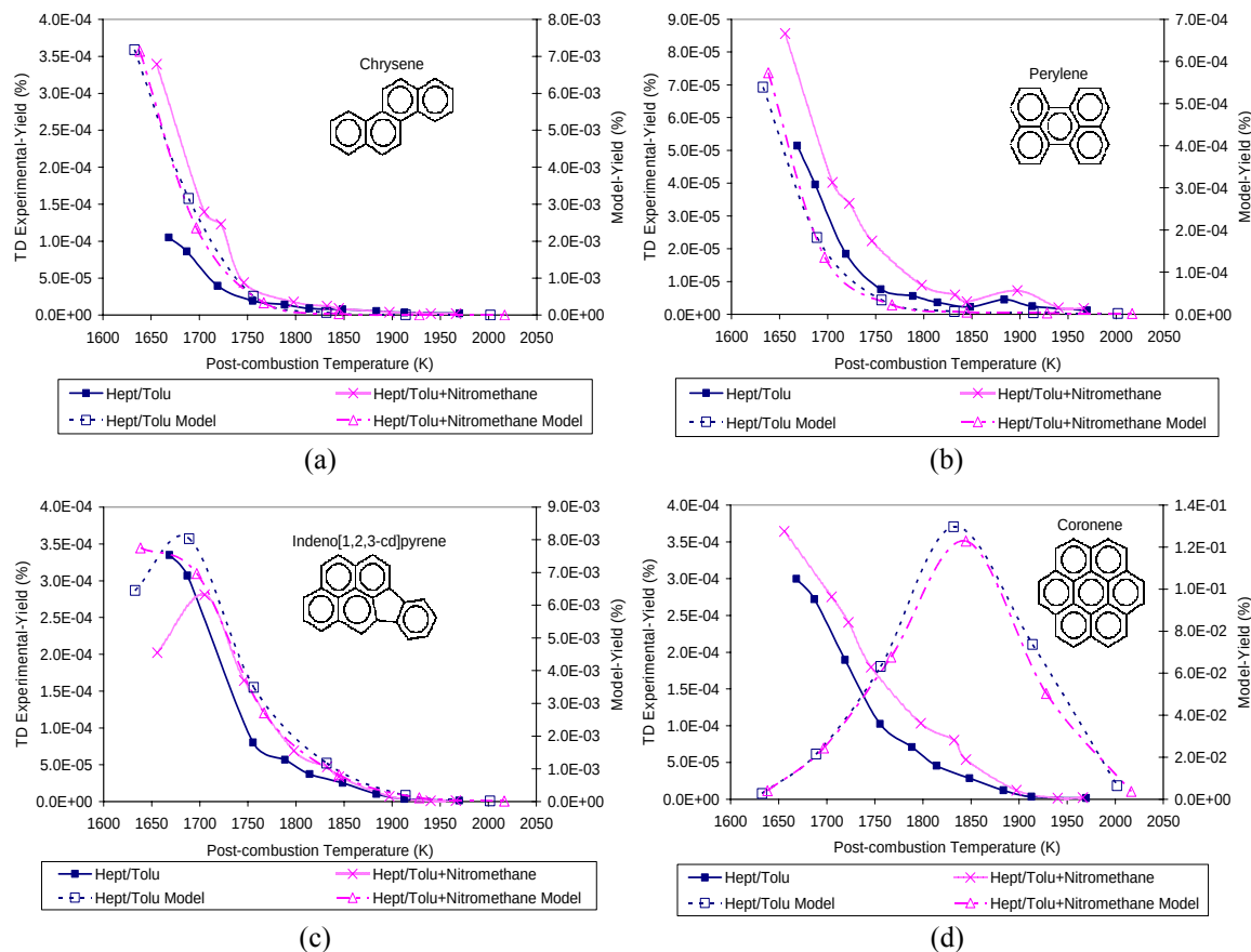
Figure 3.2.2-3. Yields of (a) Chrysene, (b) Perylene, (c) Indeno[1,2,3-cd]Pyrene, and (d) Coronene from Combustion of n-Heptane/Toluene and n-Heptane/Toluene + Nitromethane at 21 atm.
