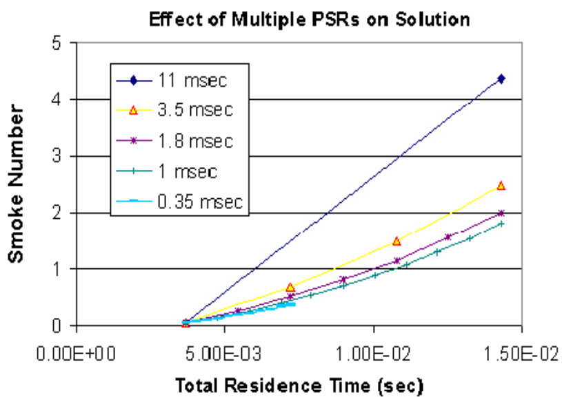
Figure 3.1.3-16. Effect of Multiple Reactors in Simulating the Exhaust from the Stirred Reactor.
