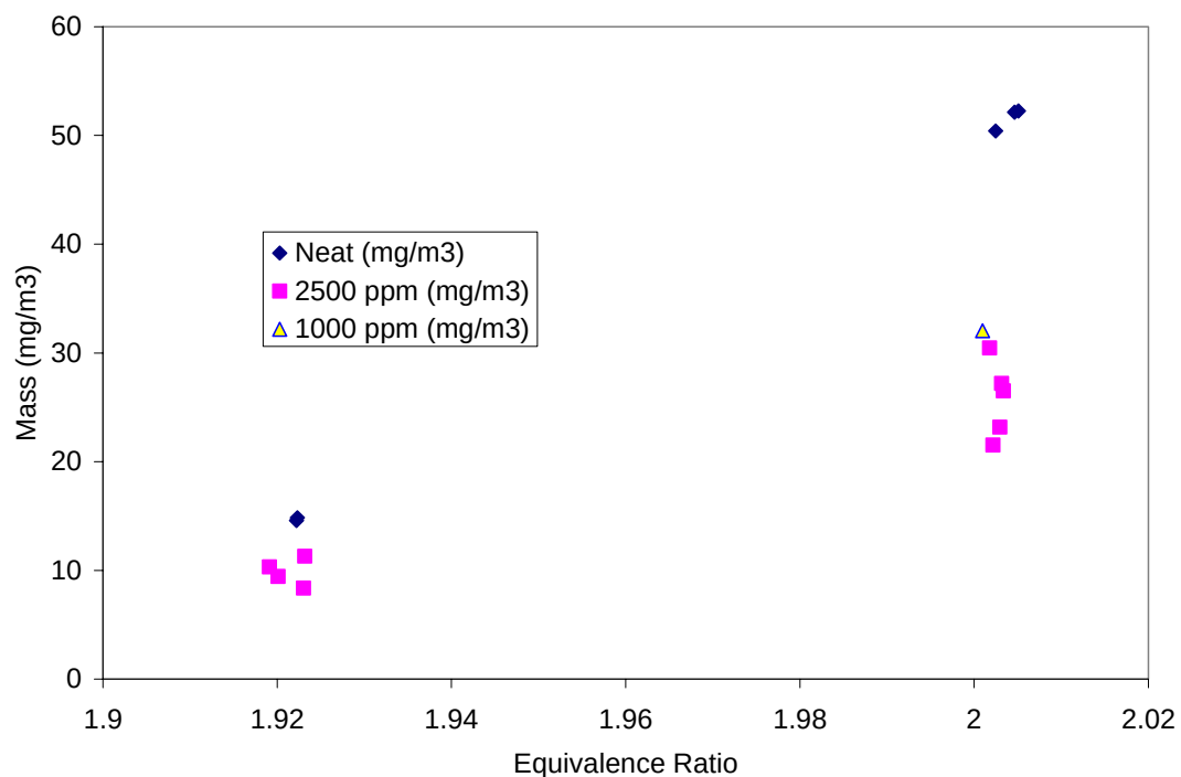
Figure 3.5.3-2. The Effect of Diethyl Allyl Phosphate on the Volatile Carbon Mass from Samples in the WSR.
