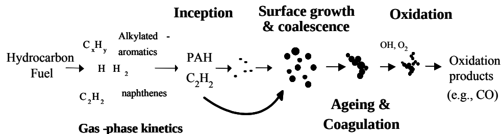
Figure 2.2.2-2. Sequence for Soot Formation and Oxidation.
