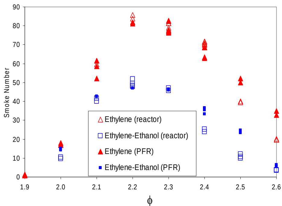
Figure 3.1.3-5. Smoke Number Results for Neat Ethylene and Ethanol Additive.
