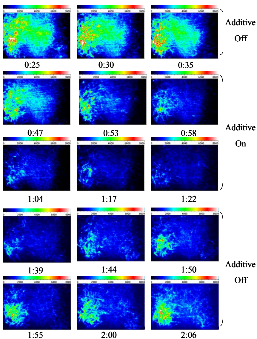
Figure 3.2.6-1. Series of LII Images Illustrating the Time Dependent Behavior of the Commercial Additive.
