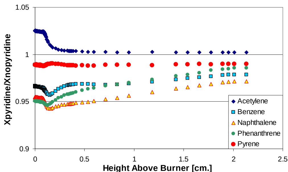
Figure 3.4.4-6. Normalized Concentrations of Key Species in Fuel-Rich Premixed Flames with Added Pyridine.
