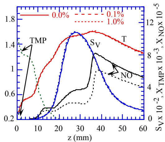
Figure 3.5.8-5. Effect of TMP on Heptane Jet Diffusion Flame. Distributions of T and species along the centerline.
