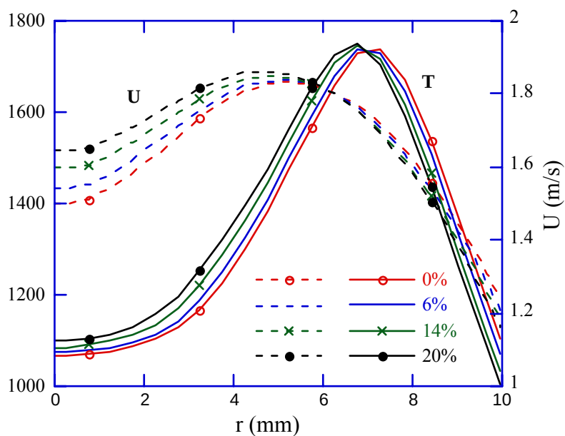
Figure 3.2.8-2. Distributions of Axial Velocity and Temperature at a Height of 60 mm Above the Burner.
