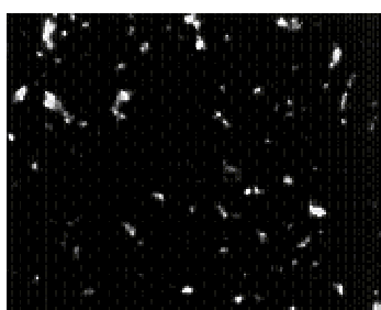
nitromethane
