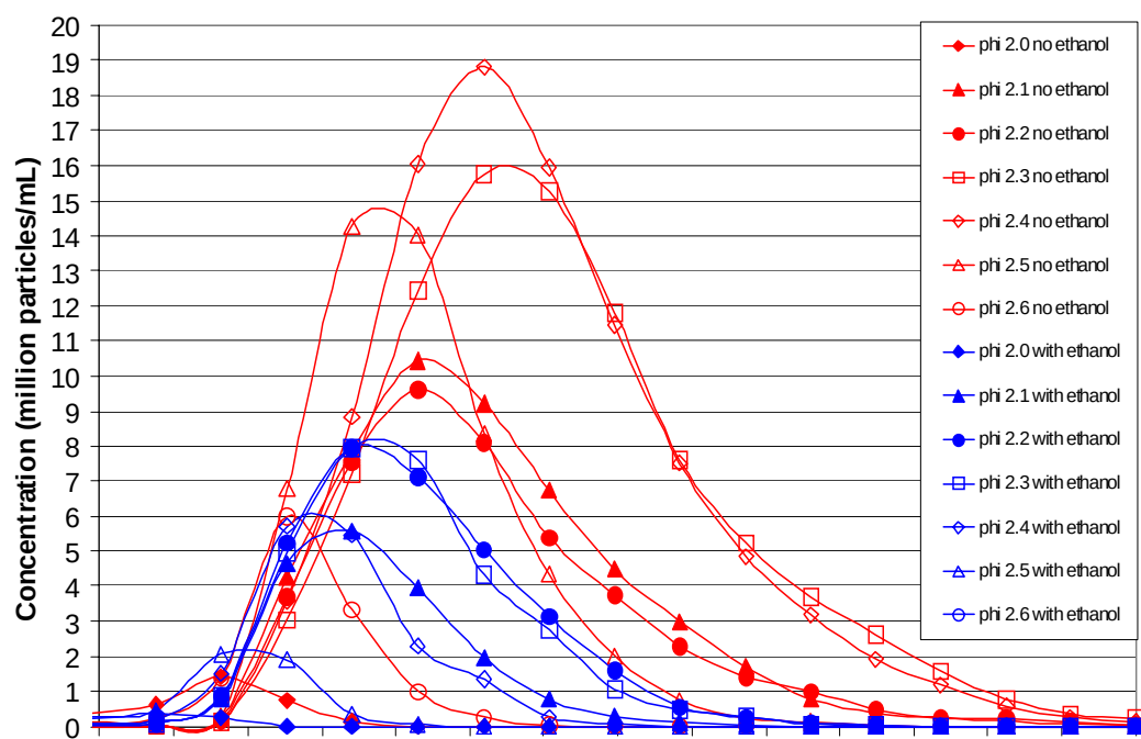
Figure 3.1.3-8. Particle Size Distributions for Ethylene and Ethanol Additive Cases.
