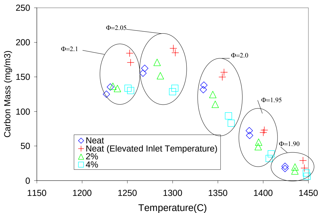
Figure 3.2.3-8. Total Carbon Mass for Nitropropane Additive Cases Studied in the WSR.
