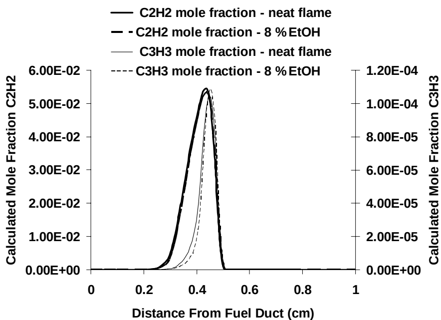
Figure 3.1.6-13. Calculated Acetylene ( C_2H_2 ) and Propargyl ( C_3H_3 ) Profiles for Neat Flames and for Flames with 8% Ethanol Vapor Added to the Fuel Stream. Intermediate values of ethanol addition yield C_2H_2 and C_3H_3 profiles between those for the extreme values. Note that the calculation predicts negligible change in C_2H_2 and C_3H_3 for fuel side addition of ethanol.
