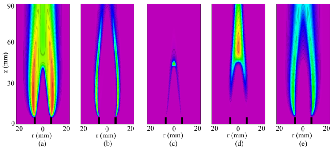
Figure 3.5.8-7. Heptane Premixed Flame with 0.1% TMP. Mixture of heptane and air with \phi = 2.0 is issued from a 13 mm tube at 1.0 m/s. Distributions of (a) temperature, (b) OH, (c) benzene, (d) soot volume fraction, and (e) NO.
