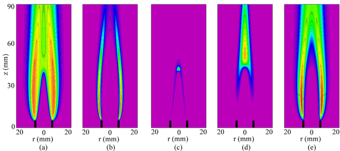
Figure 3.5.8-6. Heptane Premixed Flame with 0% TMP. Mixture of heptane and air with \phi = 2.0 is issued from a 13 mm tube at 1.0 m/s. Distributions of (a) temperature, (b) OH, (c) benzene, (d) soot volume fraction, and (e) NO.
