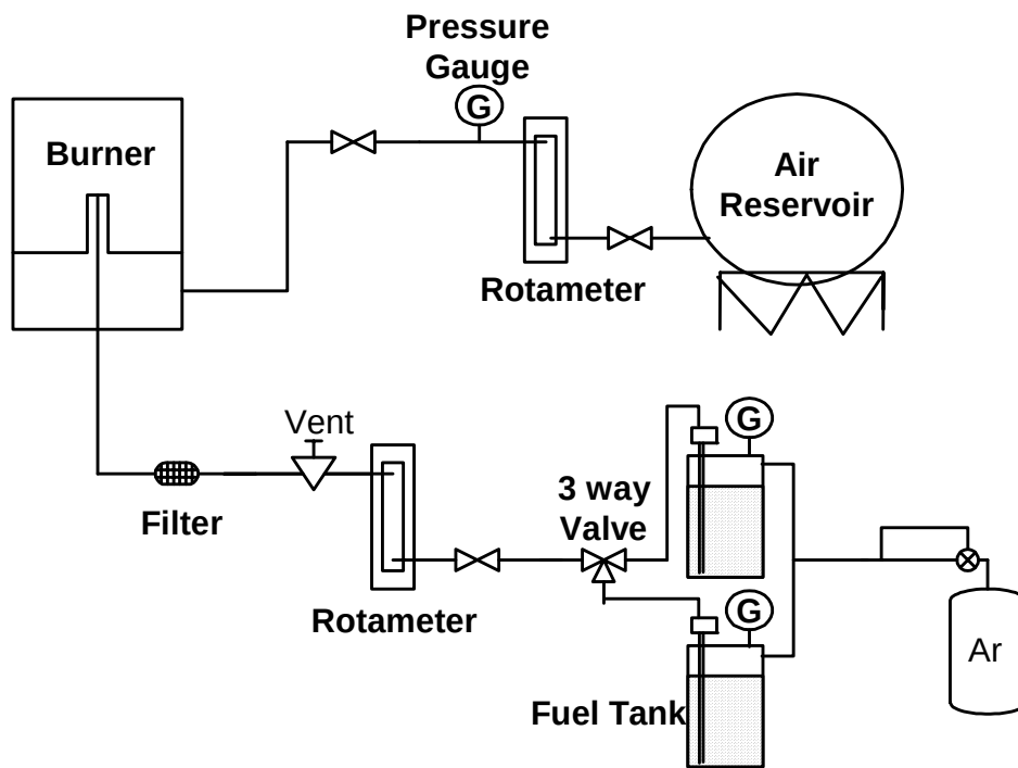
Figure 2.1.7-3. Flow Control System for Turbulent Spray Burner.
