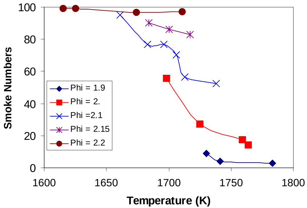
Figure 3.1.3-2. Smoke Number vs Temperature for Neat and Additive Cases.
