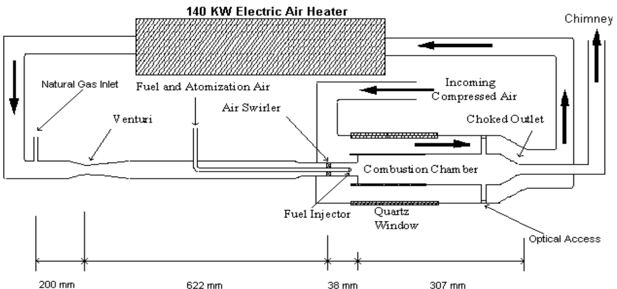
Figure 2.1.8-1. Schematic Diagram of High Pressure Turbulent Reactor.
