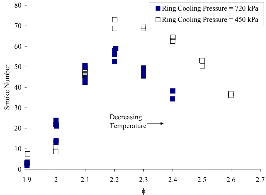
Figure 3.1.3-3. Smoke Number vs Equivalence Ratio for Ethylene-Air Mixtures Effect of Cooling.
