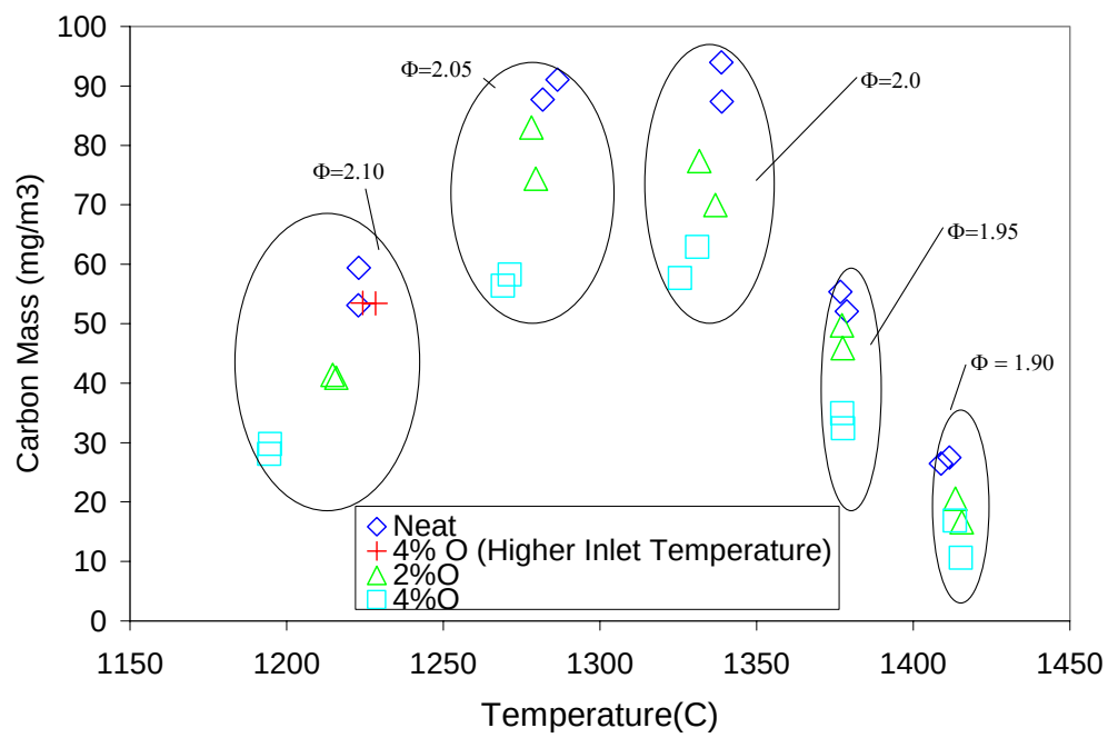
Figure 3.1.3-19. Carbonaceous Carbon Mass for Cyclohexanone Additive.
