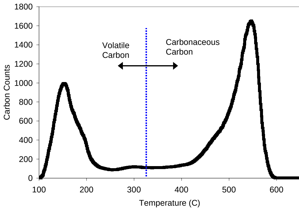
Figure 2.1.2-5. Carbon Signal vs Burn-off Temperature for a Typical Quartz Filter Sample.
