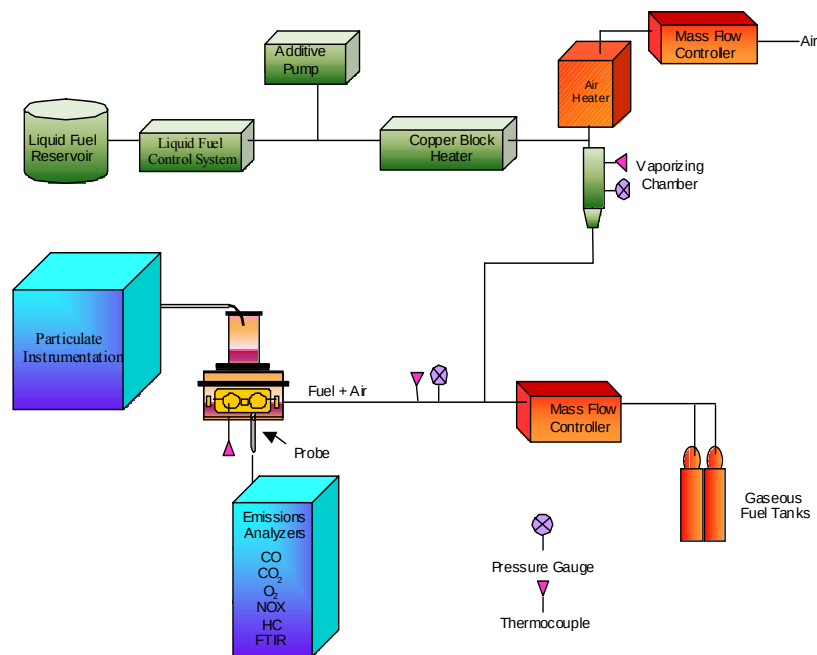
Figure 2.1.2-4. Well-Stirred Reactor Air, Fuel and Instrumentation Systems.
