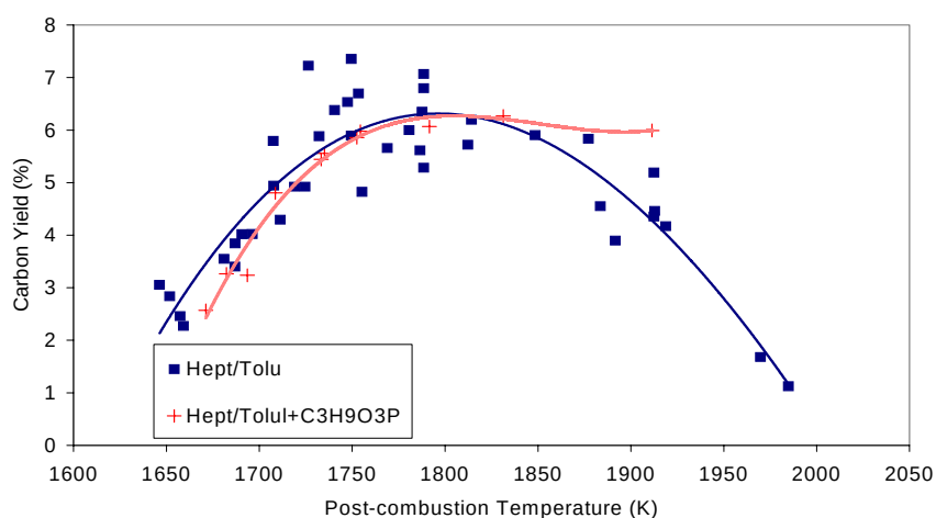
Figure 3.5.2-1. Carbon Yield from Combustion of Heptane/Toluene and Heptane/Toluene+(25K ppm) Trimethyl Phosphite.
