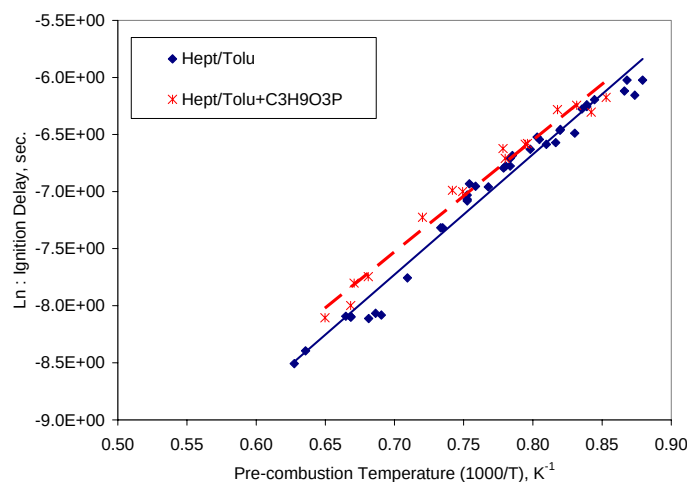
Figure 3.5.2-2. Ignition Delay from Combustion of Heptane/Toluene and Heptane/Toluene+(25K ppm) Trimethyl Phosphite.
