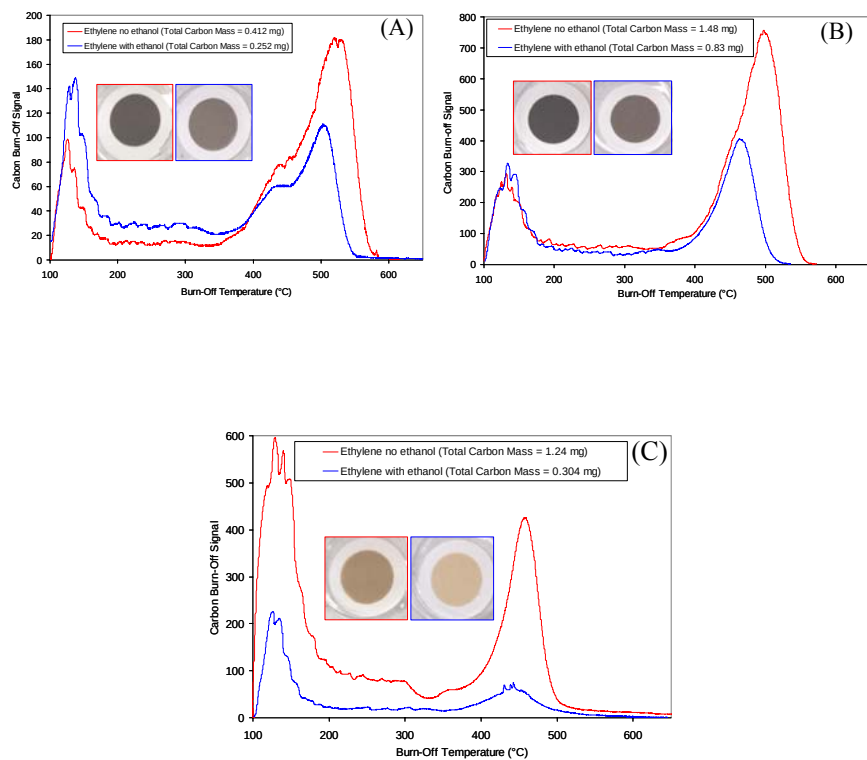
Figure 3.1.3-7. Carbon Mass Measurement vs Filter Temperature During Carbon Oxidation, A ( \phi = 2.1 ), B ( \phi = 2.3 ), and C ( \phi = 2.6 ).
