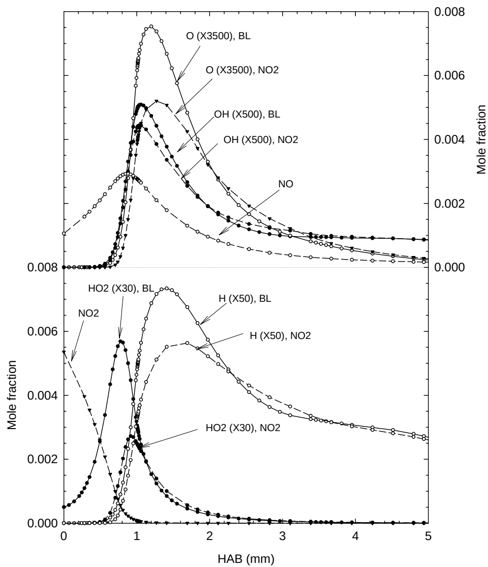
Figure 3.3.3-4 . Minor Species at \Phi=2.64 . Solid line: baseline; open line: \text{NO}_2 addition.
