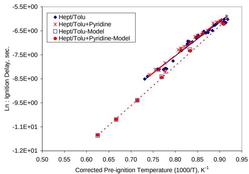
Figure 3.4.2-3. Ignition Delay from Combustion of Heptane/Toluene + Pyridine at 21 atm.
