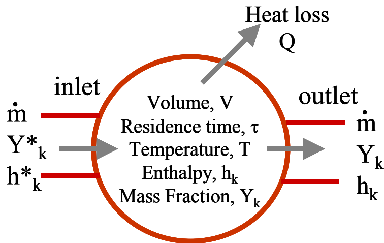
Figure 2.2.2-1. Schematic of Perfectly Stirred Reactor.
