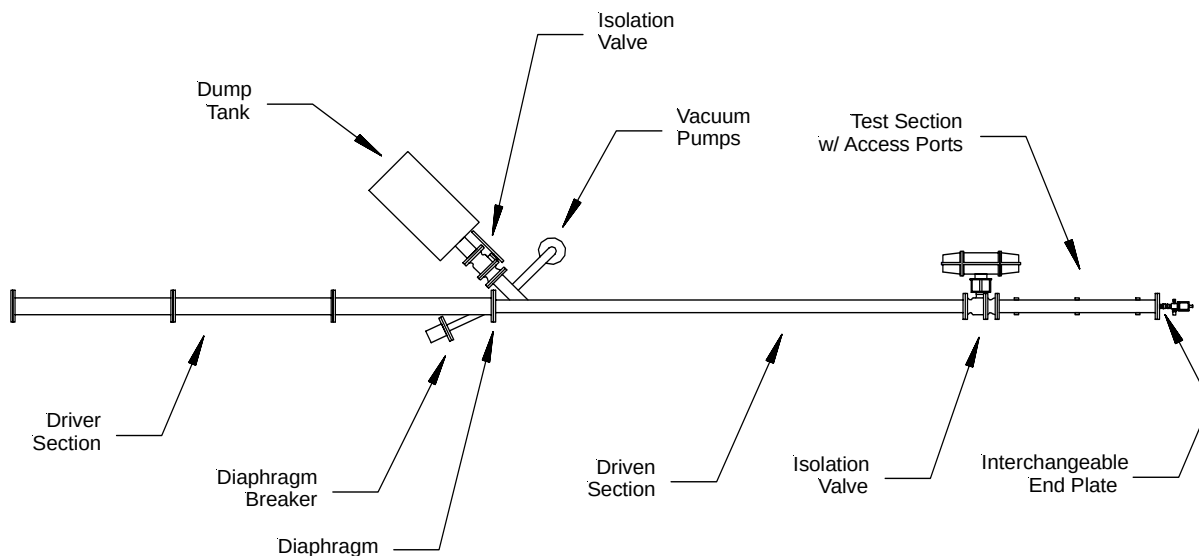
Figure 2.1.1-1. General Schematic of the Shock Tube.
