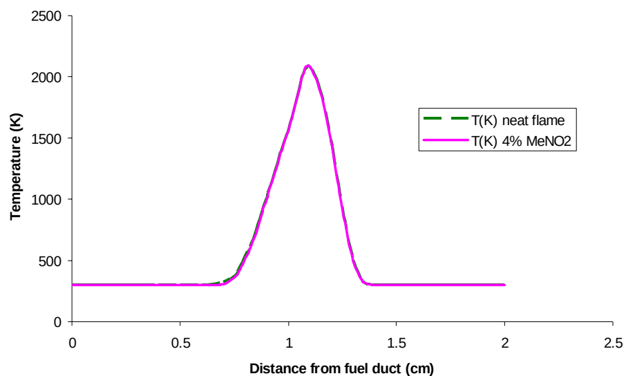
Figure 3.2.5-4. Calculated Temperature for Neat Ethylene/Air Flames and Ethylene/Air Flames to which 4 Mole Percent Nitromethane has been Added to the Fuel Side.
