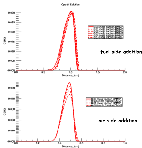
Figure 3.5.6-10. Calculated C 2 H 2 Concentration vs Flame Position (centerline) for Fuel and Oxidizer Side Addition to Ethylene/Air Opposed Flow Flames.
