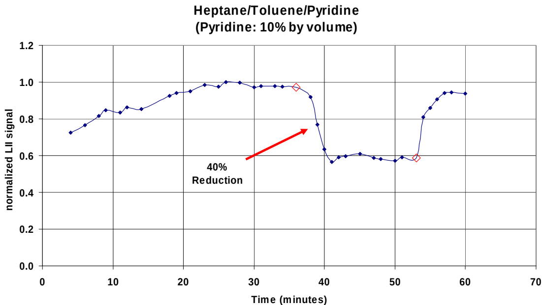
Figure 3.4.5-1. Effect of Pyridine on Soot in the Turbulent Spray Flame.
