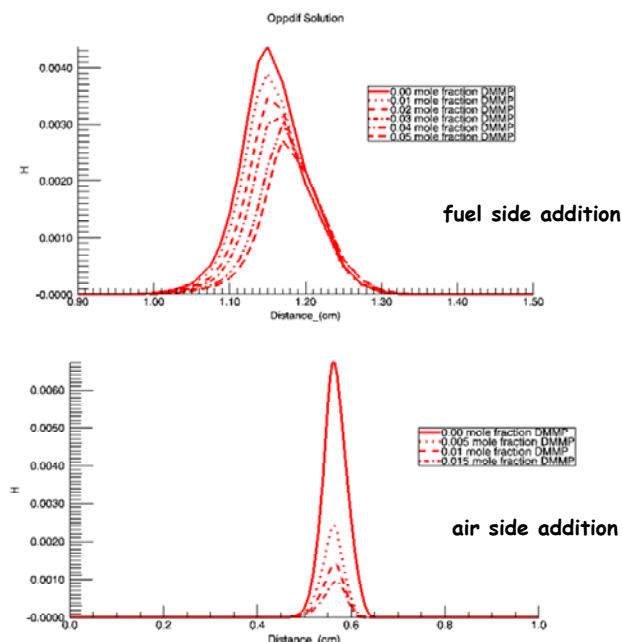
Figure 3.5.6-9. Calculated H Atom Concentration vs Flame Position (centerline) for Fuel and Oxidizer Side Addition to Ethylene/Air Opposed Flow Flames.
