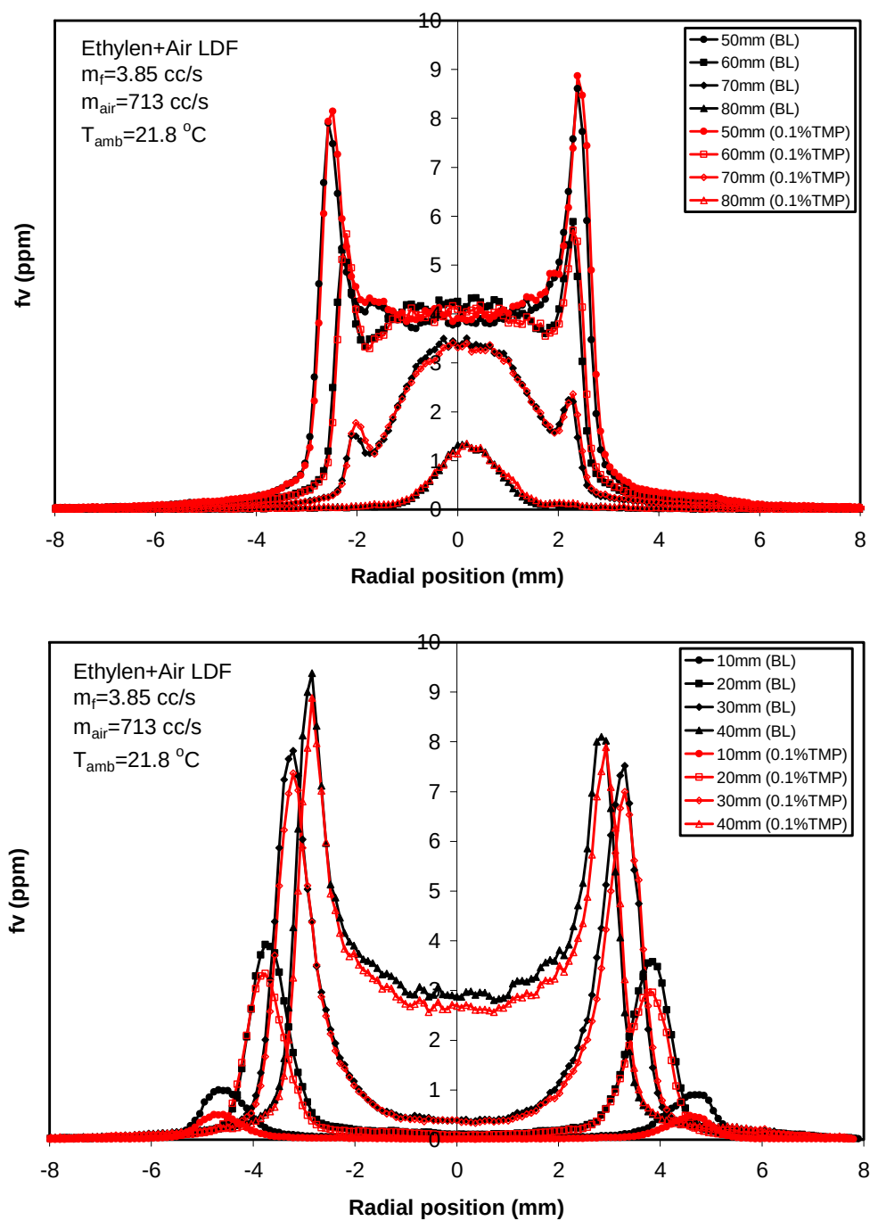
Figure 3.5.5-2. Soot Volume Fraction Profiles for Ethylene Flame with Baseline and TMP Addition.
