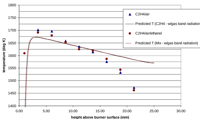
Figure 3.1.4-1. Temperature Along the Centerline of Flame 1 and 2.
