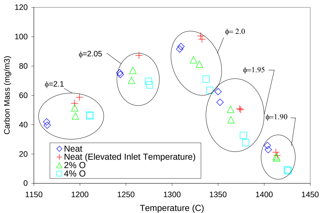
Figure 3.2.3-2. Carbonaceous Carbon Mass for the Nitromethane Additive Cases Studied in the WSR.
