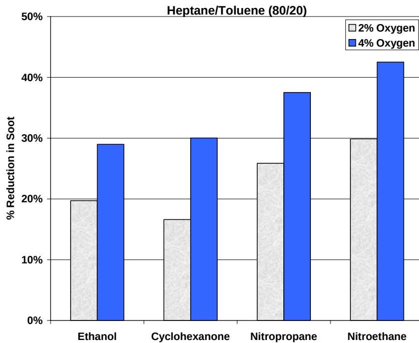
Figure 3.2.6-3. Effect of Individual Components of the Commercial Additive on Soot (ethanol included for comparison purposes).
