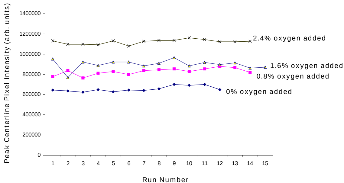
Figure 3.2.5-3. The Peak Pixel Value of the Raw PLII Signal Measured Along the Centerline of the Burner for Fuel Side Addition of Nitromethane to Heptane/Toluene/Air Flames. (Up to an oxygen addition from nitromethane corresponding to 2.4% oxygen by weight.)
