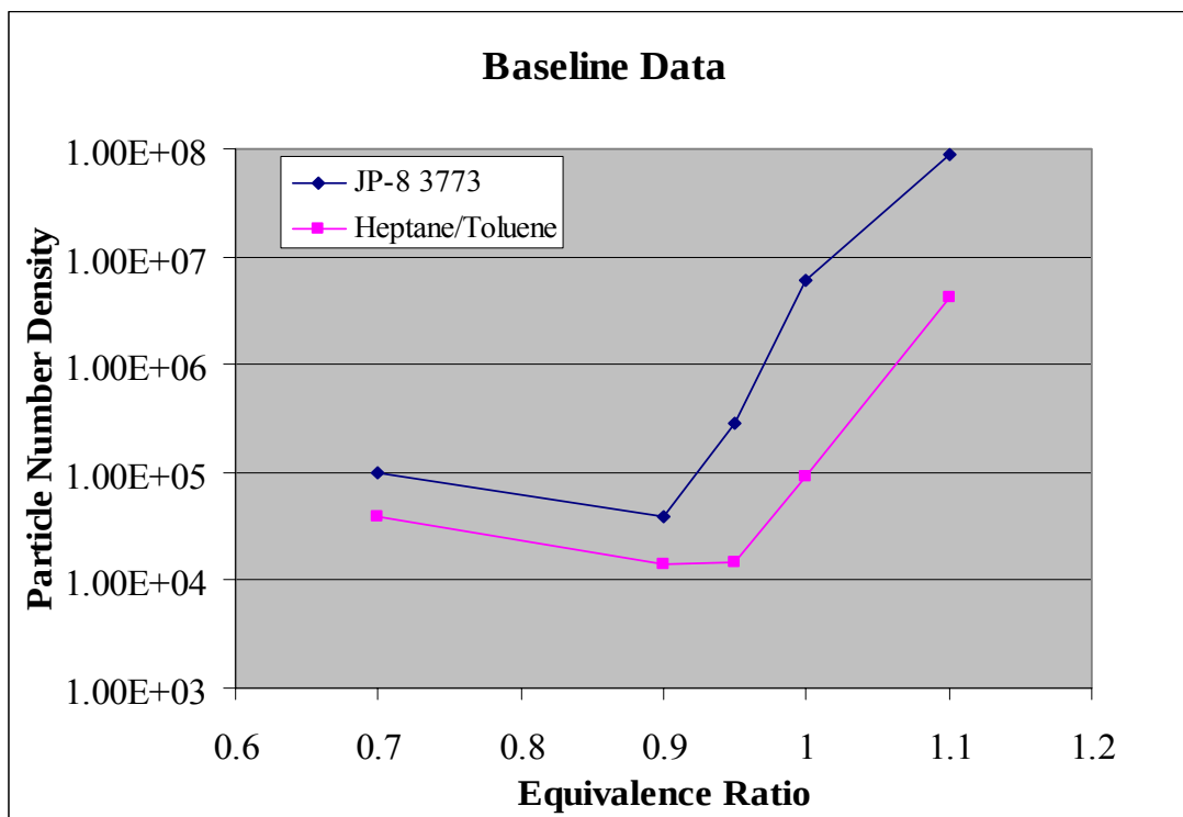
Figure 3.5.7-1. Particle Number Density as a Function of Equivalence Ratio for JP-8 3773 and Heptane/Toluene (80/20).
