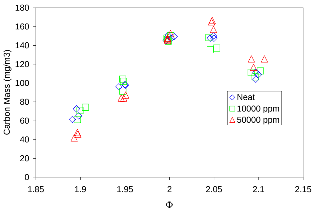
Figure 3.4.3-1. Total Carbon Particulate Mass vs \phi for Pyridine Additive Cases.
