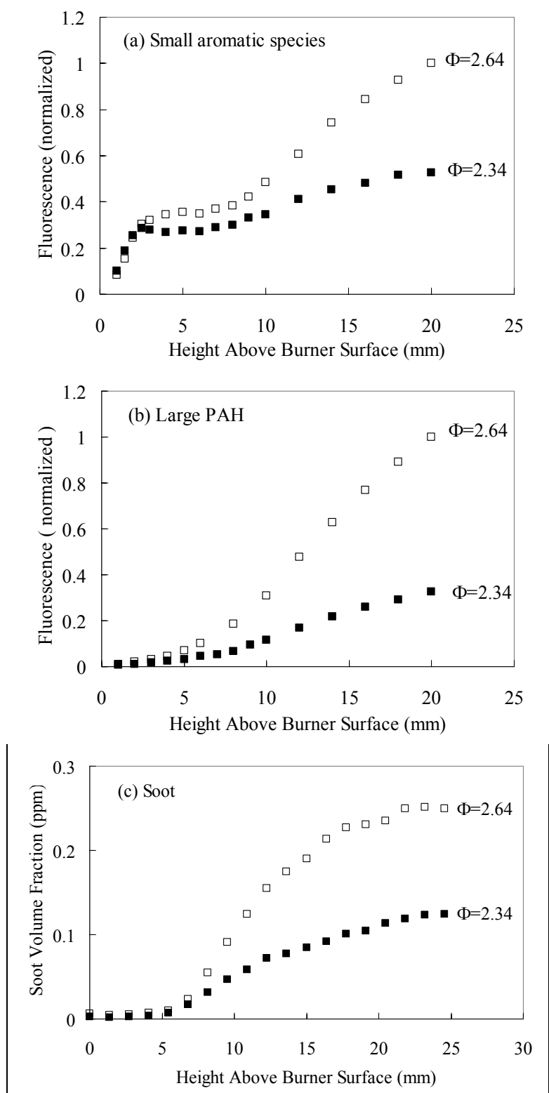
Figure 3.1.5-2 (a) Small Aromatic Species, (b) Large PAH, and (c) Soot for Ethylene/Air Flames. (Note that the PAH data are normalized by the maximum signal observed at \Phi=2.64 ).
