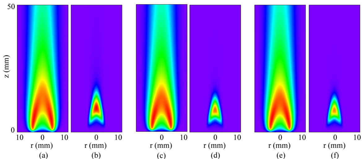
Figure 3.5.8-2. Effect of TMP on Propane Jet Diffusion Flame. Distributions of (a) temperature and (b) soot volume fraction for base flame with 0% TMP, (c) and (d) for the flame with 0.1% TMP, and (e) and (f) are for the flame with 1% TMP.
