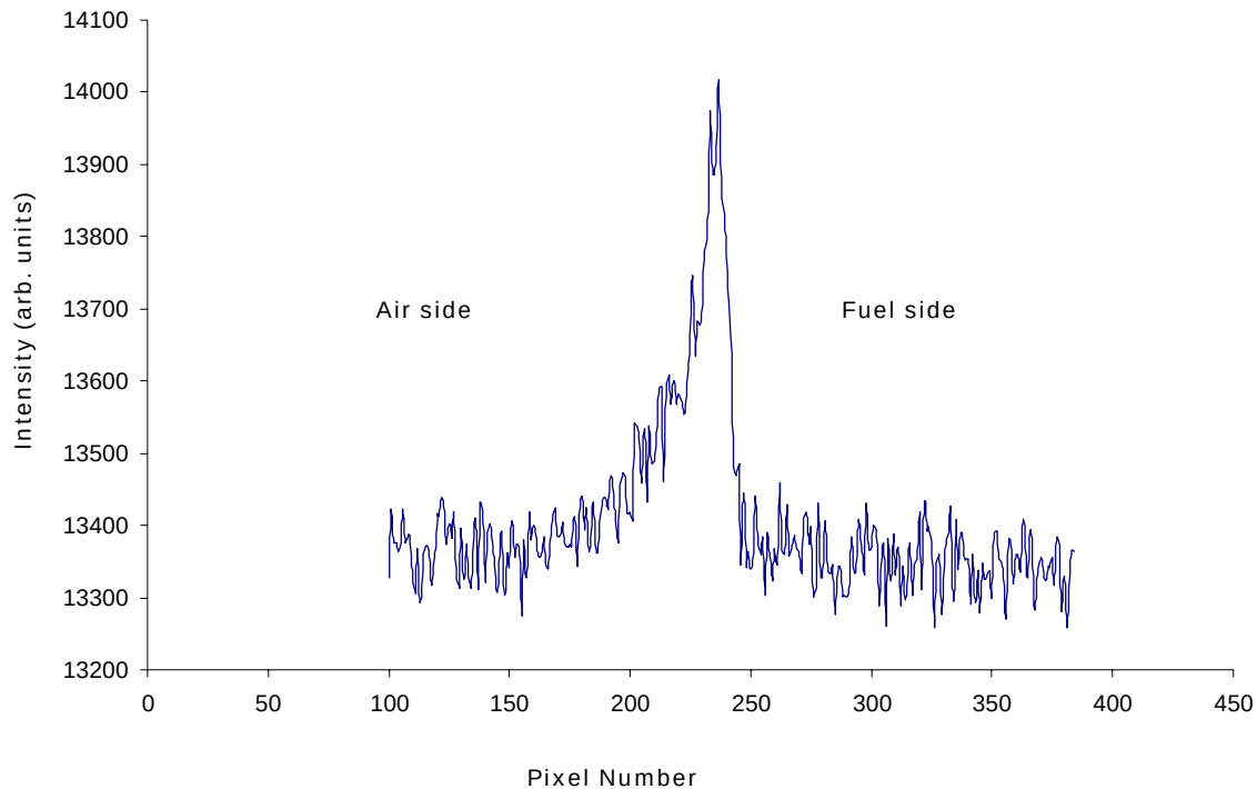
Figure 3.2.5-2. Pixel Intensities Along the Burner Centerline of the PLII Image of a Heptane/Air Opposed Flow Flame.
