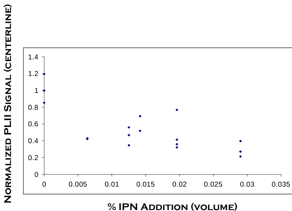
Figure 3.2.5-7. PLII Signal (peak centerline) vs IPN Addition to the Fuel Stream of Opposed Flow Heptane/Air Flames.
