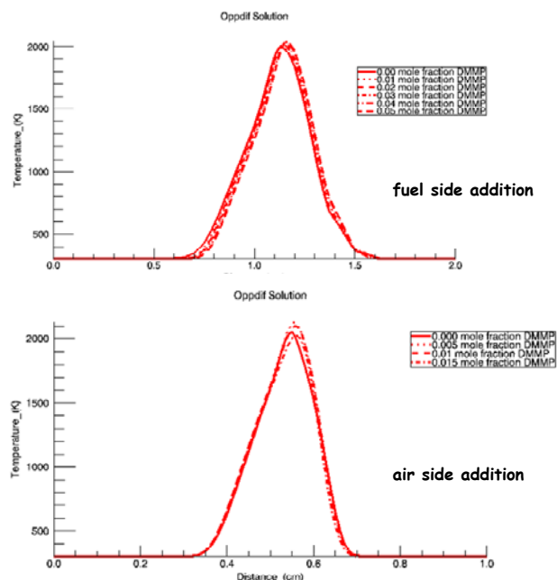
Figure 3.5.6-7. Calculated Temperature vs Flame Position (centerline) for Fuel and Oxidizer Side Addition to Ethylene/Air Opposed Flow Flames.
