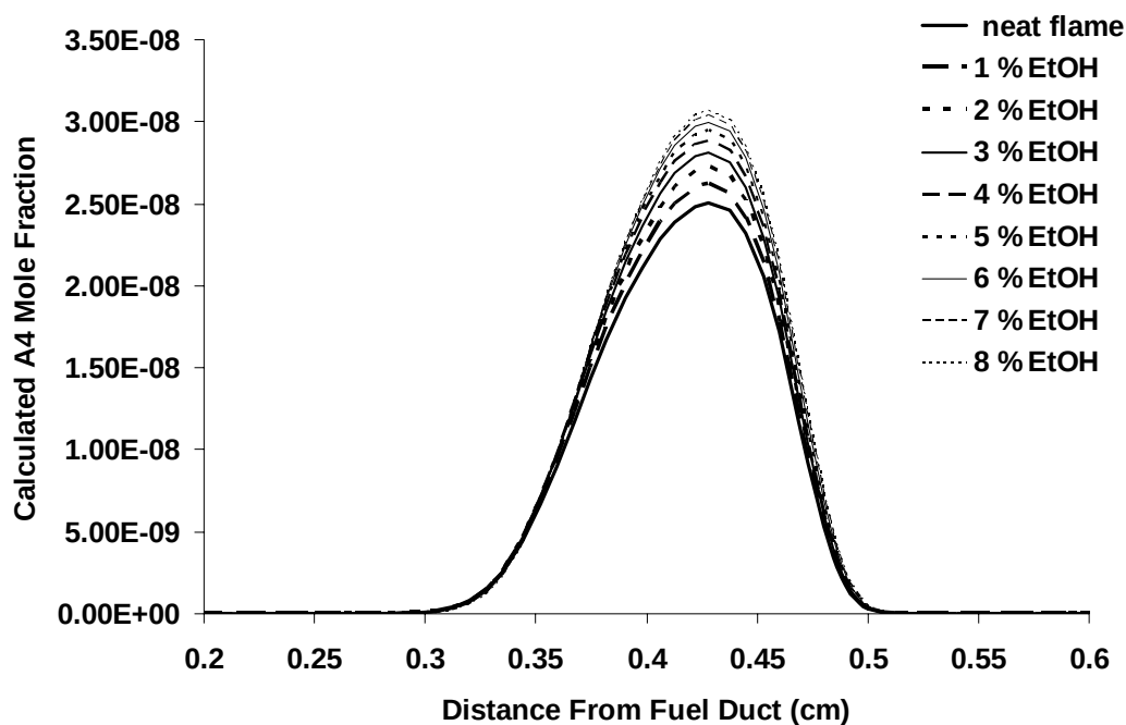
Figure 3.1-6-12. Calculated A4 Mole Fraction Profile for Increasing Amounts of Ethanol Vapor Added to the Fuel Stream.
