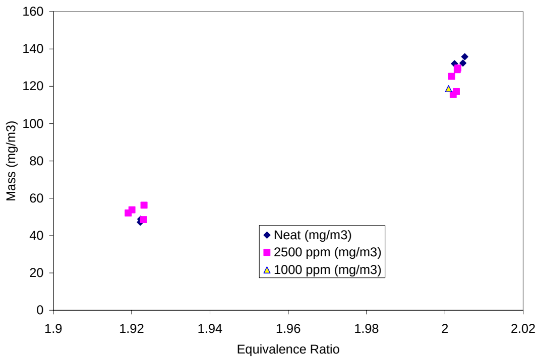
Figure 3.5.3-3. The Effect of Diethyl Allyl Phosphate on the Carbonaceous Carbon Mass from Samples in the WSR.
