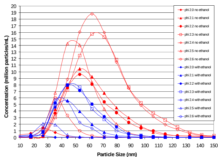
Figure 3.1.3-13. Experimental Particle Size Distribution for Stirred Reactor.
