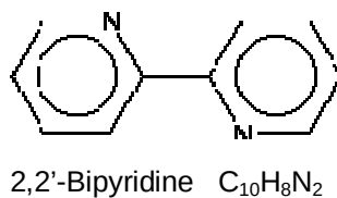
Figure 3.2.2-4. Molecular Structure and Formulae of Semivolatile Nitrogenated Compounds Detected from Nitromethane, NO_2 and Pyridine Additives at 21 atm.
