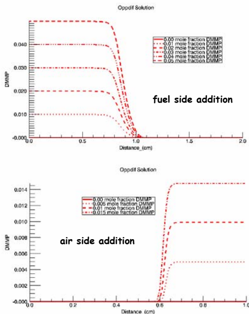
Figure 3.5.6-6. DMMP Calculated Concentration vs. Flame Position (centerline) for Fuel and Oxidizer Side Addition to Ethylene/Air Opposed Flow Flames.
