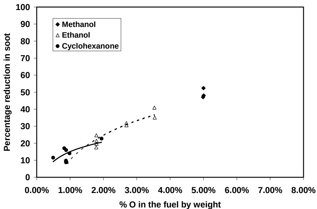
Figure 3.1.8-2. Effect of Oxygenated Additives on Soot Formation with JP-8.
