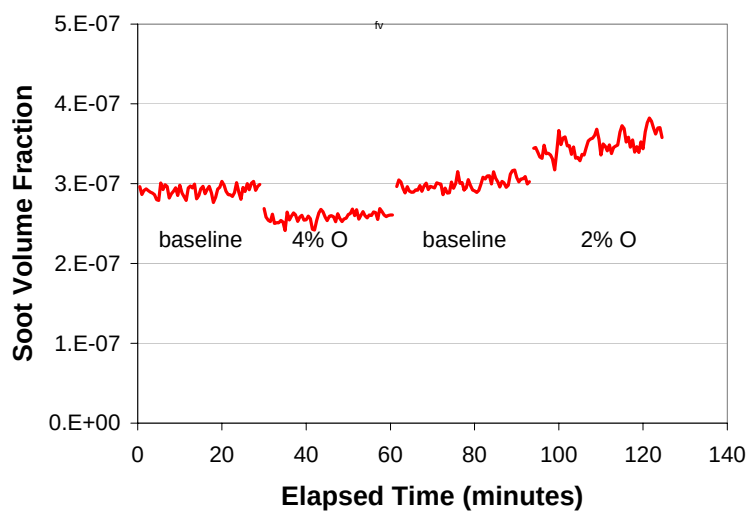
Figure 3.2.4-2. Time Trace Confirming Concentration Effect with Nitropropane.
