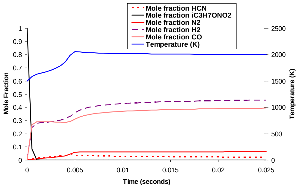
Figure 3.2.5-10. Calculated Thermal Decomposition of Neat Isopropyl Nitrate at 1500 K in a Closed Homogeneous Reactor. Major decomposition products are H_2 , CO, N_2 , HCN.
