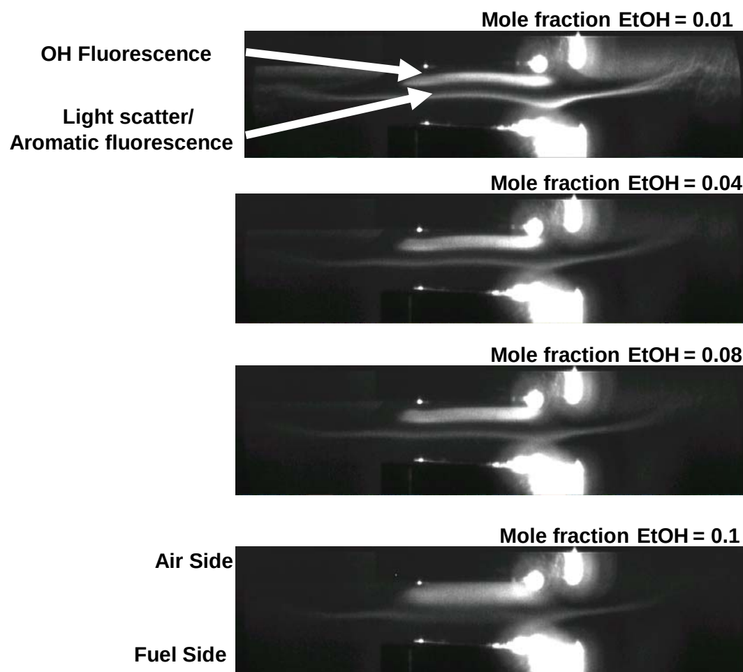
Figure 3.1.6-4. Images of OH PLIF and Light Scattering by Soot Particles as Increasing Amounts of Ethanol Vapor are Added to the Air Side. Note increasing width of OH region (upper feature) and decreasing intensity of light scatter from particles (lower feature).
