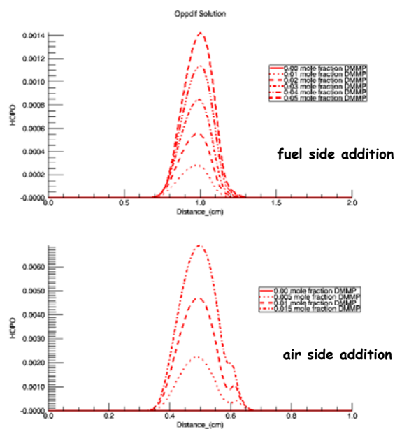
Figure 3.5.6-12. Calculated HOPO Concentration vs Flame Position (centerline) for Fuel and Oxidizer Side Addition to Ethylene/Air Opposed Flow Flames.
