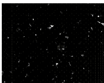
nitroethane
