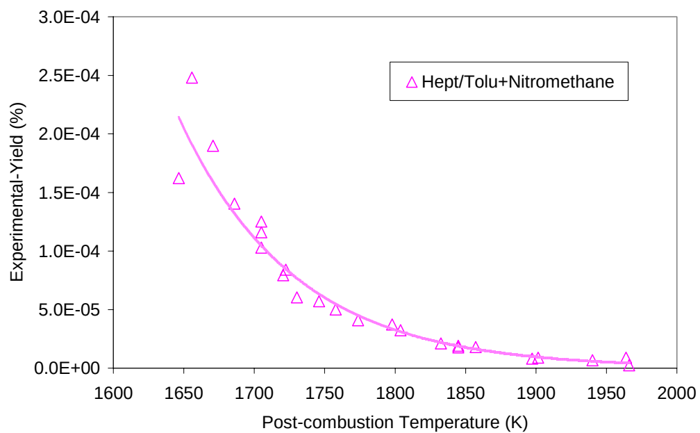
Figure 3.2.2-5. Benzonitrile Yield from Heptane/Toluene + Nitromethane at 21 atm.
