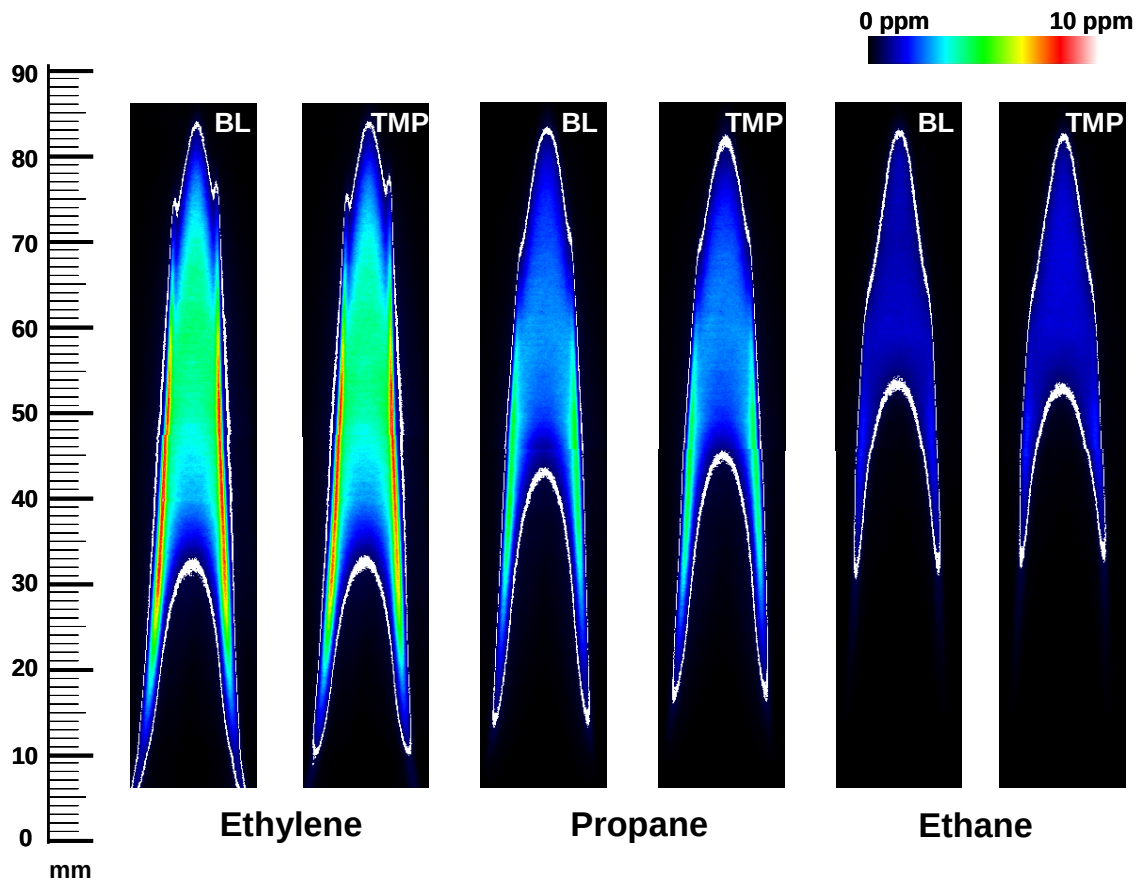
Figure 3.5.5-1. Soot Volume Fraction Fields for Baseline and TMP Addition Flames of Ethylene, Propane and Ethane. Contour of fv=0.5 ppm shown in white line is superimposed on soot volume fraction fields.
