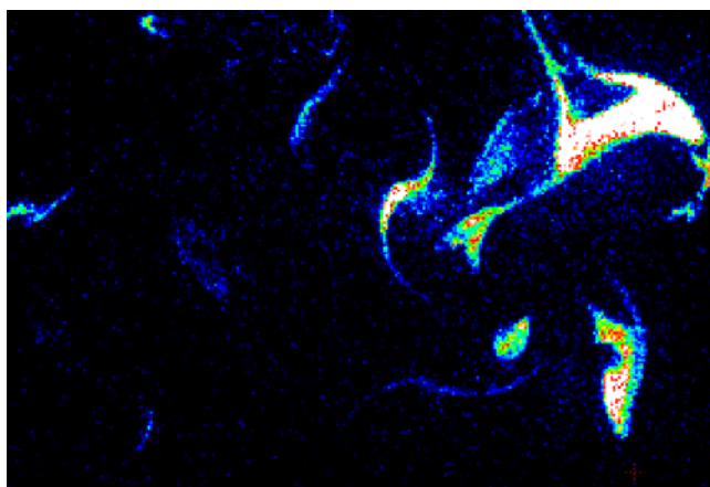
Figure 3.1.7-2. Sample Single Shot LII Image from Heptane Spray Flame.
