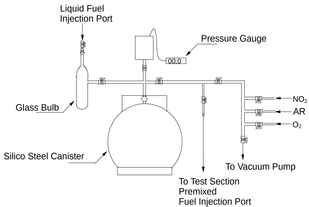
Figure 2.1.1-3. Sample Preparation Unit.
