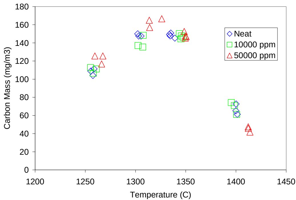
Figure 3.4.3-2. Total Carbon Particulate Mass vs WSR Temperature for Pyridine Additive Cases.
