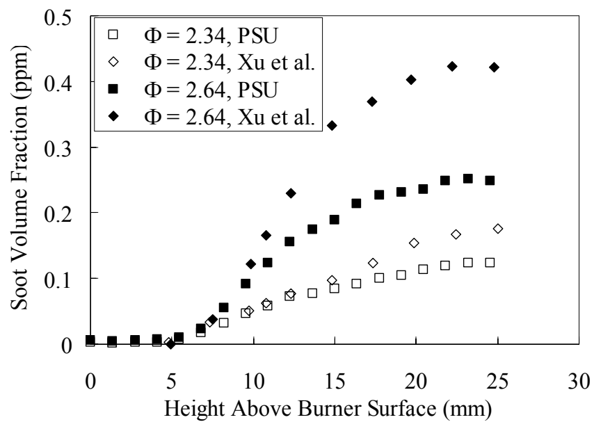
Figure 3.1.5-3. Comparison of Soot Volume Fraction Measurement Results to Those of Xu et al [1997].
