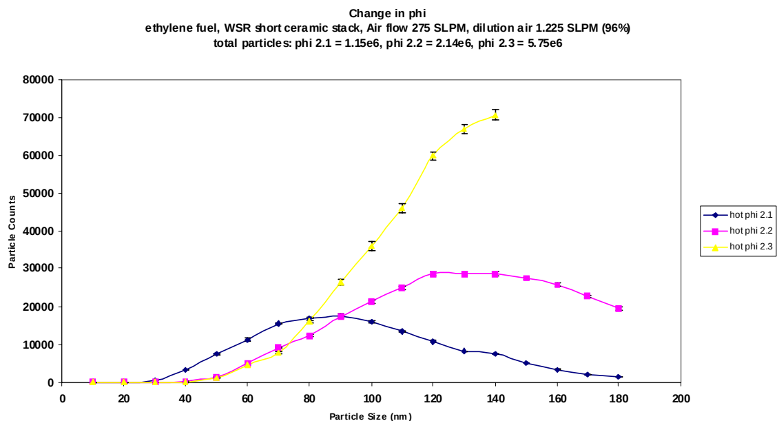
Figure 2.1.2-10. Particle Size Distribution for WSR on Ethylene Fuel vs Equivalence Ratio.
