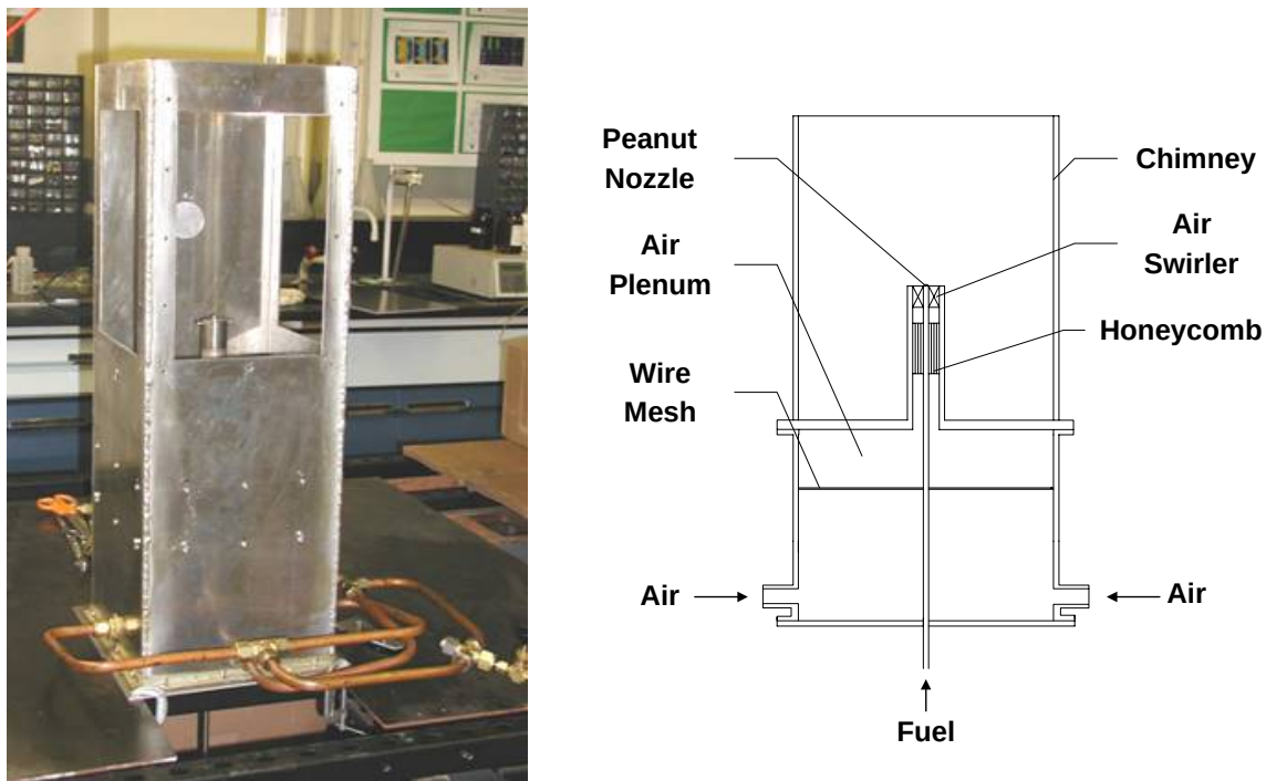
Figure 2.1.7-1. Image and Schematic of Turbulent Spray Burner.
