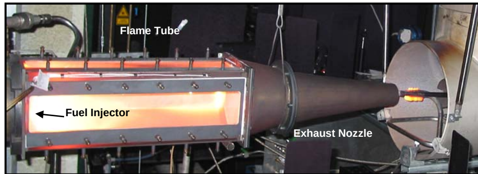
Figure 2.1.9-1. Swirl-Stabilized Atmospheric Pressure Research Combustor.
