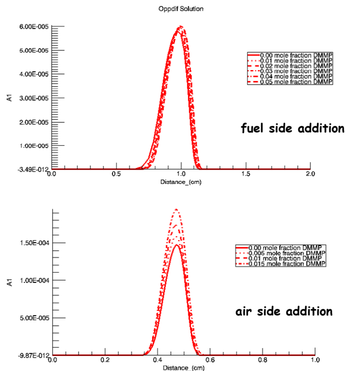
Figure 3.5.6-13. Calculated A1 (benzene) Concentration vs Flame Position (centerline) for Fuel and Oxidizer Side Addition to Ethylene/Air Opposed Flow Flames.
