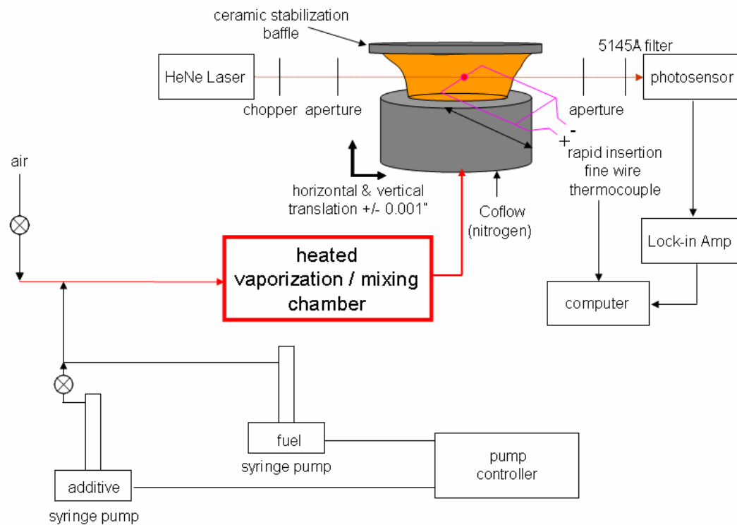
Figure 2.1.4-7. Experimental Setup for the Heptane Flame Experiments.
