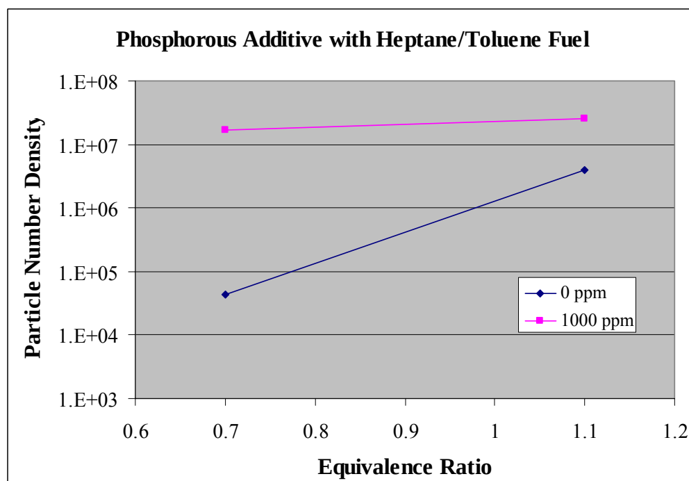
Figure 3.5.7-2. Particle Number Density Changes for Diethyl Allyl Phosphate Added to 80/20 Heptane/Toluene at 1000 ppm.
