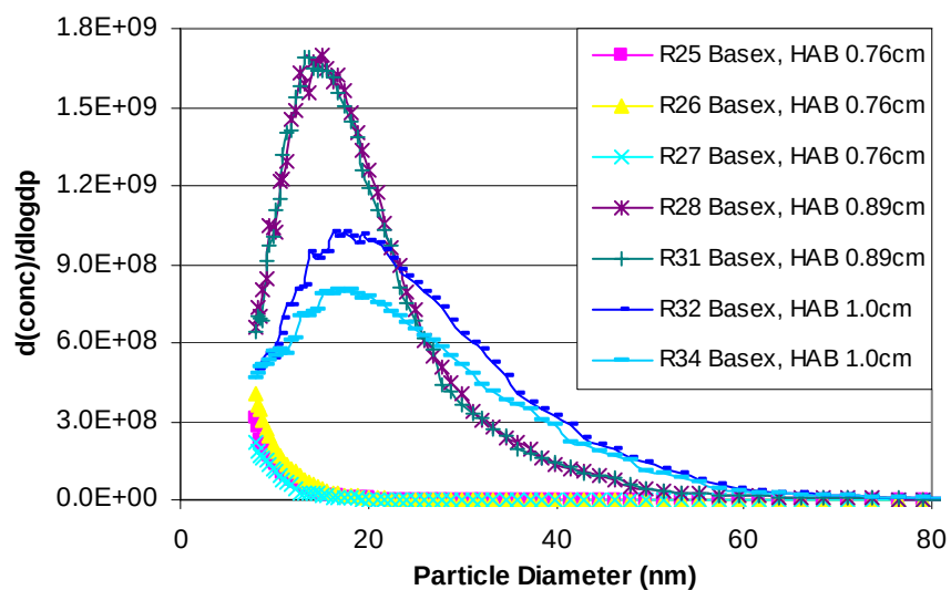
Figure 3.2.4-4. Particle Size Distributions in Diluted Samples.
