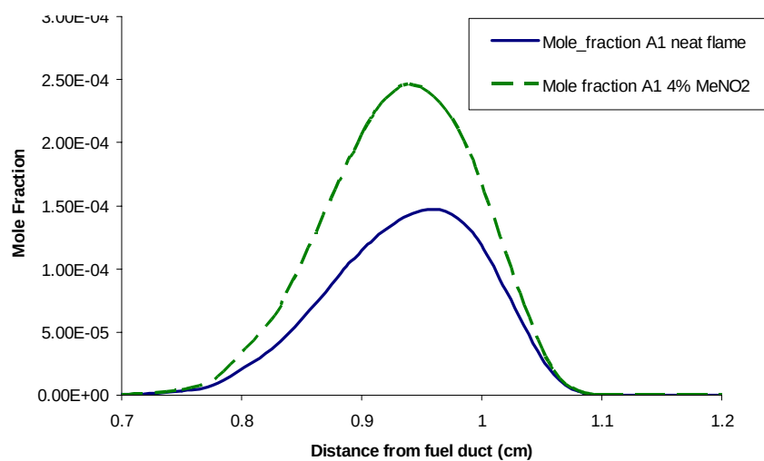
Figure 3.2.5-5 Calculated A1 Concentrations for Neat Ethylene/Air Flames and Ethylene/Air Flames to which 4 Mole Percent Nitromethane has been Added to the Fuel Side.
