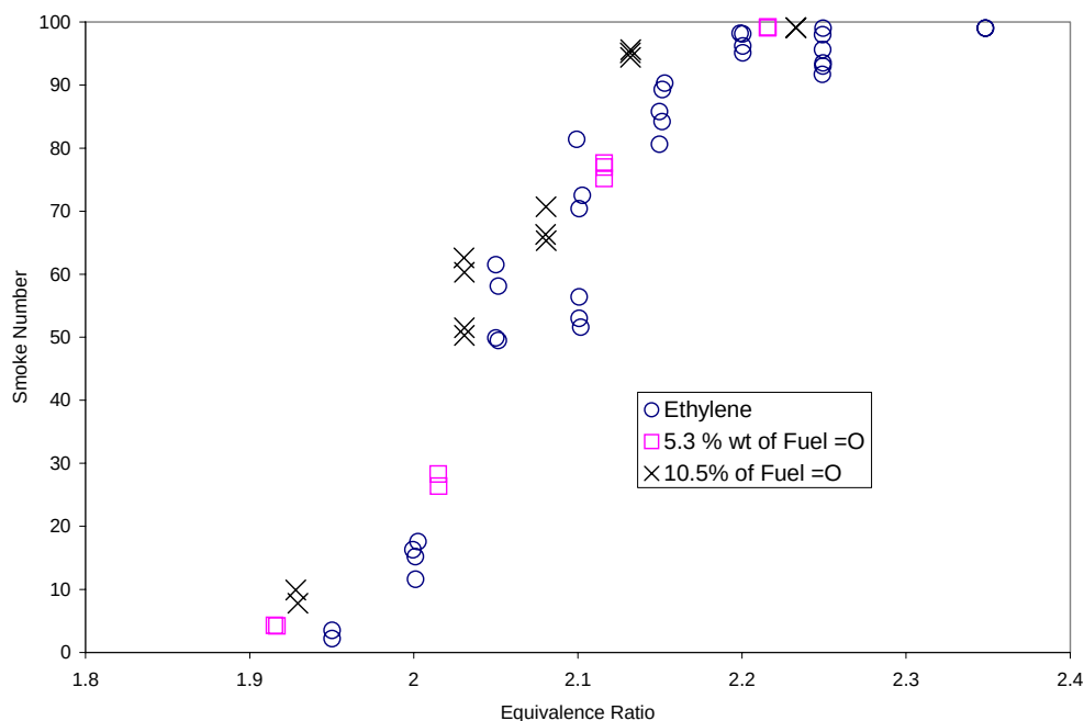
Figure 3.1.3-1. Smoke Number vs Equivalence Ratio for Ethanol Additive Experiments.
