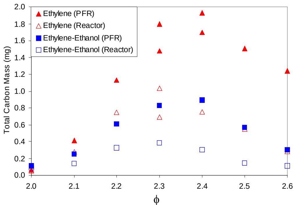
Figure 3.1.3-6. Total Carbon Measurements Results for Neat Ethylene and Ethanol Additives (Silicon Carbide Reactor).
