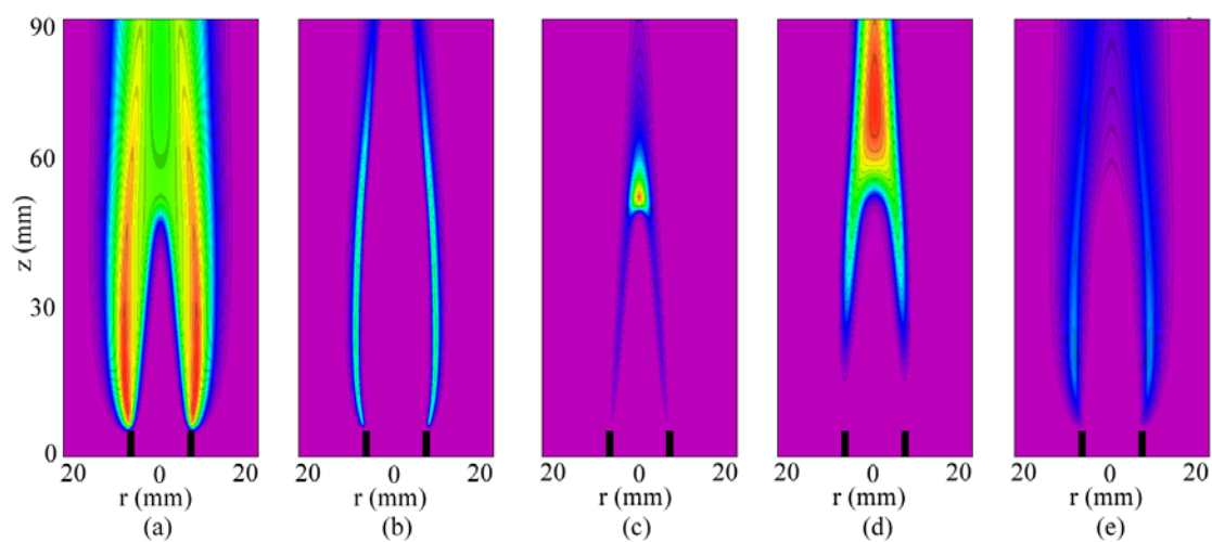
Figure 3.5.8-8. Heptane Premixed Flame with 1.0% TMP. Mixture of heptane and air with \phi = 2.0 is issued from a 13 mm tube at 1.0 m/s. Distributions of (a) temperature, (b) OH, (c) benzene, (d) soot volume fraction, and (e) NO.
