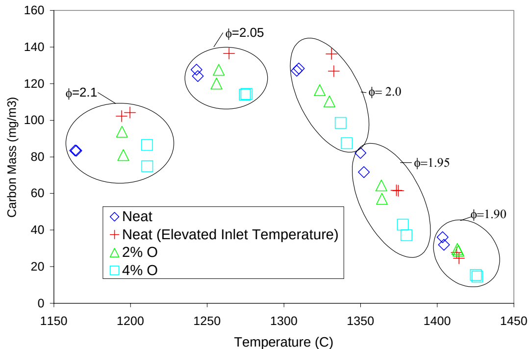
Figure 3.2.3-1. Total Carbon Mass for Nitromethane Additive Cases Studied in the WSR.
