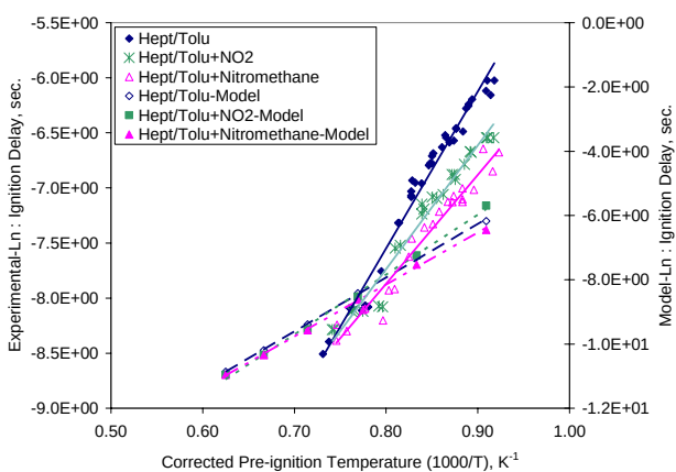
Figure 3.3.2-4. Ignition Delay from Combustion of n-Heptane/Toluene + NO x Additives at 21 atm.
