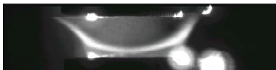
Figure 3.1.6-15. Normal and PLIF Images of the Heptane/Air Diffusion Flame.
