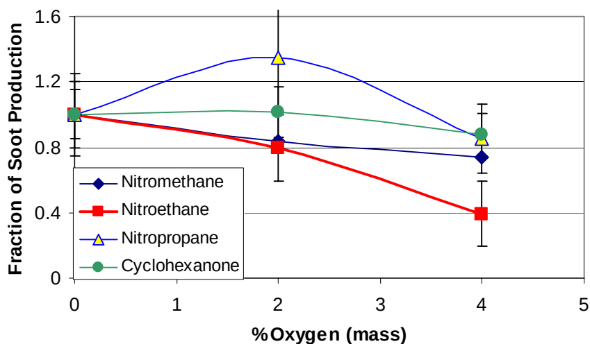
Figure 3.2.4-1. Relative Soot Production in Laminar Premixed Flame.
