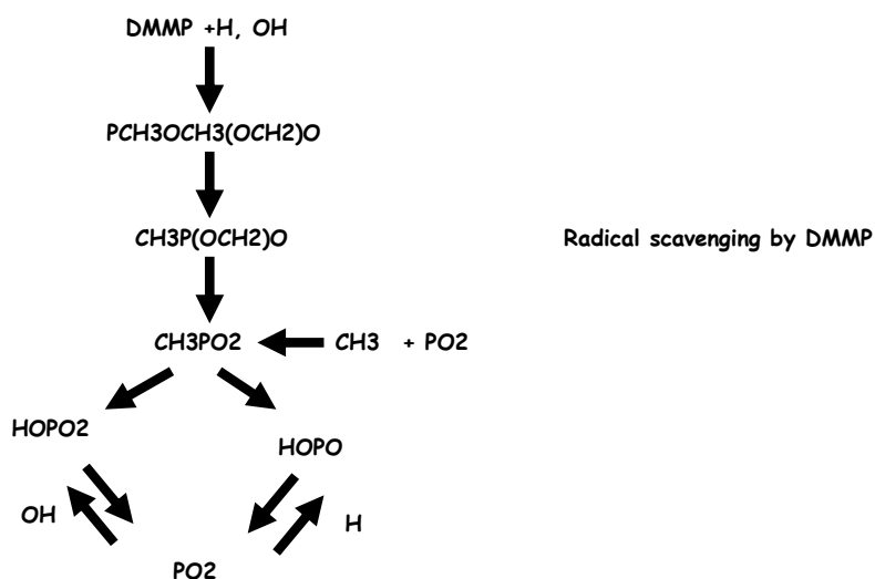
Figure 3.5.6-14. The Radical Scavenging Mechanism Believed to be Responsible for the Flame Suppression Effectiveness of DMMP.
