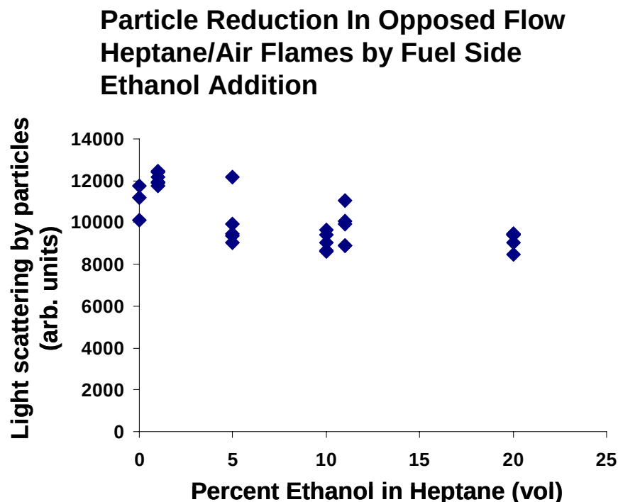
Figure 3.1.6-16. Light Scattering by Particles vs Fuel Side Ethanol Addition for Heptane/Air Opposed Flow Flames.
