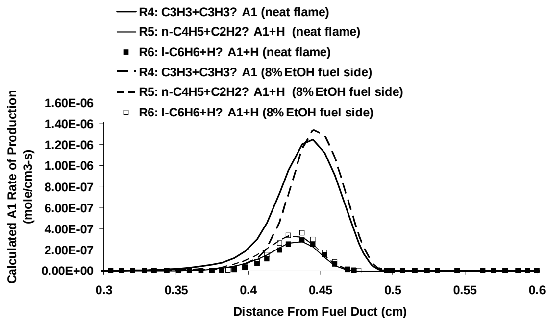
Figure 3.1.6-14. Rates of Production of A1 by the Three Most Important Reactions Contributing to A1 Production. Note the overall enhancement of rates of reactions that do not involve propargyl. The net rate of A1 production by propargyl combination is only slightly affected by the ethanol addition.
