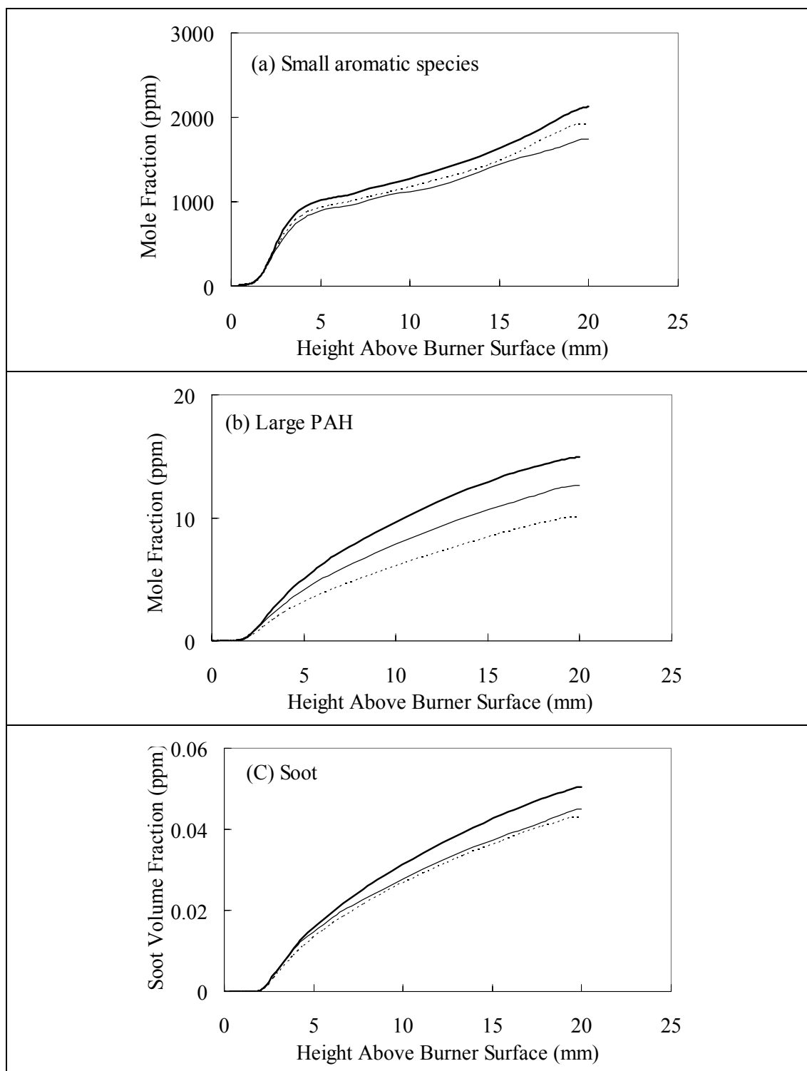
Figure 3.1.5-8. Effect of Temperature on (a) Small Aromatic Species, (b) Large PAH, and (c) Soot Predicted by Model at \Phi=2.34 . (Thick solid lines represent baseline cases, thin solid lines represent 5% oxygen cases with measured temperature profiles, and dashed lines represent 5% oxygen cases with same temperature profiles as the baseline cases.)
