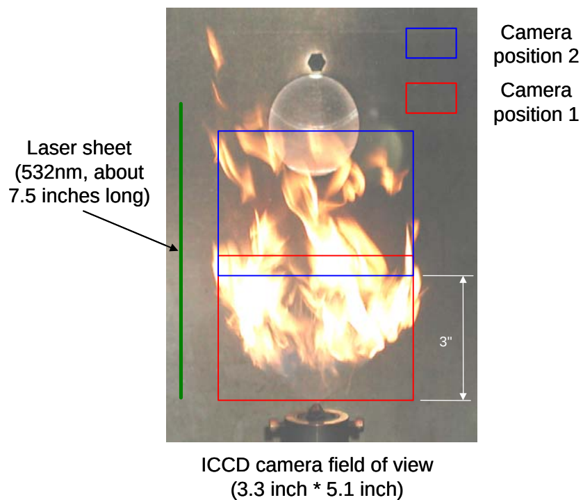
Figure 3.1.7-4. Overlapping of Fields of View Required to Cover Full Extent of the Flame.
