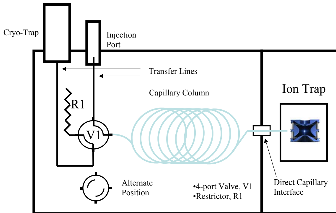
Figure 2.1.2-9. Plumbing Diagram of Saturn GC/MS Subsystem of PMCMS in the Original Oven Configuration.
