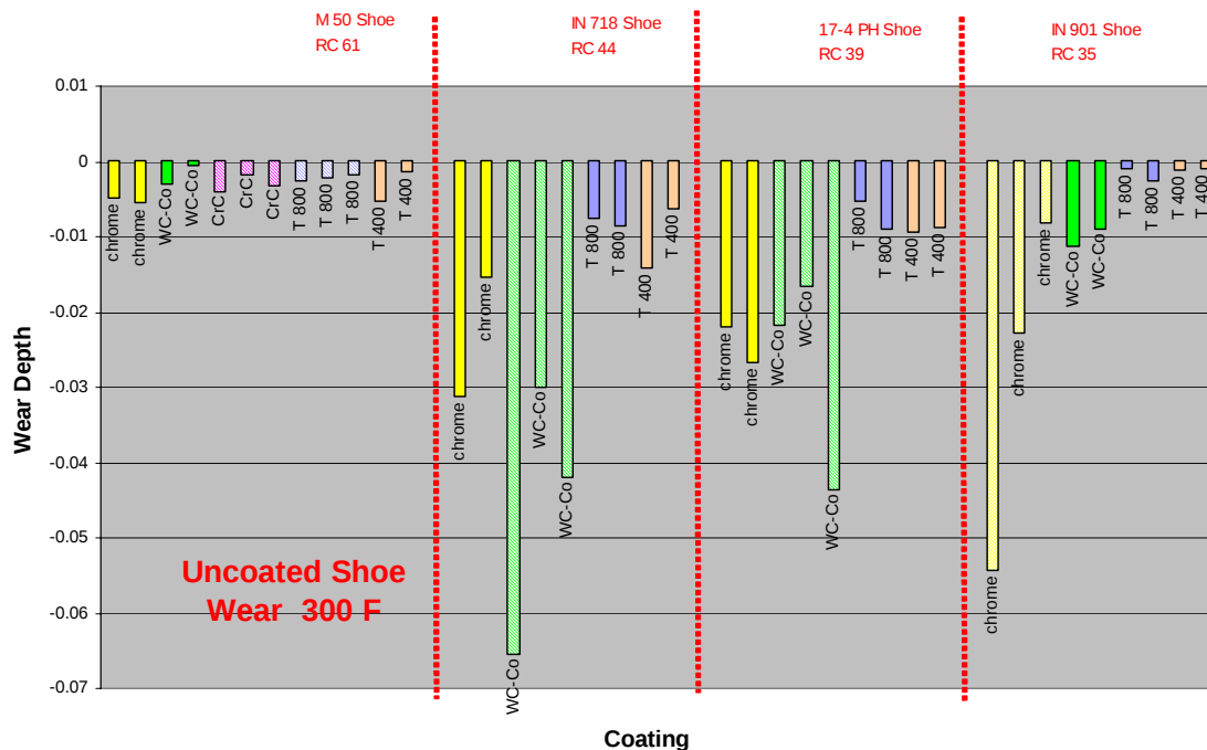
Figure 14. Wear Coefficients (plotted as average wear depth) for Shoes Sliding Against the Indicated Coatings for Testing at 300°F.
