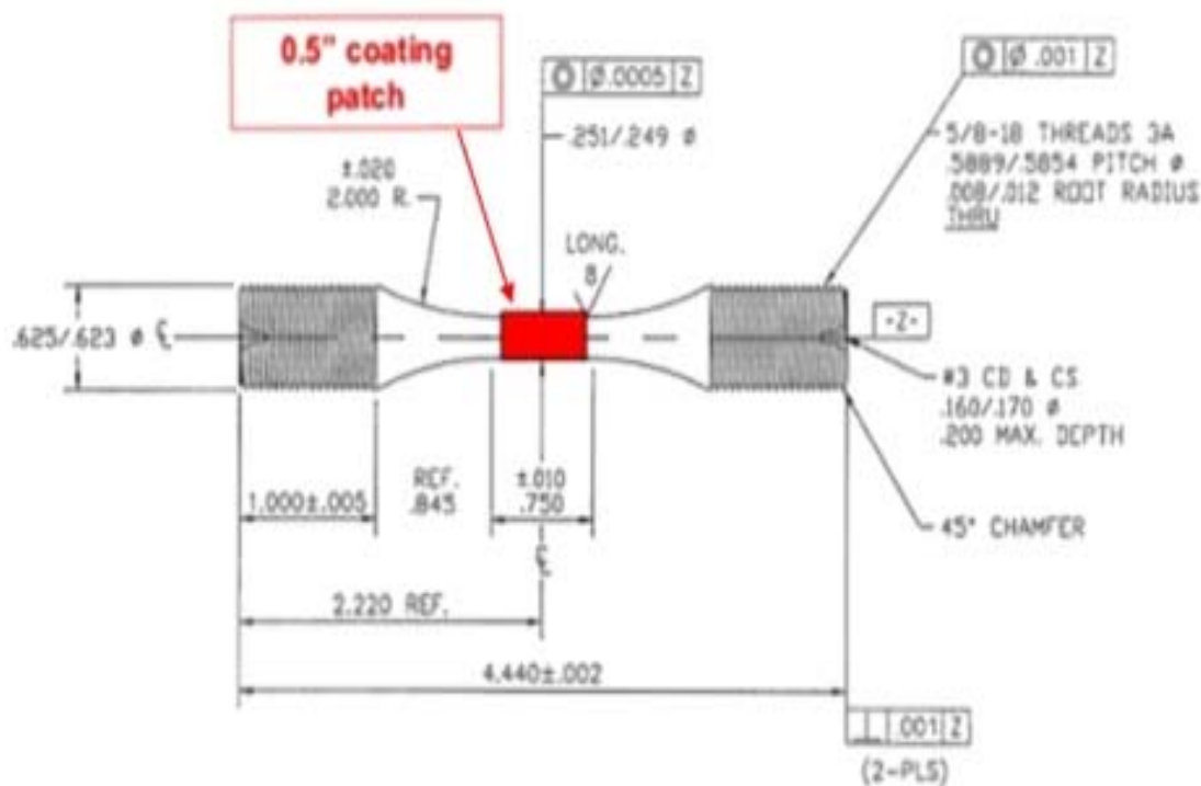
Figure 6. Schematic of Smooth-Gage Fatigue Specimen Showing Location of Coating Patch.
