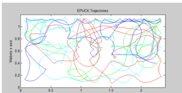
Figure 2: Agent Trajectories.
