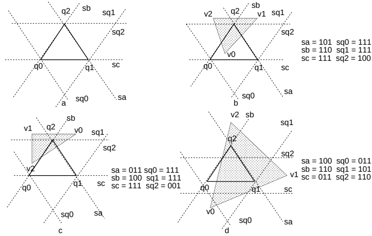
Figure 18: Triangle intersection test a) Quadtree q0, q1, q2 . Triangle vertices are tested against lines shown. Lines are labeled with corresponding bit test variables, sa, sb, sc, sq0, sq1, sq2 . b) (sa \& sb \& sc) = 100 , vertex v0 is interior and triangle is accepted. c) Edge v0v1 is trivially rejected because of test sq1 . Likewise for v1v2 for test sb . After parametric intersection test, triangle is accepted. d) Edge v0v1 intersects below the range on edge q1q2 . Edge v1v2 intersects above the range on edge q1q2 . Therefore the triangle is accepted without having to do further testing.
