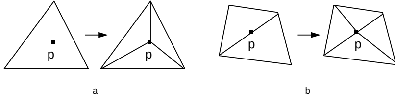
Figure 3: Point Insertion: a) Sample p falls inside existing triangle: 3 new triangles are created. b) Sample p falls on edge: 4 new triangles are created.
