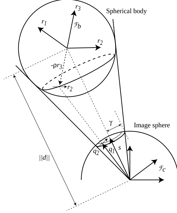
Figure 1: Projection of a spherical body with a feature point on it to the image-sphere. The image-plane measurement is given by y = (Q, \lambda, \mathbf{s}) = c(H) .
