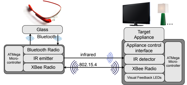
Figure 6. In our system architecture, selection is initiated through infrared but confirmed over 802.15.4. This permits wearers to move their head freely after connecting to an appliance. In the research prototype, users have to carry an additional microcontroller board that marshals messages between Glass' Bluetooth radio and IR/802.15.4, but our custom hardware could also be integrated into the wearable device.
