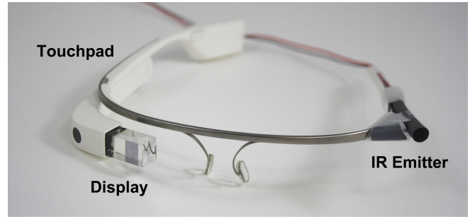
Figure 5. Our augmented Glass prototype has a frame-mounted infrared emitter.
