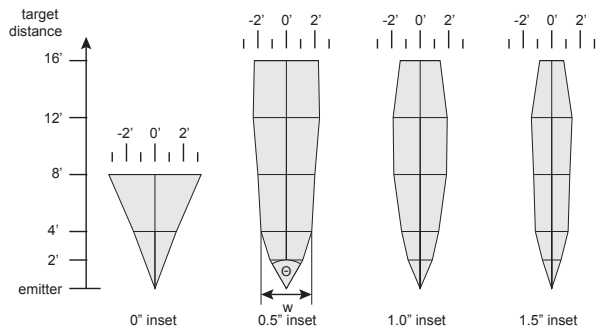
Figure 7. Different IR configurations suggest usable beam widths of 2 to 4 feet and distances up to 16 feet
