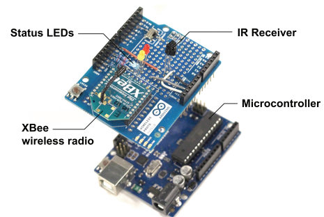
Figure 9. An example node from the targeting study — we constructed 10 such nodes — each mounted in a box.
