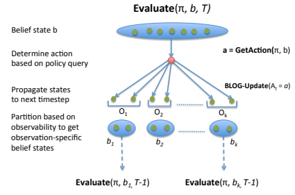
Figure 2: Illustration of one iteration of Alg. 1
