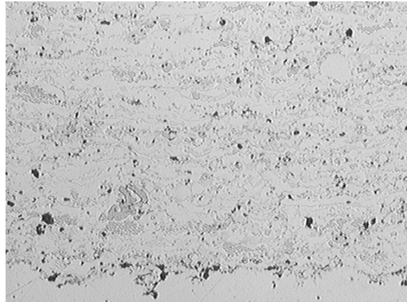
Fig. 19: Diamalloy 2002; with F-100 (8 H 2 )
