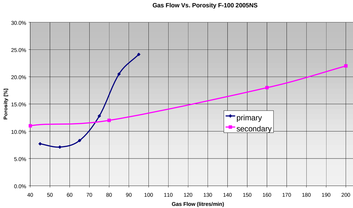
Figure 2-9 Effect of primary and secondary gas flow on porosity - Diamalloy 2005NS WC-17Co from F-100 gun. Primary gas flow (Ar) 45 lm-1 when varying secondary gas. Secondary gas (He) held at 10 lm-1 when varying primary gas.
