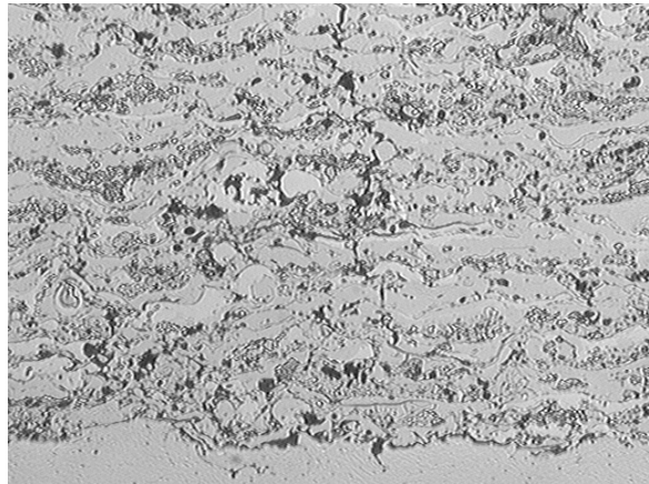
Fig. 13: Metco 439NS-2; with F-100 (8 H 2 )
