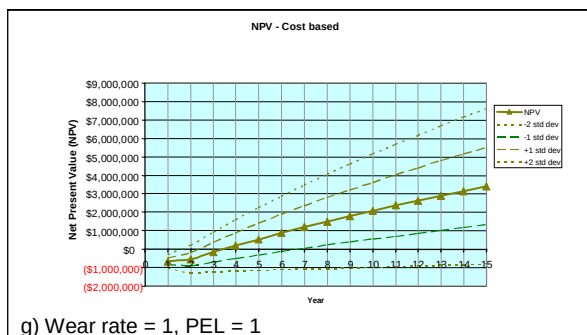
Figure 5-1. Simple NPV calculations for low and high wear rate, low and high PEL. Small ID gun (top) and large ID gun (bottom).
