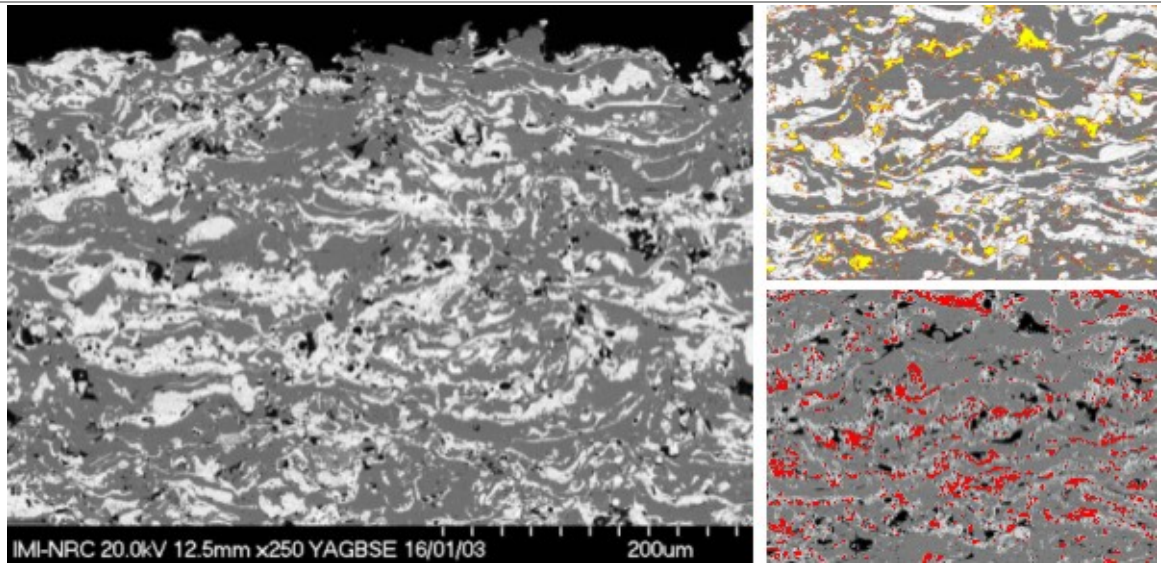
Figure 4-9 Cross sectional microstructure of WC-Co self fluxing (Ni 988). Right – map of porosity on a typical area (yellow), WC (red)
