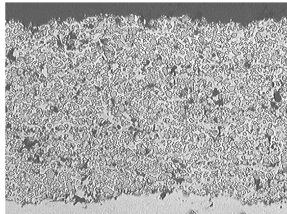
Fig. 6: Diamalloy 2005, sprayed with F-100 Run number 91201-1, 200x unetched Porosity 11.2% Macrohardness (15N) 84.3 Microhardness (HV 300 ) 847 average
