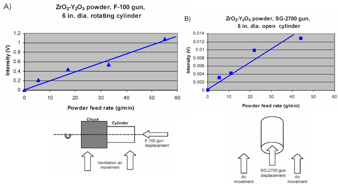
Figure 5-4. Optical signals for two different gas feed geometries. A) F100 gun with gas flow across outside of rotating cylinder; B) SG-2700 gun with gas flow through stationary cylinder. Note intensity scales.
