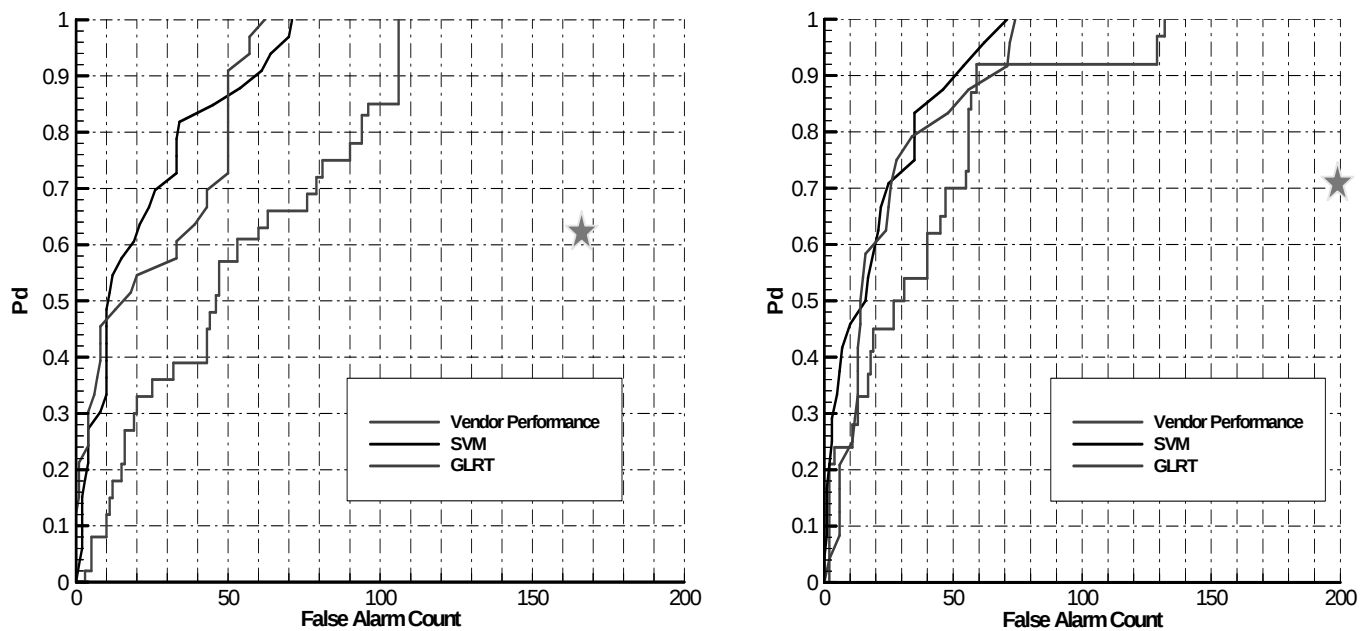
Figure 12. ROC Performance for JPG V, GEM3 data scored blind. Left panel, Area 1 results on 178 anomalies, 33 UXO. Right panel, Area 2 results on 236 anomalies, 24 UXO.
