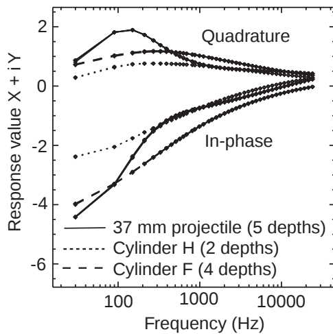
Figure 8. EMI response from the 37mm projectile shows strong differences from response of similarly sized cylinders. This difference is consistent over a range of depths, and it is about an order of magnitude larger than any competing effect.
