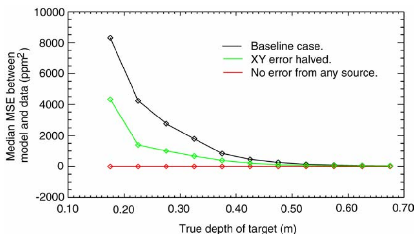
Figure 10. Effect of horizontal x - y position error with target depth.
