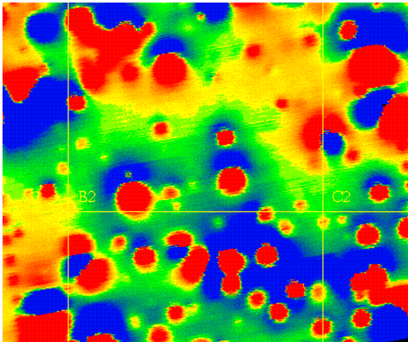
Figure 44: Magnetometer data from a section of the Blind Test Grid. Image scale \pm 25 gamma.
