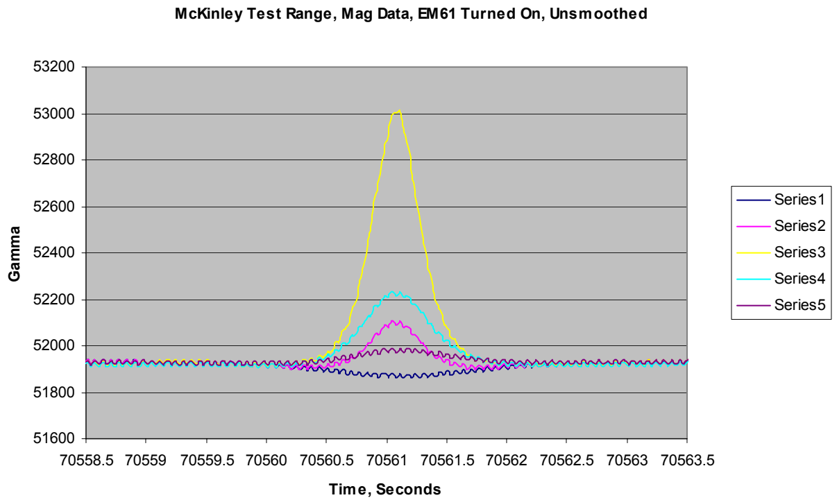
Figure 29: Magnetometer Data with EM61s Turned On
