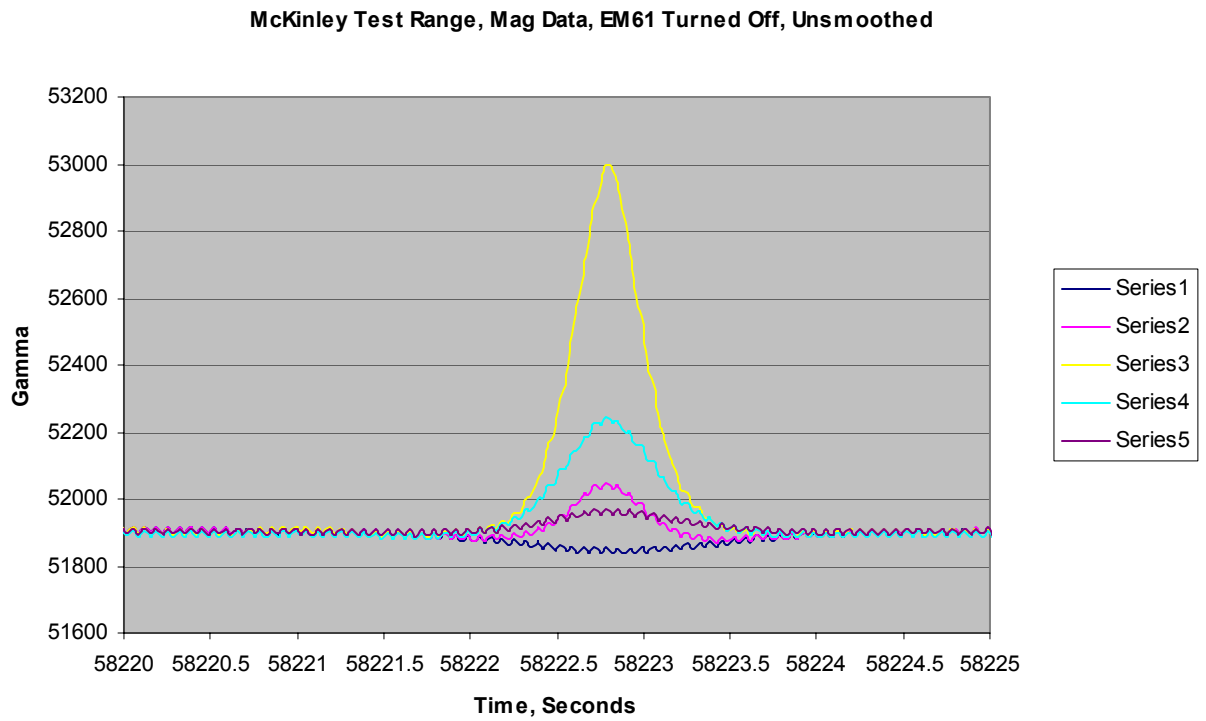
Figure 28: Magnetometer Data with EM61s Turned Off
