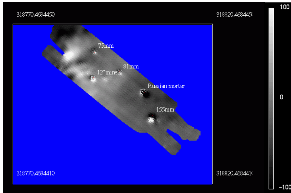
Figure 19: Magnetometer data acquired during integration and testing (magnetometers while EM61 electronics are running). Image scale +/- 100 gamma.
