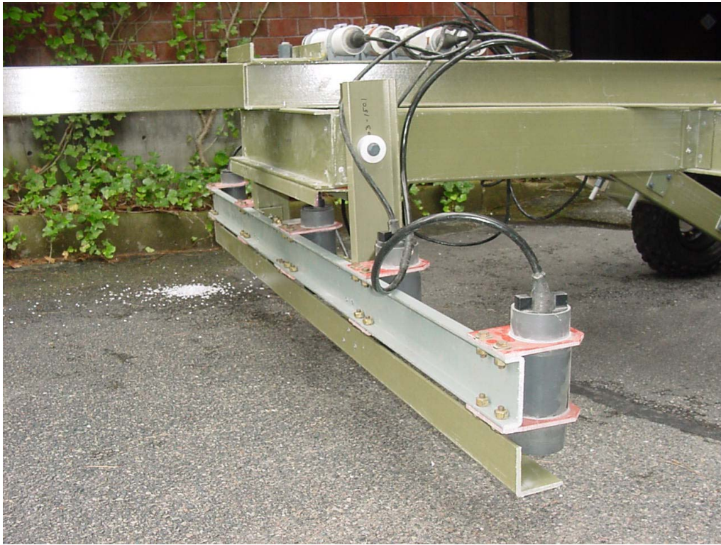
Figure 13: Five total field magnetometers spaced \frac{1}{2} meter apart mounted on swing-back boom.
