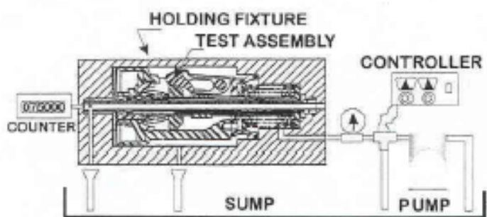
FIGURE 2 TEST SCHEMATIC
