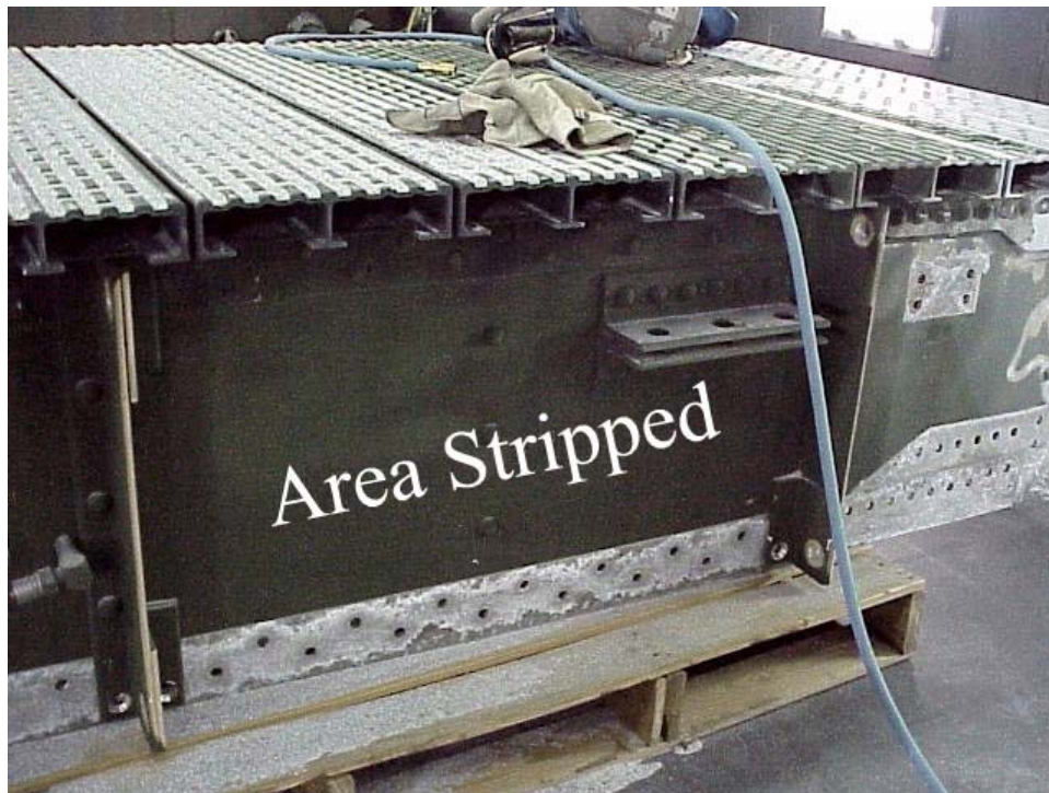
Figure 39 -- Area of 'Bridge' Section Stripped with Type III DMB Process at Albany MCLB
