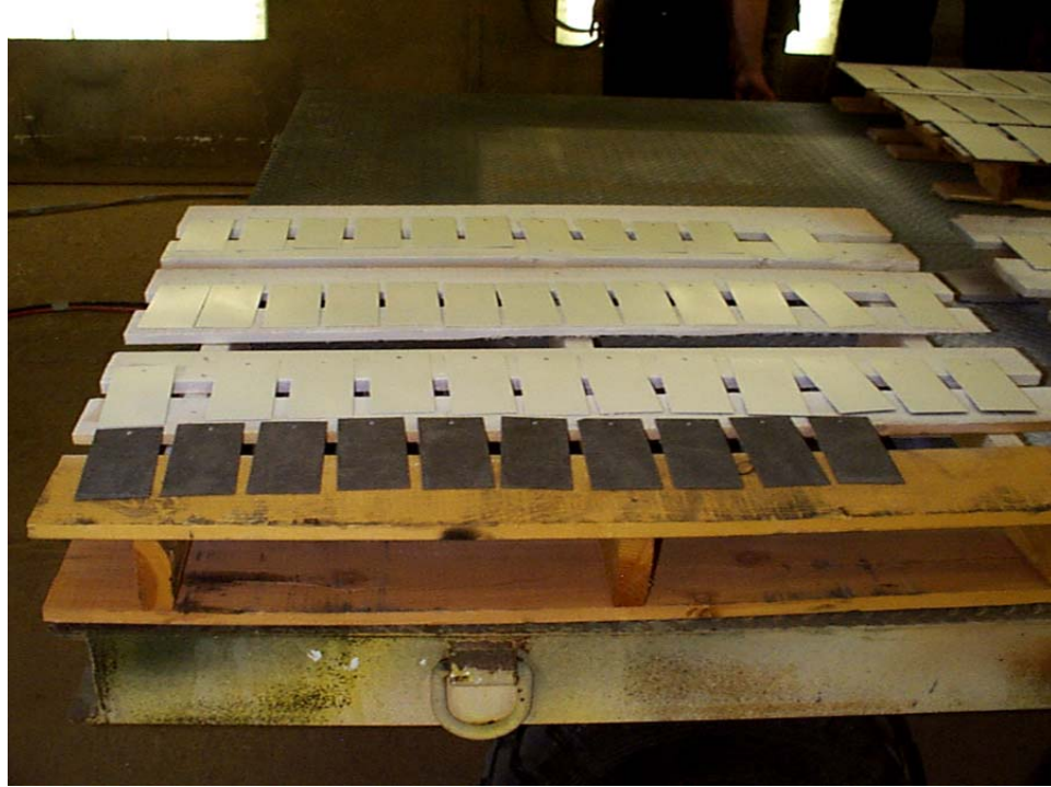
Figure 1 -- Test Panels Before Application of WD CARC at MCB
