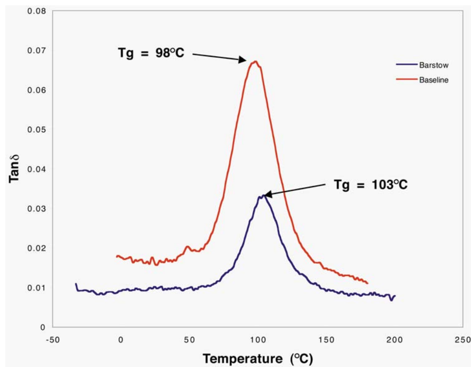
Figure 25 -- Determination of Glass Transition Temperature of Laboratory and Field Samples
