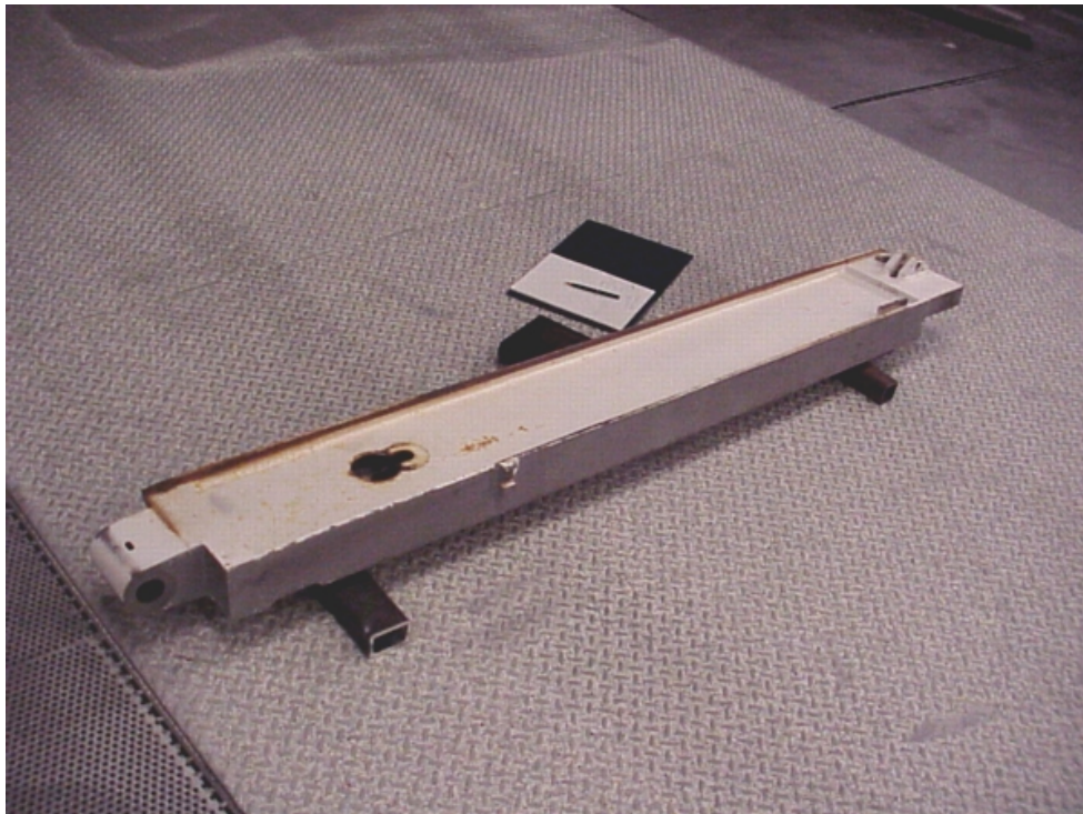
Figure 33 -- Beam Blasted in OO-ALC, Building 847 Blast Booth
