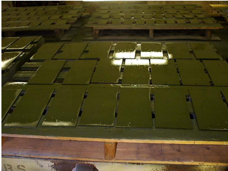
Figure 2 -- Test Panels with WD CARC Applied at MCB
