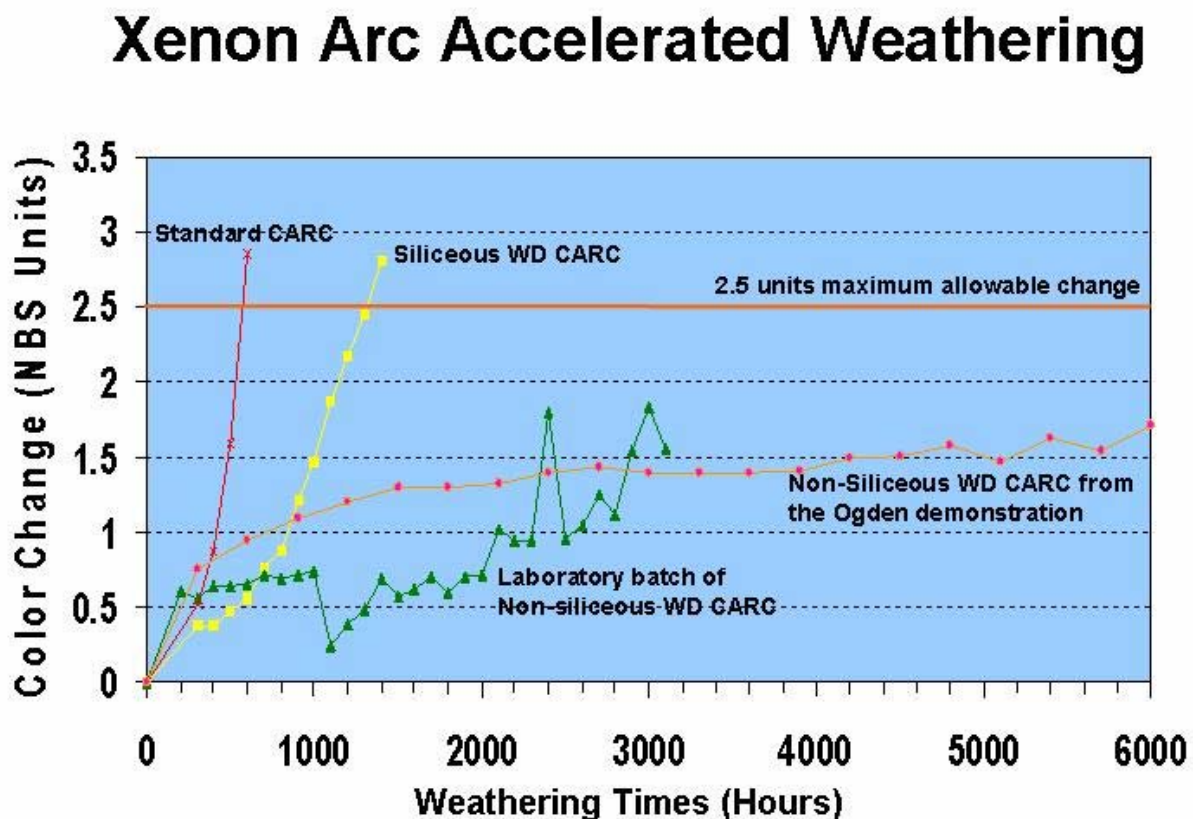
Figure 28 -- Accelerated Weathering Results for Ogden Demonstration
