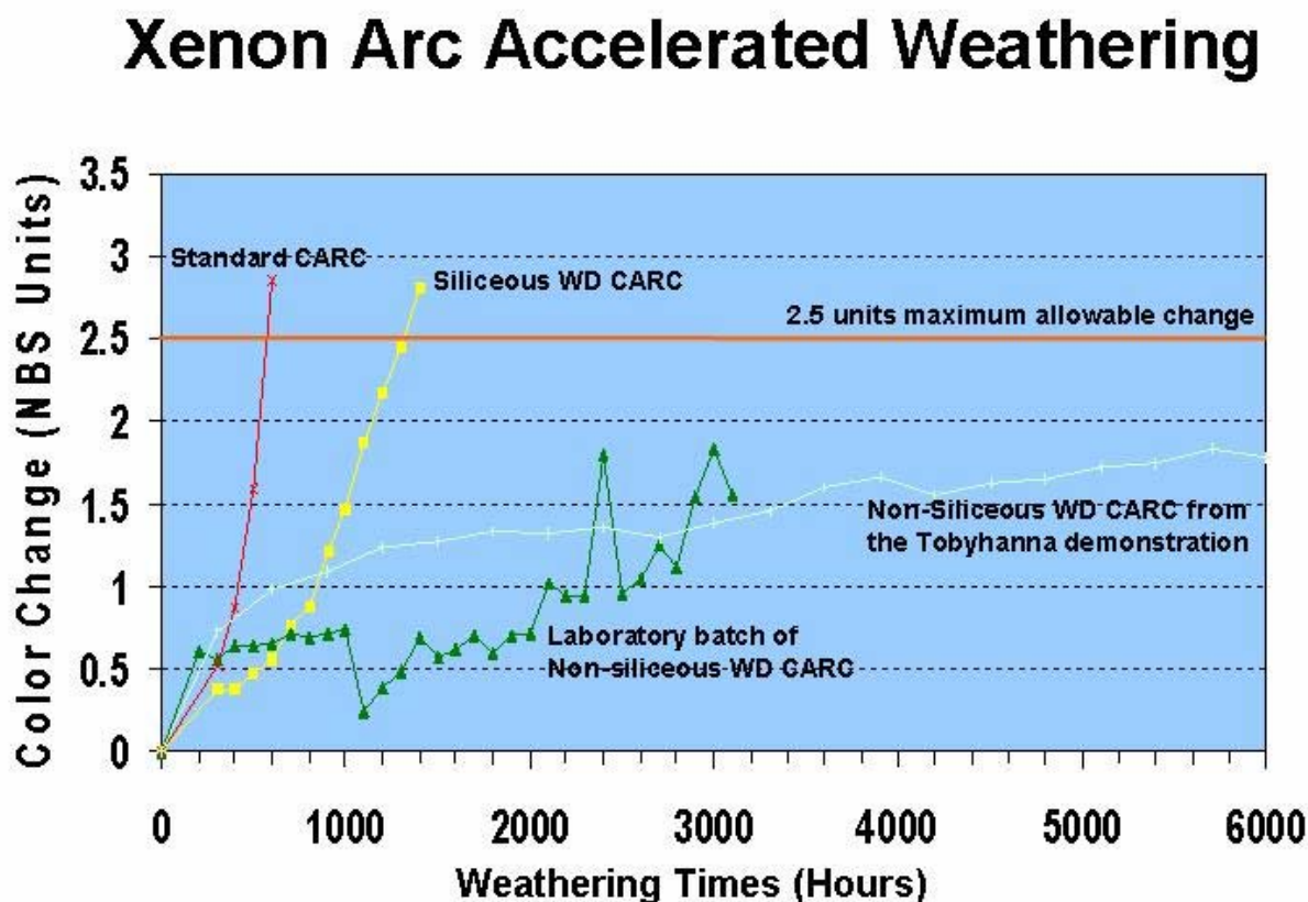
Figure 30 -- Accelerated Weathering Results for Tobyhanna Demonstration
