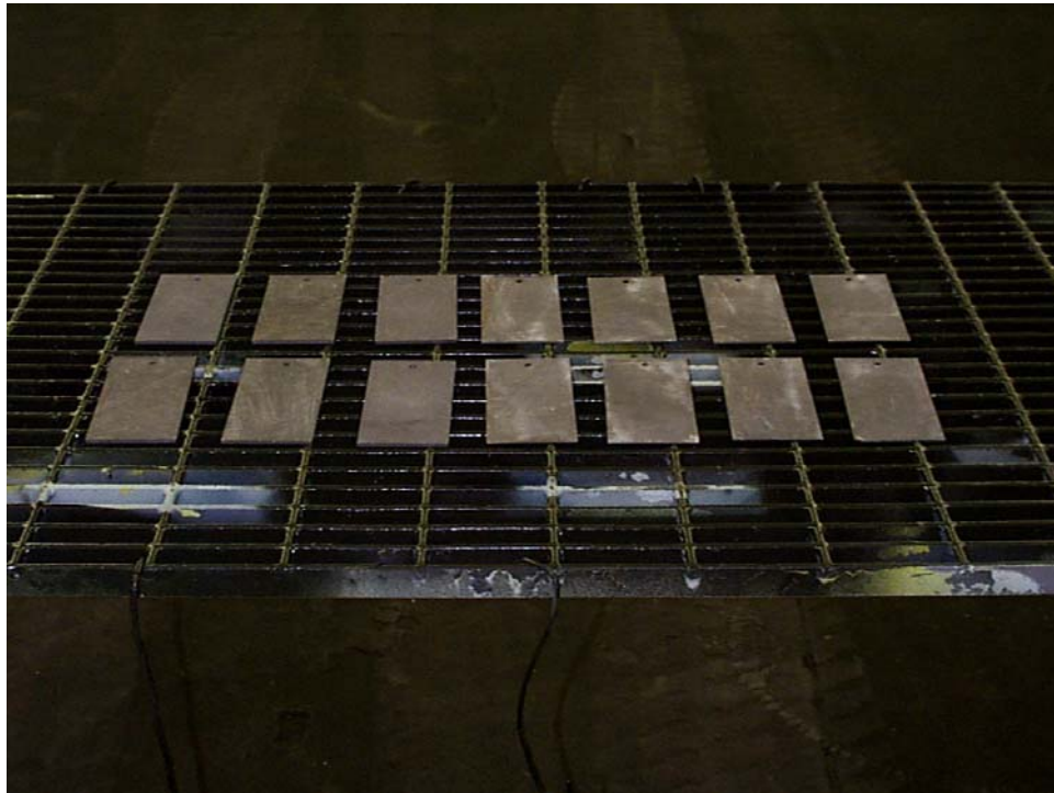
Figure 10 -- Test Panels Before Application of WD CARC at Ogden ALC
