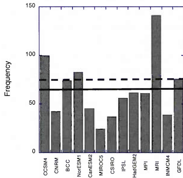
Figure 2. Number of days per year with extreme cyclones in the CMIP5 Historical simulations (1979-2005). Extreme cyclones are defined as occurrences of daily mean SLP at least 40 hPa below the annual average SLP at a grid point. The multi-model average frequency (64.4) is denoted by the solid line and the MERRA average (75.8) by the dashed line.
