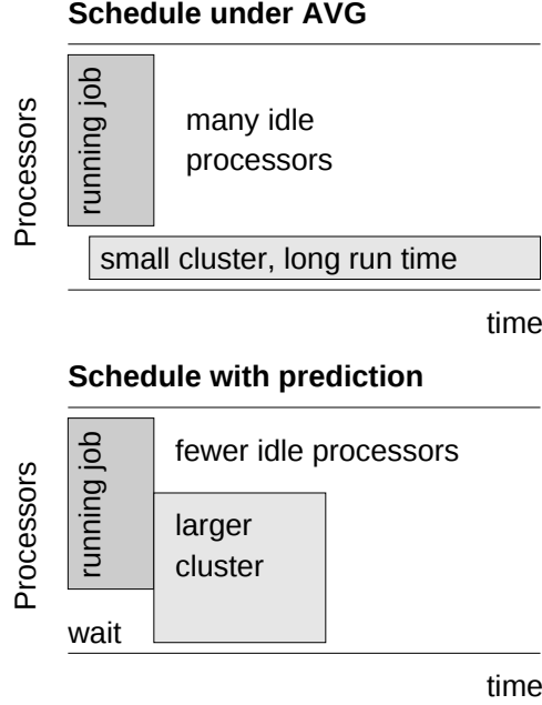
Figure 6: Sample schedules showing how longer queue times and larger cluster sizes can, paradoxically, improve system utilization. Queue time prediction makes it possible to avoid L-shaped schedules and thereby reduce the number of idle processors.
