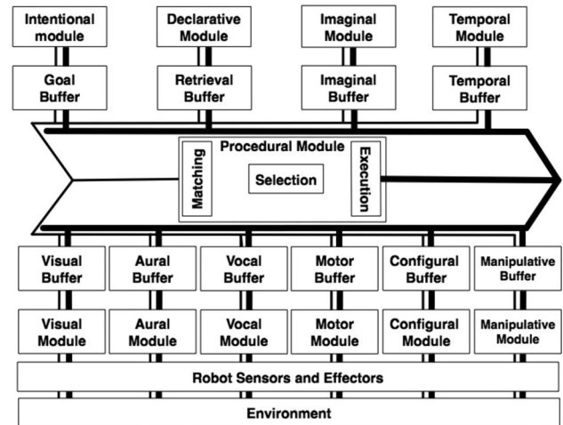
Fig. 1. Schematic of ACT-R/E.
