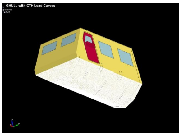
Figure 11: LS-DYNA STL geometry (loaded surfaces shown in white)
