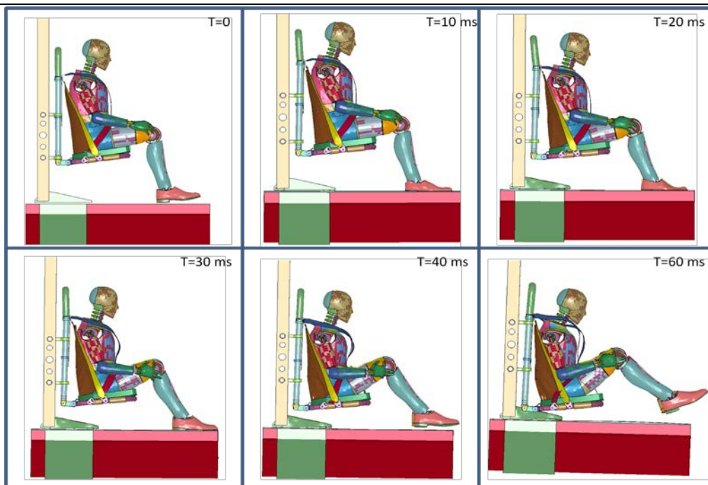
Figure 14: Dummy kinematics at different instants of time
