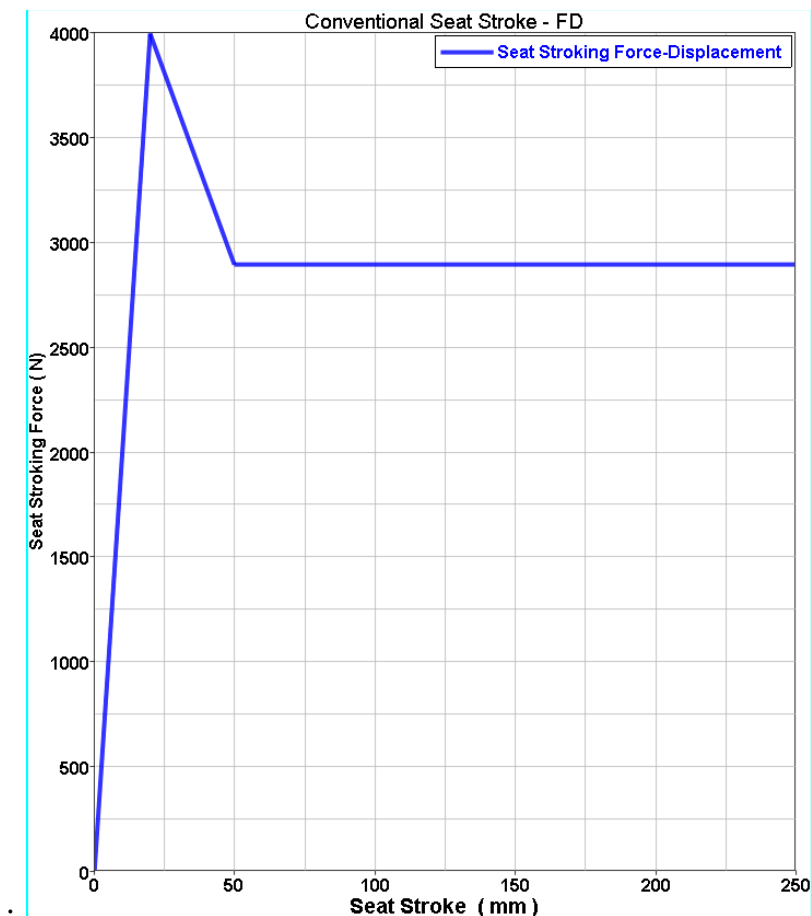
Figure 7: Conventional seat force-displacement (FD) curve
