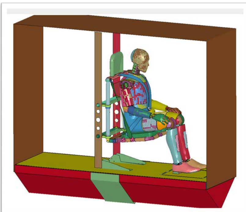
Figure 4: Complete subsystem
