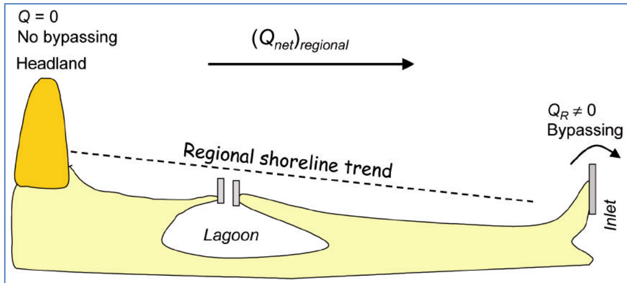
Figure 3. Regional trend in shoreline created by blockage of sand by large headland.
