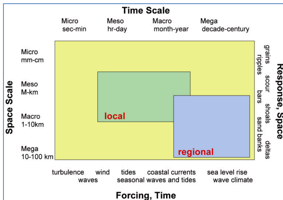
Figure 1. Classification of coastal processes with respect to time and space scales (adapted from Larson and Kraus 1995).
