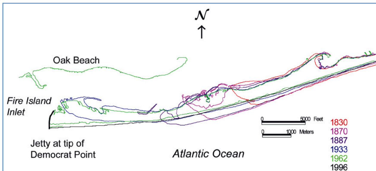
Figure 12. Growth of Fire Island, Long Island, NY.
