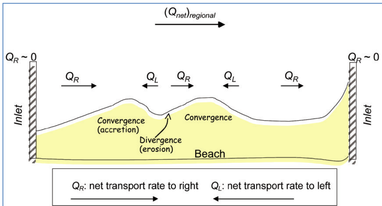
Figure 2. Gradients in the local longshore transport causing areas of erosion and accretion.
