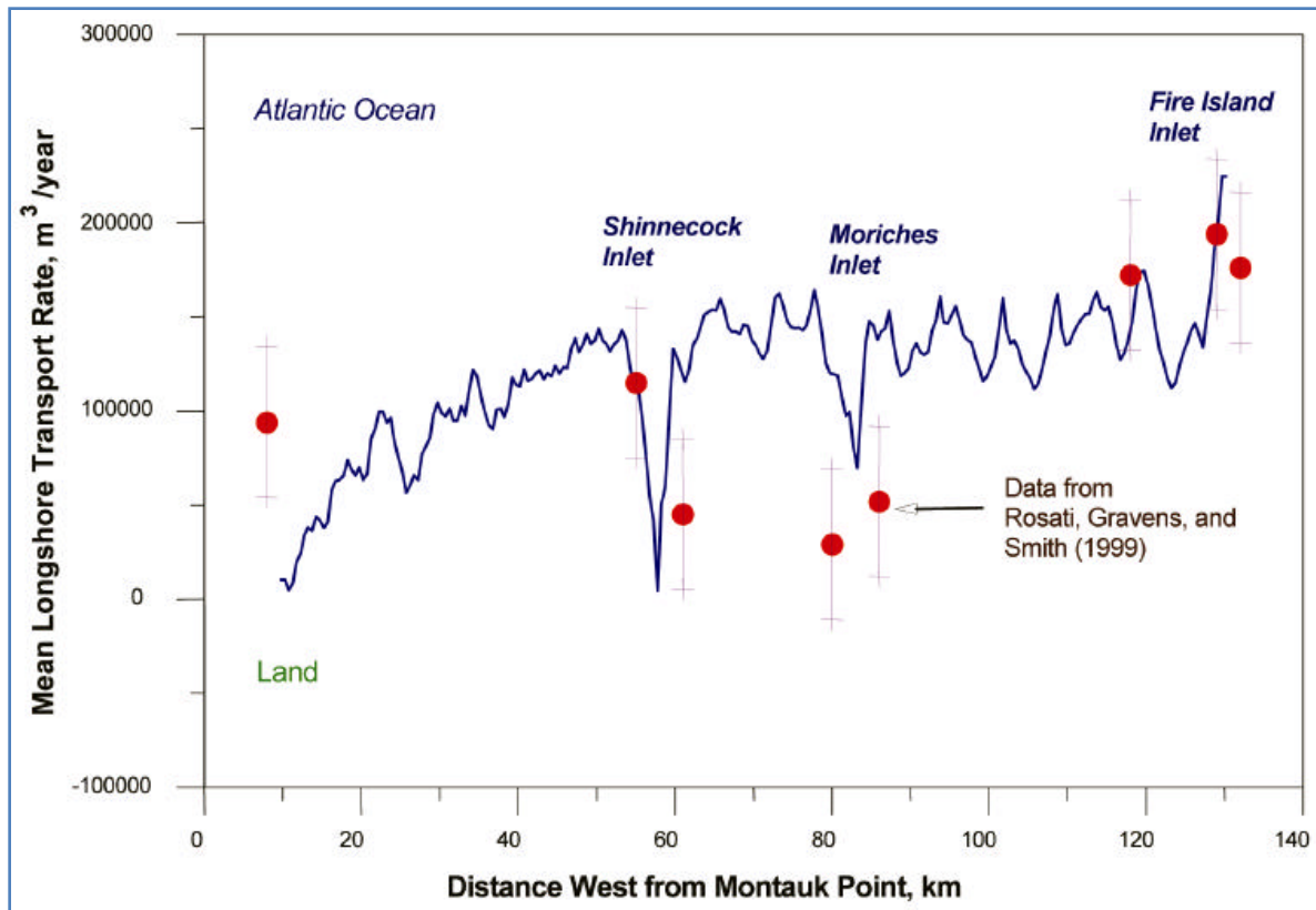
Figure 4. Calculated regional trend in the annual net longshore sand transport along the south shore of Long Island, NY (the horizontal axis goes from east to west).
