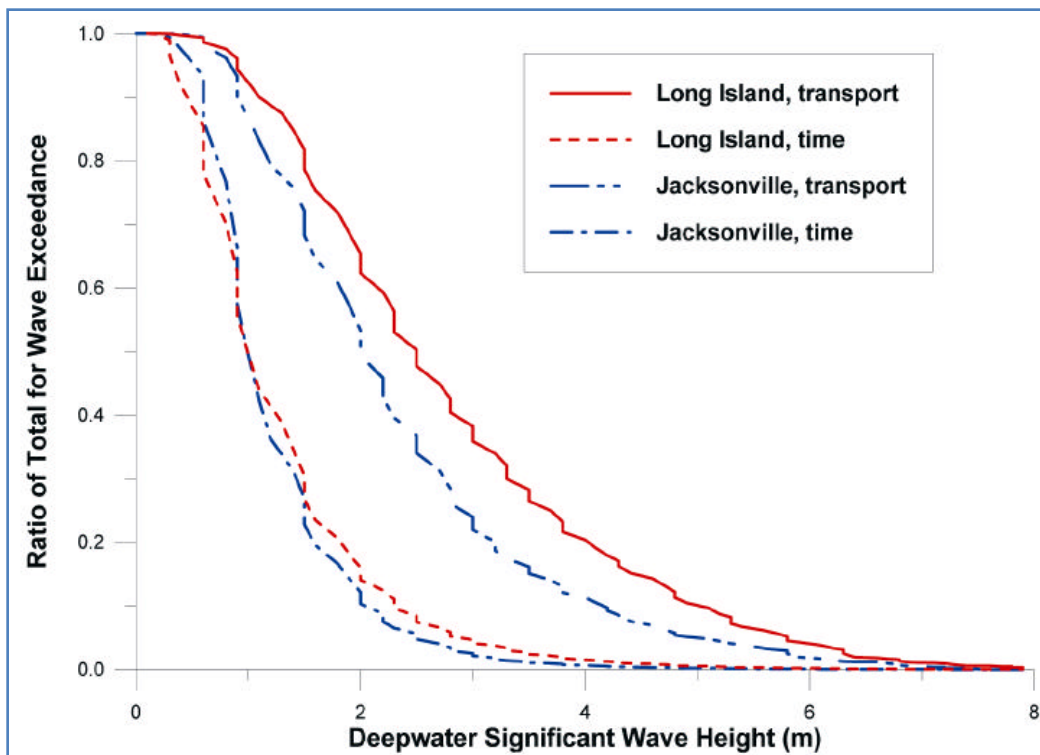
Figure 5. Ratios of total gross longshore sand transport rate and duration of wave action exceeding a specific wave height for Long Island, NY, and Jacksonville, FL.
