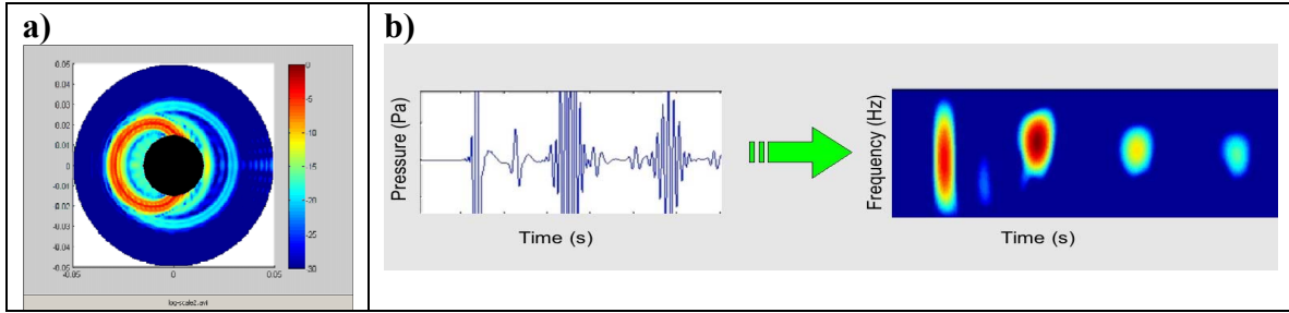
Figure 1: a) Bistatic response of an elastic shell (shell is 1m diameter, 1.5 cm thick steel). b) Time-frequency analysis of the backscatter response of an elastic stell (monostatic response). Note the various (narrowband) strong resonances appearing beyond the firstg specular echo.
