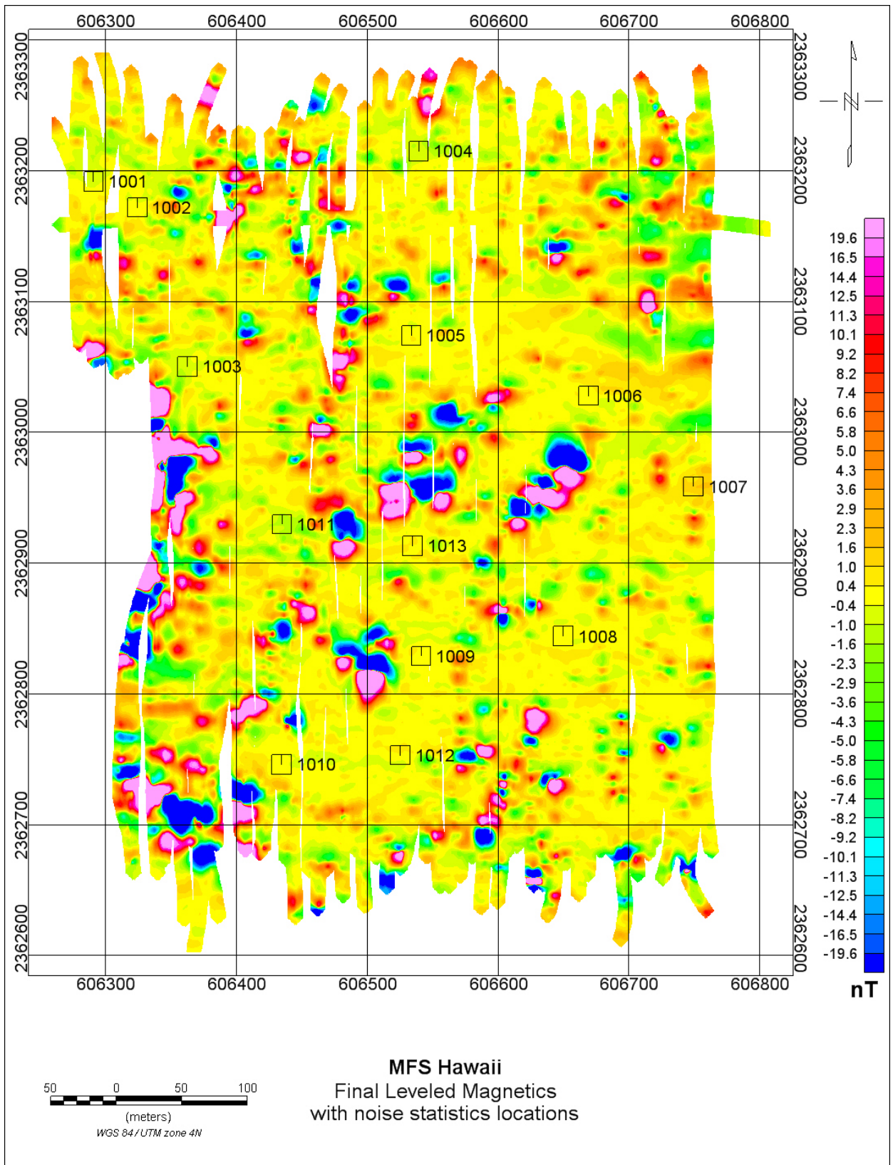
Figure 14. Final levelled magnetics with noise statistic locations overlain. The magnetic data located within the boxes shown were used to derive the noise level statistics.
