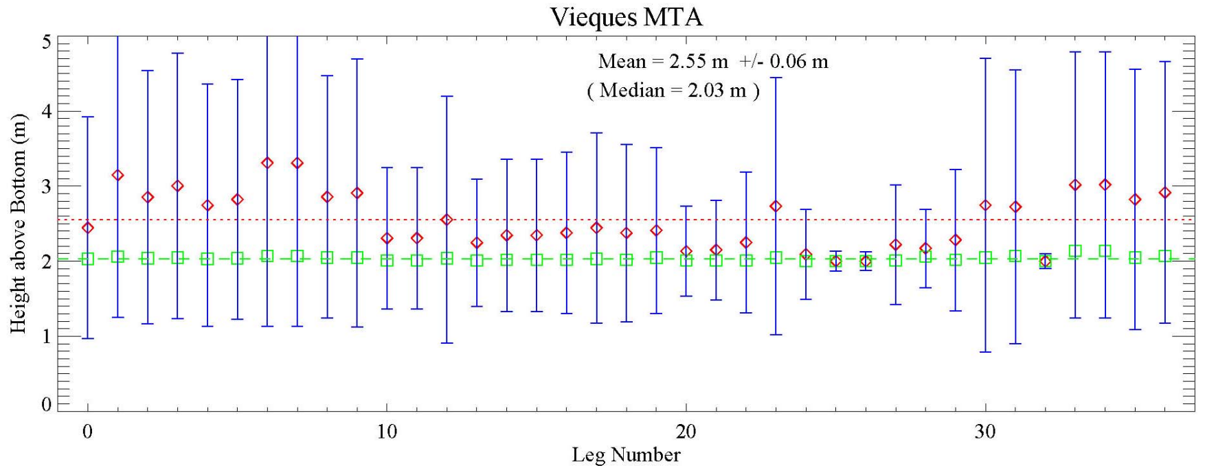
Figure 13 – Plot of the height statistics of the sensor array above the bottom for each leg of survey data. Each leg or separate time series of data is represented by its mean (red diamond), median (green square) and standard deviation (blue bars) about the mean. The red dotted line signifies the mean of the means, while the green dashed lines signifies the median of the medians. In addition, the values of both these levels, along with the standard deviation of the means, are presented for completeness.
