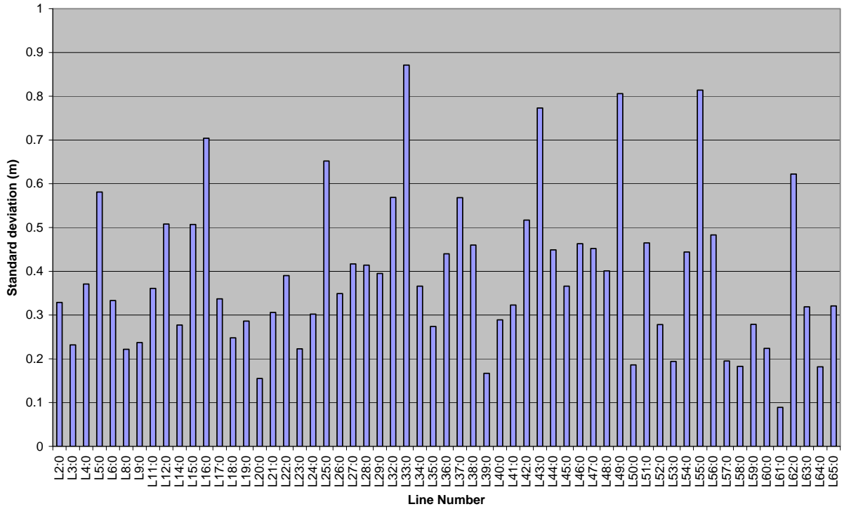
Figure 22. Standard deviation of the sensor height above the sea floor.
