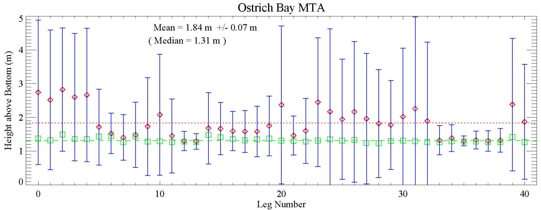
Figure 11 – Plot of the height statistics of the sensor array above the bottom for each leg of survey data. Each leg or separate time series of data is represented by its mean (red diamond), median (green square) and standard deviation (blue bars) about the mean. The red dotted line signifies the mean of the means, while the green dashed lines signifies the median of the medians. In addition, the values of both these levels, along with the standard deviation of the means, are presented for completeness.
