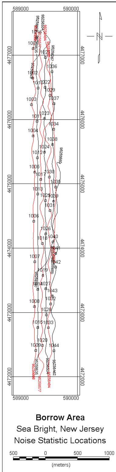
Figure 4. Survey lines with noise statistic locations overlain. The magnetic data located within 15meters of the boxes shown were used to derive the noise level statistics.
