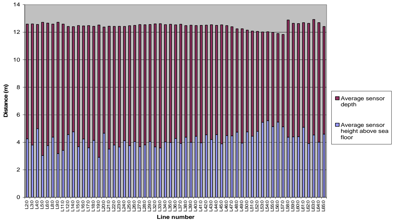
Figure 21. Average sensor depth and sensor height above the sea floor for each survey line. The sum of these two components gives the water depth.
