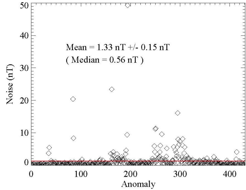
Figure 24 – The left panel shows a histogram of the SNR, expressed in decibels, for all the anomalies analyzed in the magnetometer data collected with the MTA at Duck, NC. The right panel shows a plot of the noise levels derived from the spatially outlying data for each anomaly. The mean noise level (red line) is presented with an uncertainty given by the standard deviation of the mean. The median noise level is also presented as a comparison.
