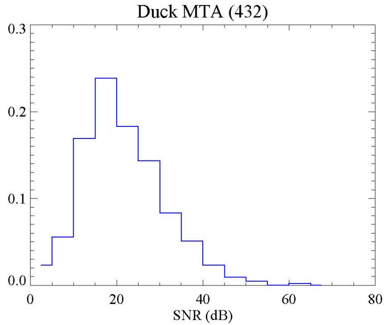
Figure 24 – The left panel shows a histogram of the SNR, expressed in decibels, for all the anomalies analyzed in the magnetometer data collected with the MTA at Duck, NC. The right panel shows a plot of the noise levels derived from the spatially outlying data for each anomaly. The mean noise level (red line) is presented with an uncertainty given by the standard deviation of the mean. The median noise level is also presented as a comparison.
