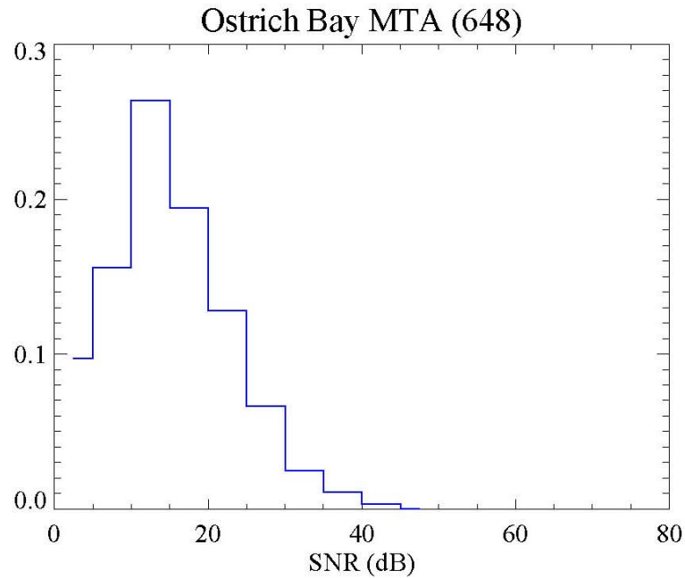
Figure 25 – The left panel shows a histogram of the SNR, expressed in decibels, for all the anomalies analyzed in the magnetometer data collected with the MTA at Ostrich Bay, WA. The right panel shows a plot of the noise levels derived from the spatially outlying data for each anomaly. The mean noise level (red line) is presented with an uncertainty given by the standard deviation of the mean. The median noise level is also presented as a comparison.
