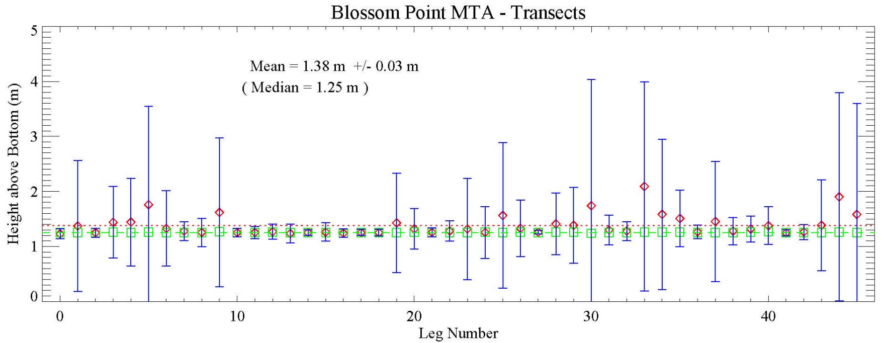
Figure 14 – Plot of the height statistics of the sensor array above the bottom for each leg of survey data. Each leg or separate time series of data is represented by its mean (red diamond), median (green square) and standard deviation (blue bars) about the mean. The red dotted line signifies the mean of the means, while the green dashed lines signifies the median of the medians. In addition, the values of both these levels, along with the standard deviation of the means, are presented for completeness.
