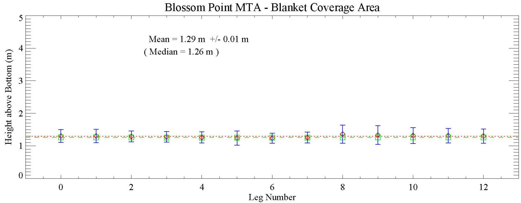
Figure 15 – Plot of the height statistics of the sensor array above the bottom for each leg of survey data. Each leg or separate time series of data is represented by its mean (red diamond), median (green square) and standard deviation (blue bars) about the mean. The red dotted line signifies the mean of the means, while the green dashed lines signifies the median of the medians. In addition, the values of both these levels, along with the standard deviation of the means, are presented for completeness.
