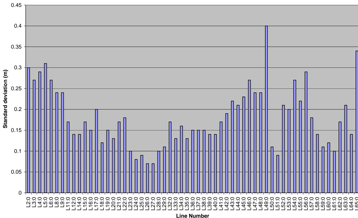
Figure 23. Standard deviation of the sea floor relief model calculated from the depth and altimeter sensors.
