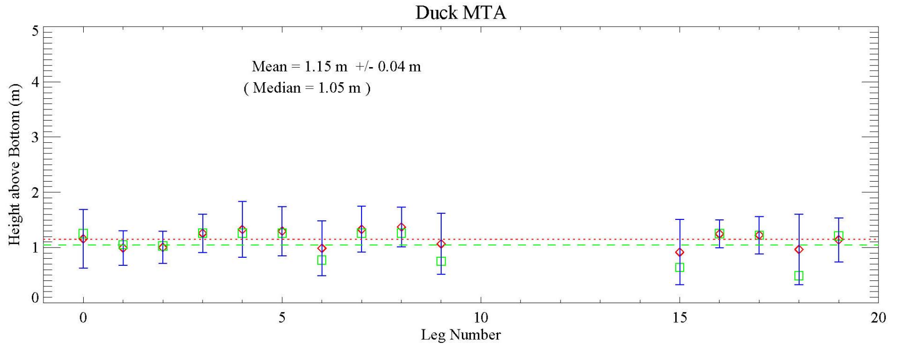
Figure 10 – Plot of the height statistics of the sensor array above the bottom for each leg of survey data. Each leg or separate time series of data is represented by its mean (red diamond), median (green square) and standard deviation (blue bars) about the mean. The red dotted line signifies the mean of the means, while the green dashed lines signifies the median of the medians. In addition, the values of both these levels, along with the standard deviation of the means, are presented for completeness.
