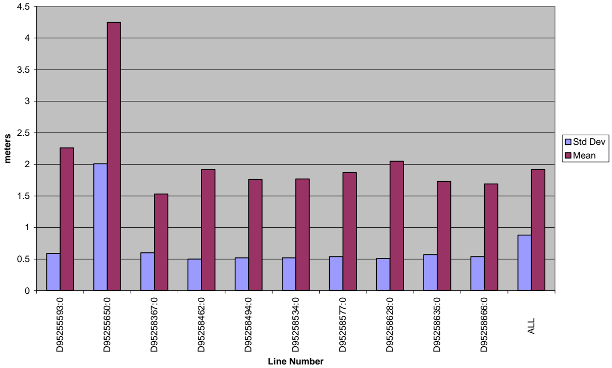
Figure 6. Standard deviation and mean of the sensor height above the sea floor.
