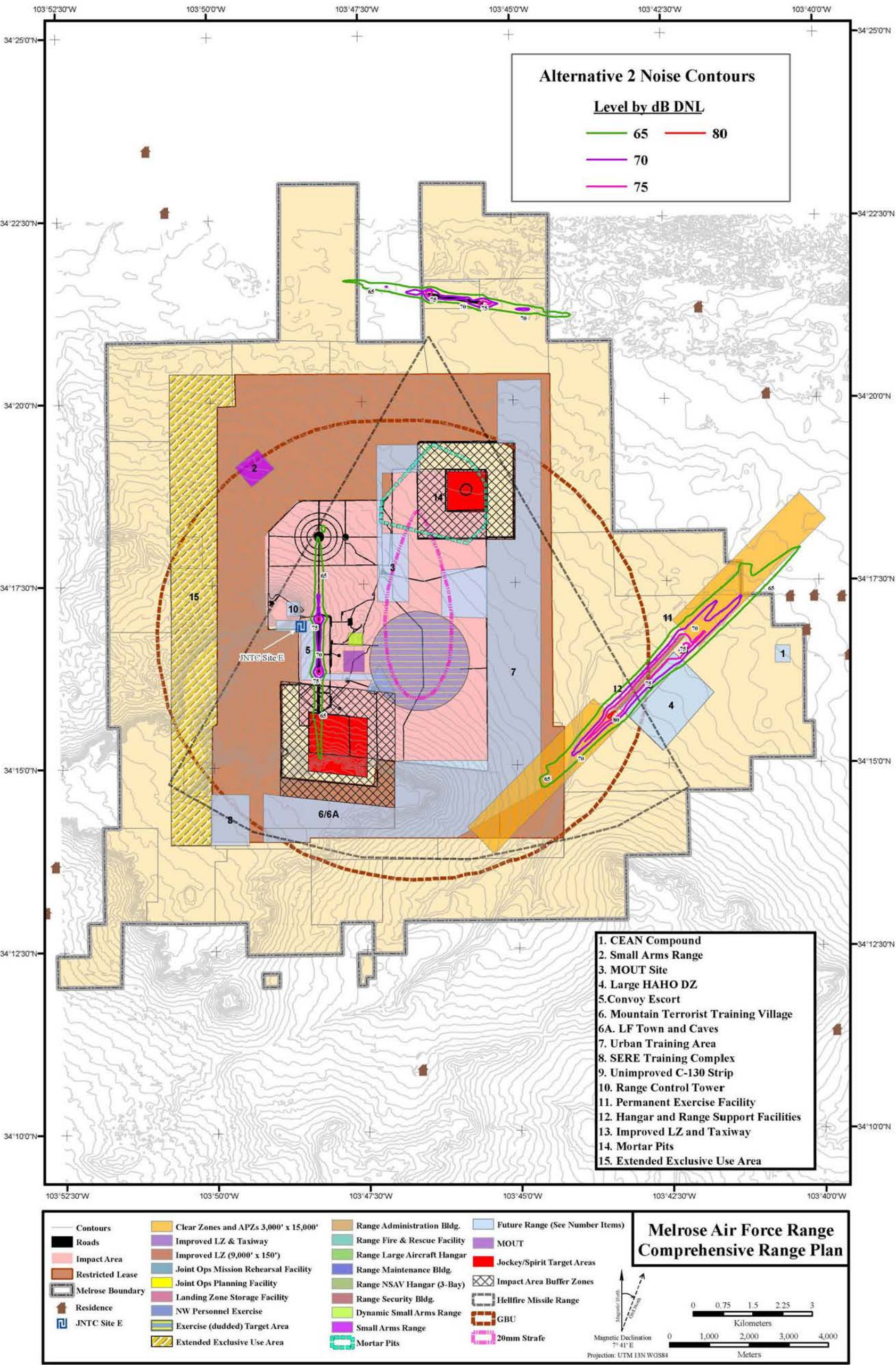
Figure 4-3. Alternative 2 Aircraft Noise Contours for Melrose AFR
