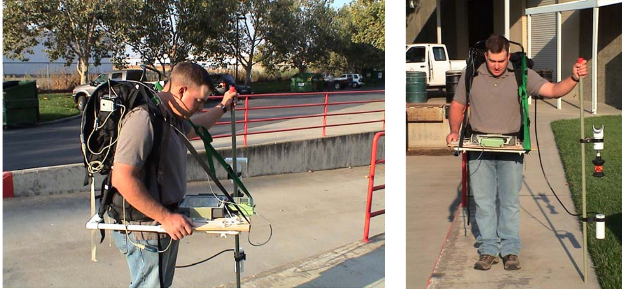
Figure 3-1. Two Pictures of the RTS/Geophysical Sensor Setup Prior to Phase III Deployment. (Note: Fiberglass pole utilized in place of G858 standard poles prior to deployment.)
