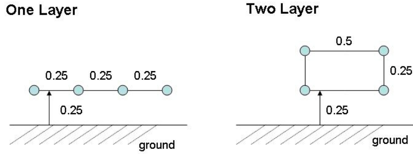
Figure 3: Scenarios for one- and two-layer measurements
