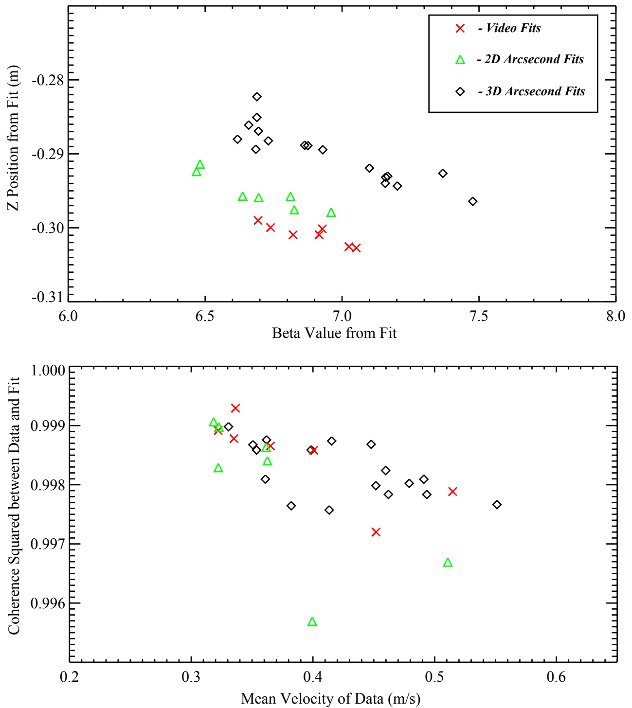
Figure 5. Results of fitting EM61-HH data with model using different positioning data.
