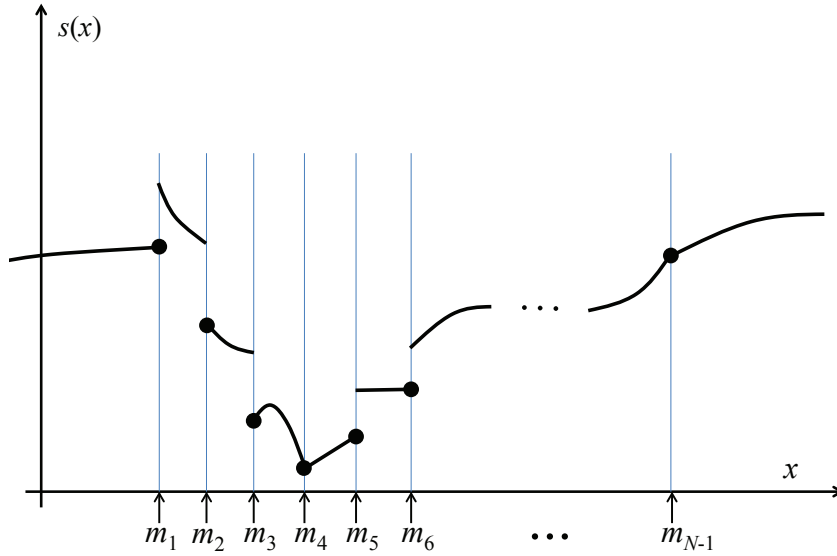
Figure 7: Mesh and epi-spline on \mathbb{R} .
