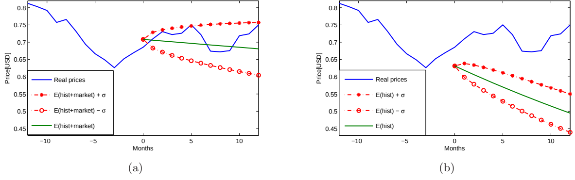
Figure 4: Epi-spline estimates of copper prices (a) with and (b) without future contract information.
