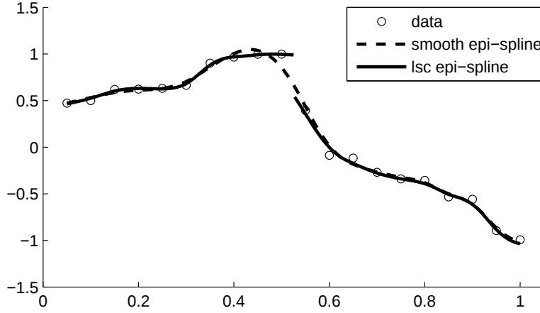
Figure 3: Second-order epi-spline fits with and without discontinuity.
