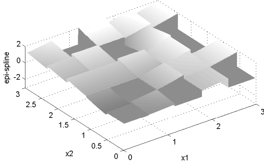
Figure 8: Epi-spline on \mathbb{R}^2 .
