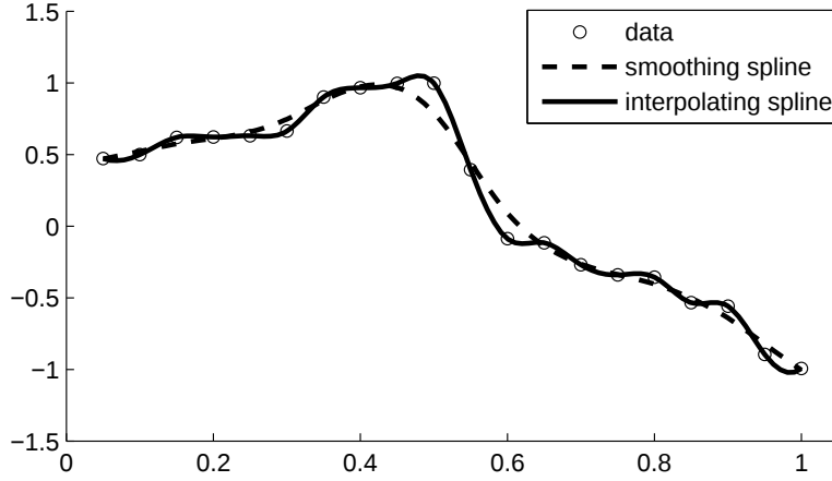
Figure 2: Cubic interpolating and smoothing spline fits.
