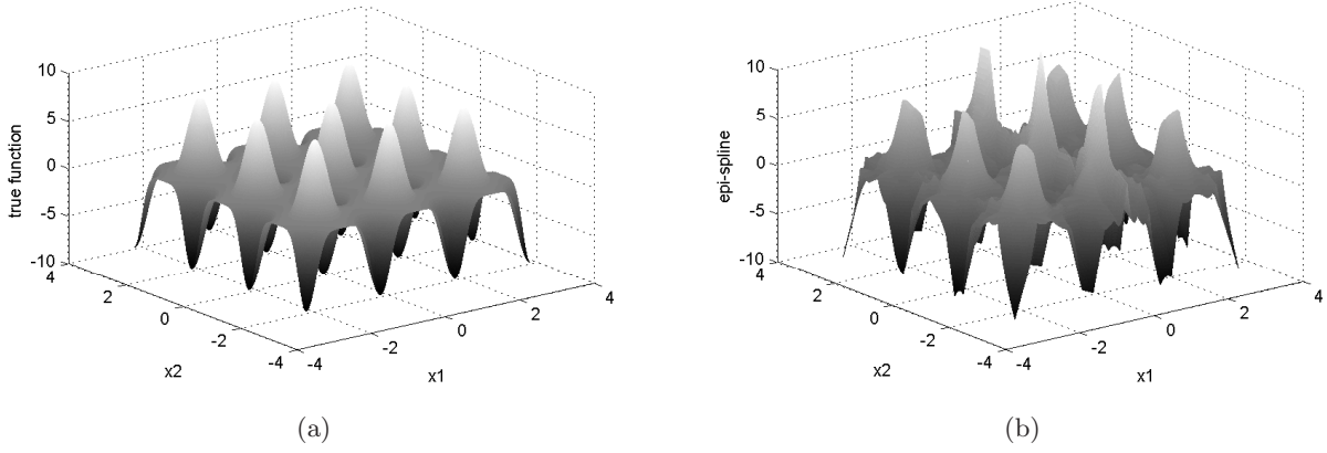
Figure 13: Image reconstruction example: actual function (a) and epi-spline (b).
