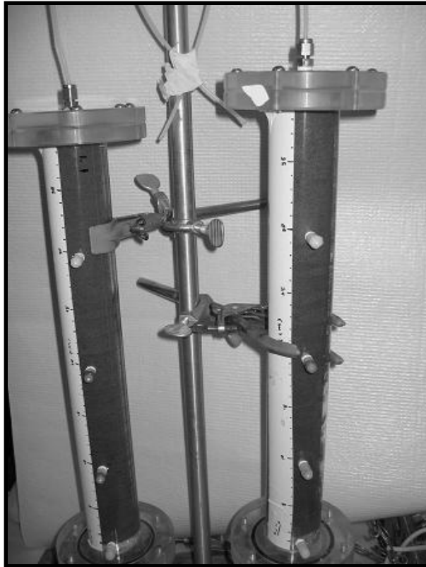
Figure 24: Typical columns used in permanganate experiments. Each column has a length of 40 cm and an inner diameter of 3.81 cm, and is equipped with four equally spaced sampling ports along its length.
