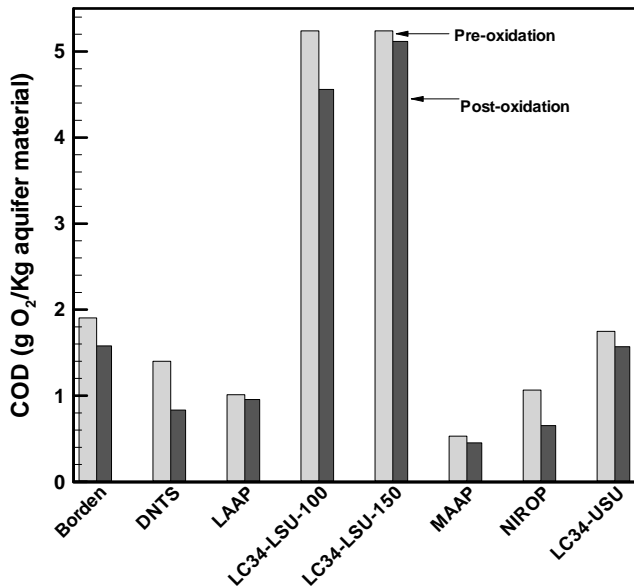
Figure 44: Pre- and post-oxidant dichromate COD test results for the batch reactors systems.
