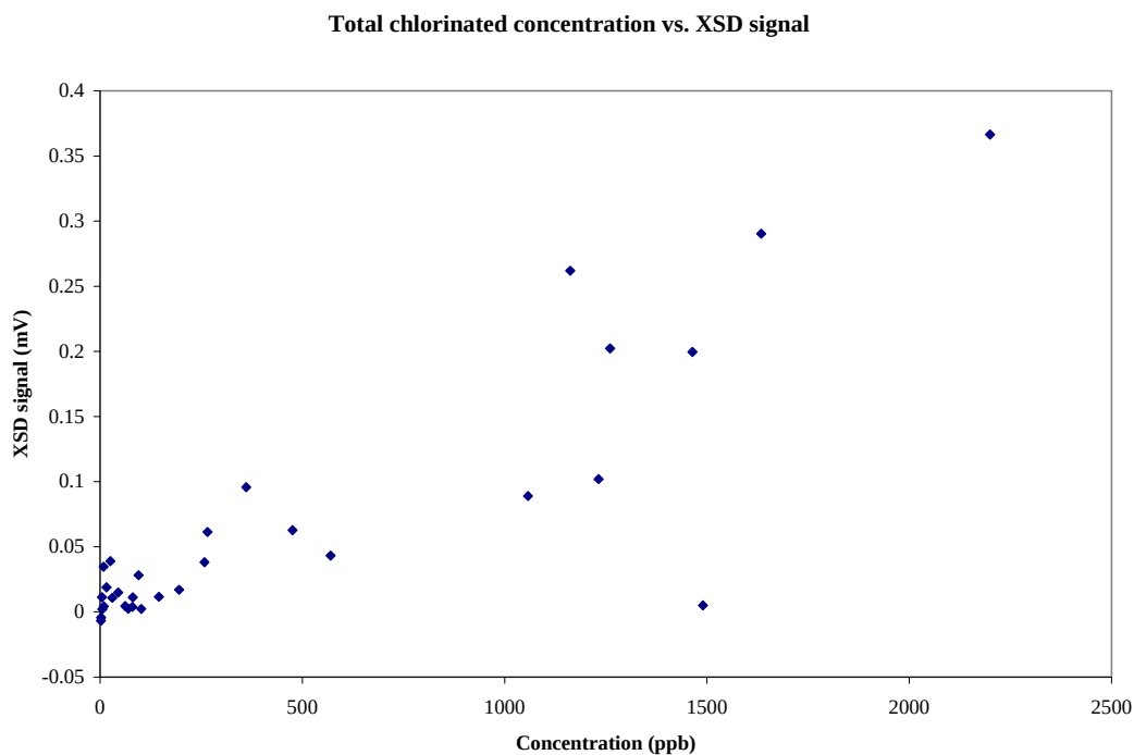
Figure 20. Correlation of XSD data with laboratory analysis of water samples collected from nearby monitoring well.
