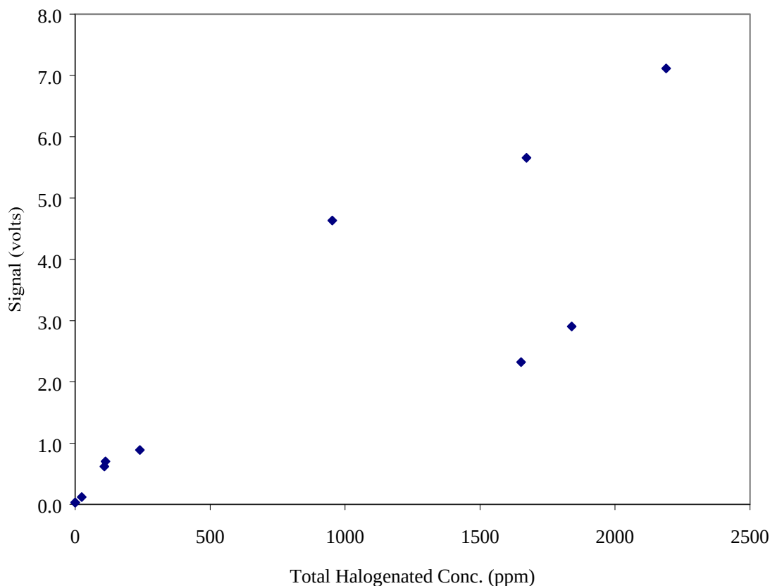
Figure 45. Comparison of laboratory water sample concentrations with XSD-MIP signals on water sample splits
