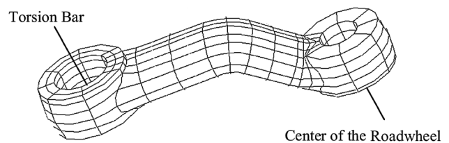
Fig. 7 Finite element model of roadarm
