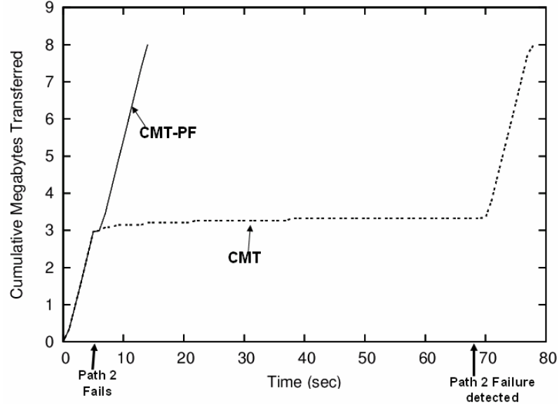
Figure 4.6: CMT vs. CMT-PF during Permanent Failure
