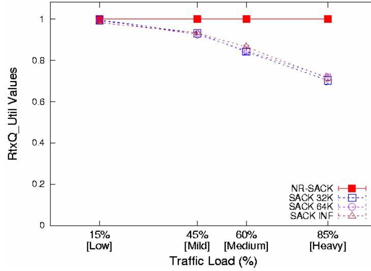
Figure 3.8: RtxQ Utilization in SCTP
