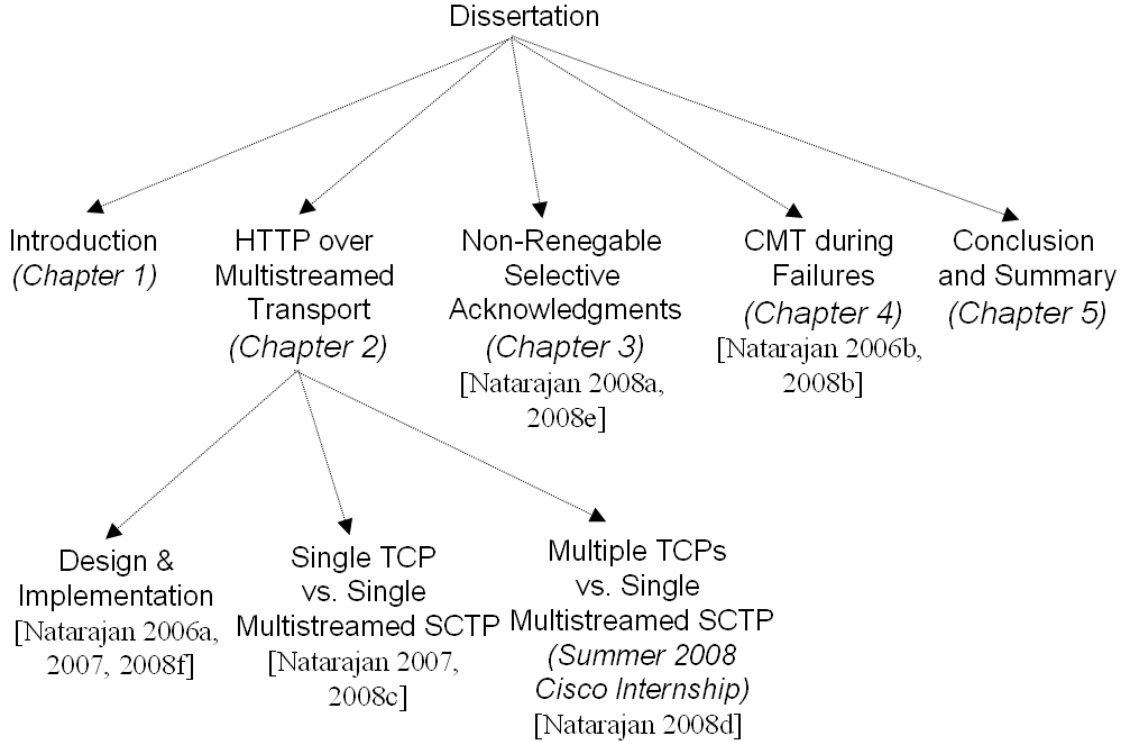
Figure 1.3: Dissertation Structure
