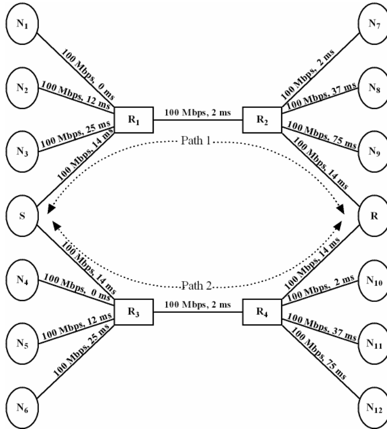
Figure 3.6: Topology for CMT Experiments (Topology 2)
