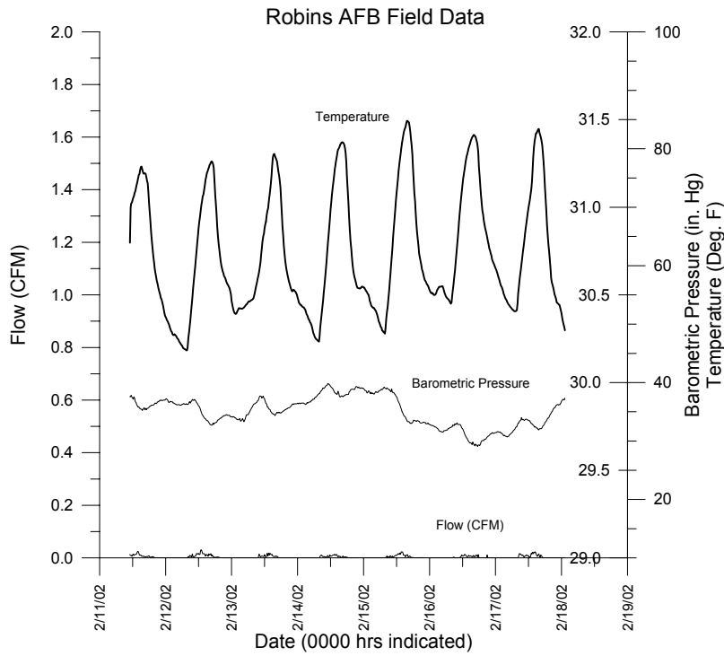
Figure 23. Robins AFB Field Data Plot
