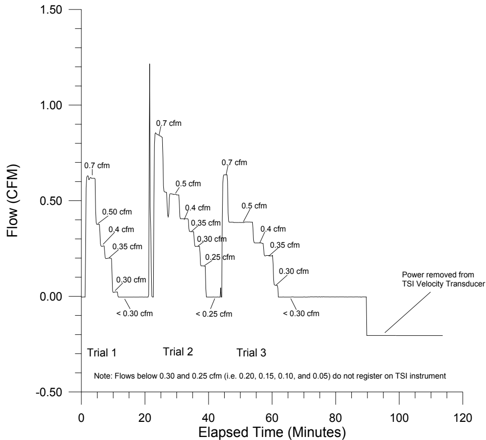
Figure C-6. Results of Mass Flow Controller Test
