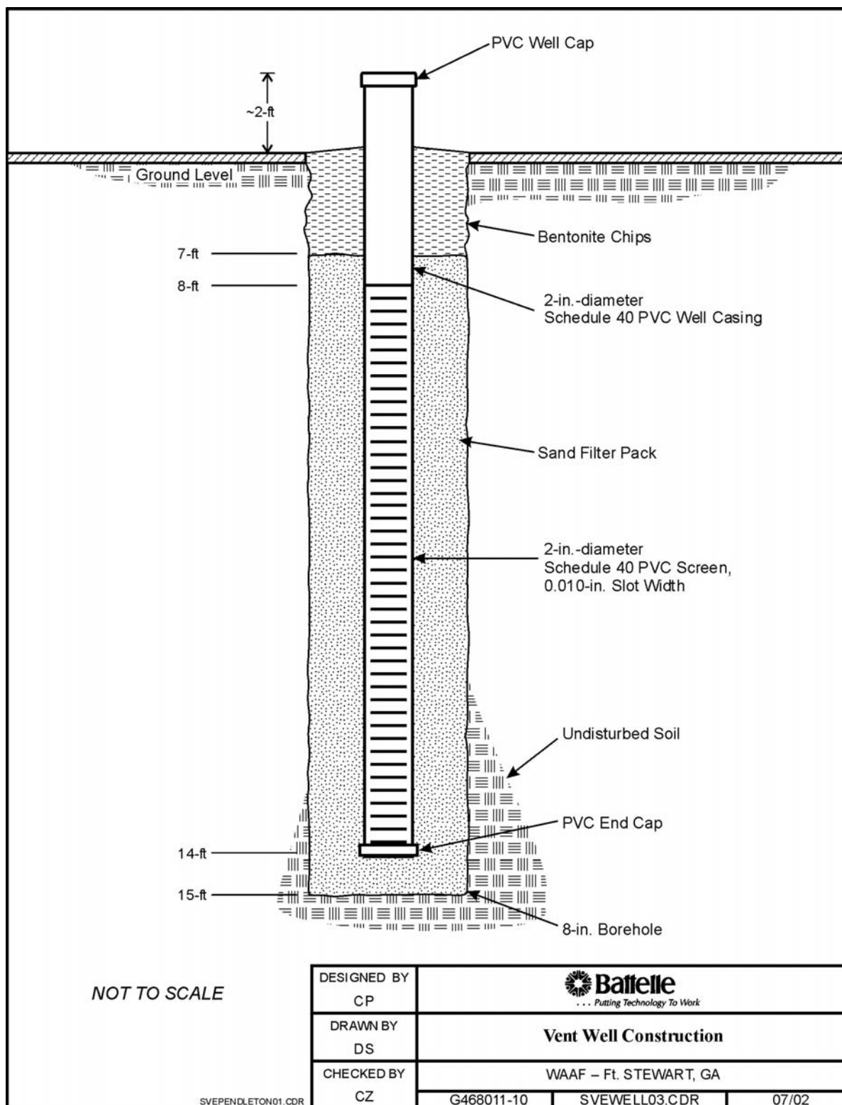
Figure 19. Vent Well Installation Schematic at Fort Stewart
