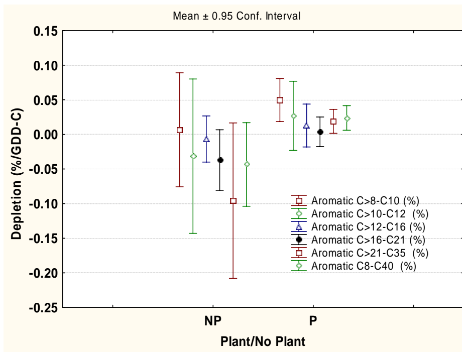
Figure 12. Three ESTCP Field Sites—Decalin and GDD Normalized Data—Plant Effects on Aromatic Fractions.
