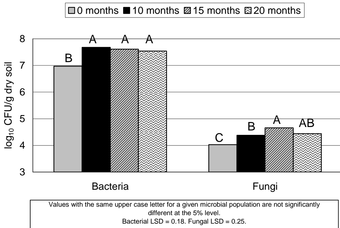
Figure 15. Bacterial and Fungal Population Changes Over Time at the Annette Island Site.
