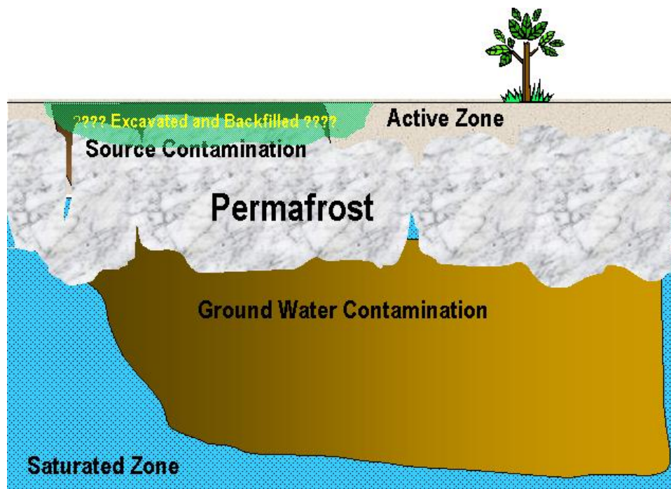
Figure 6. Depiction of Permafrost Effects on Contaminant Sources and Groundwater Contamination. Permafrost May or May Not Serve as a Barrier.
