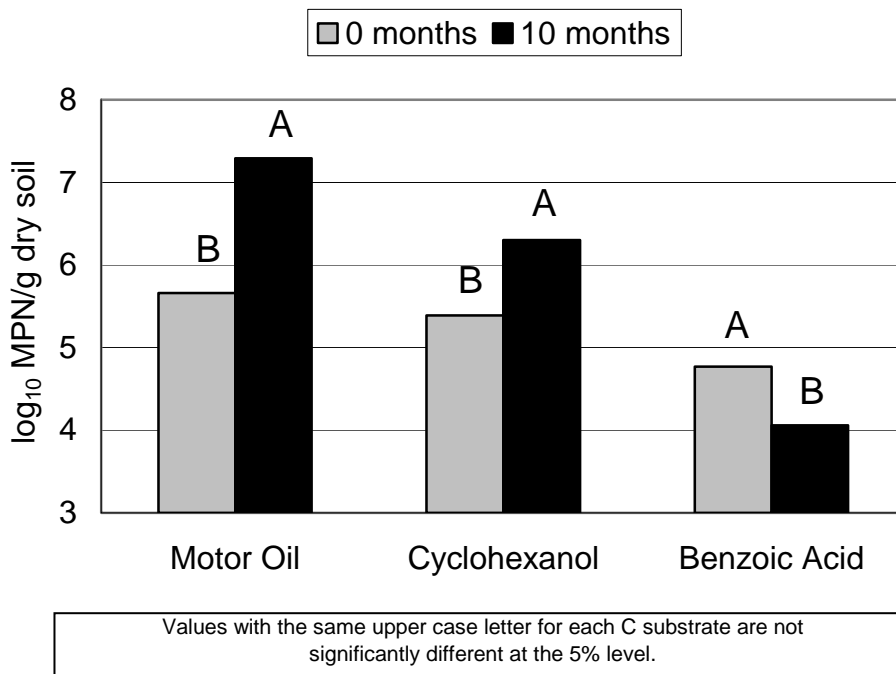
Figure 17. Motor Oil, Cyclohexanol, and Benzoic Acid Degradation Numbers Before and 10 Months After Treatments Were Implemented at the Annette Island Site.
