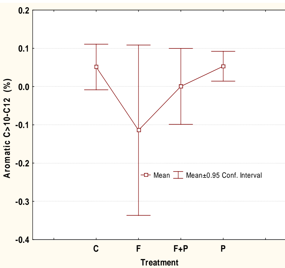
Figure 9. Three ESTCP Field Sites—Decalin and GDD Normalized Data—Treatment Effects on Aromatic C>10-C12.
