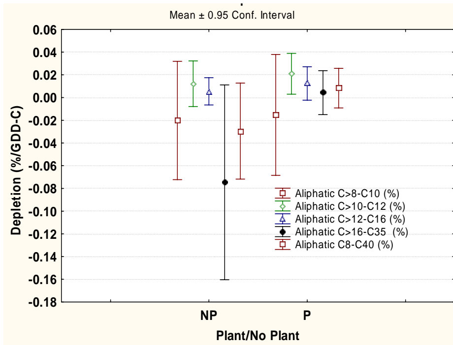
Figure 11. Three ESTCP Field Sites—Decalin and GDD Normalized Data—Plant Effects on Aliphatic Fractions.
