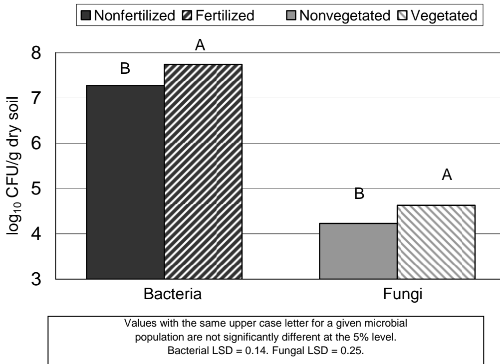
Figure 16. Bacterial Populations in the Non-Fertilized and Fertilized Plots, and Fungal Populations in the Non-Vegetated and Vegetated Plots at the Annette Island Site.
