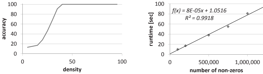
(a) Tensor with disjoint blocks - Com2 identifies communities even at low densities.
