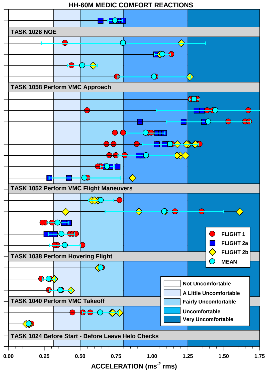
Figure A-26. ISO Comfort Reactions and \sigma VTVs \pm One Standard Deviation at the HH-60M Medic Station
