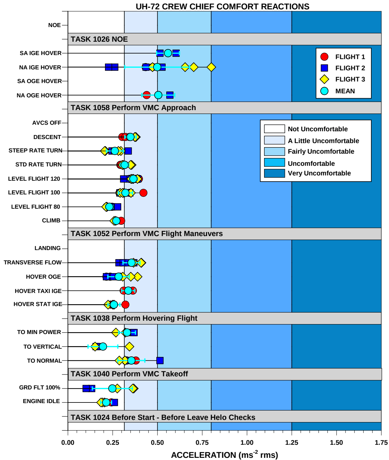
Figure A-22. ISO Comfort Reactions and oVTVs \pm One Standard Deviation at the UH-72 Crew Chief Station
