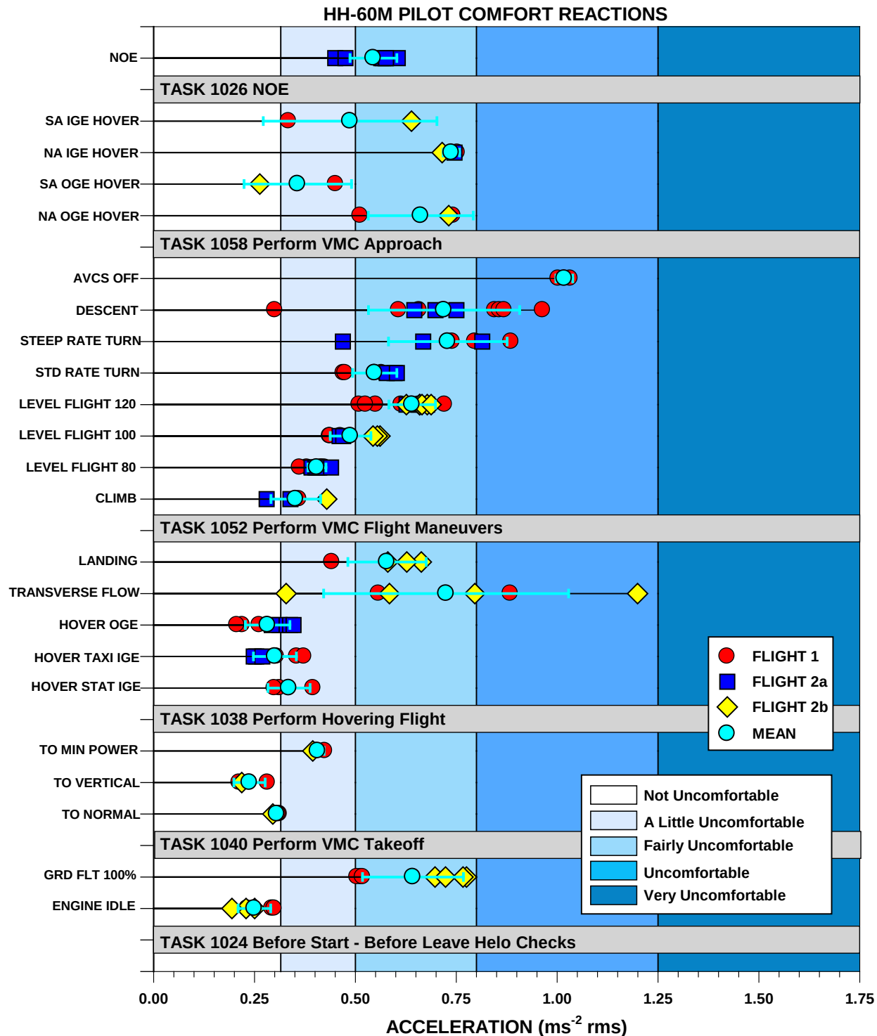
Figure A-24. ISO Comfort Reactions and oVTVs \pm One Standard Deviation at the HH-60M Pilot Station
