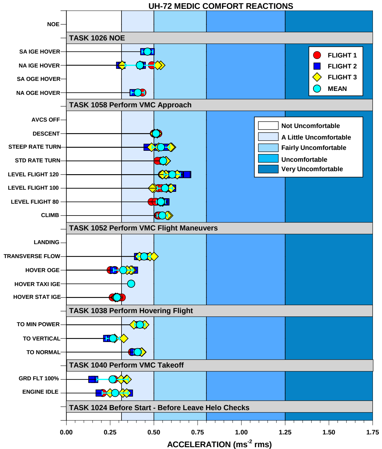
Figure A-23. ISO Comfort Reactions and oVTVs \pm One Standard Deviation at the UH-72 Medic Station
