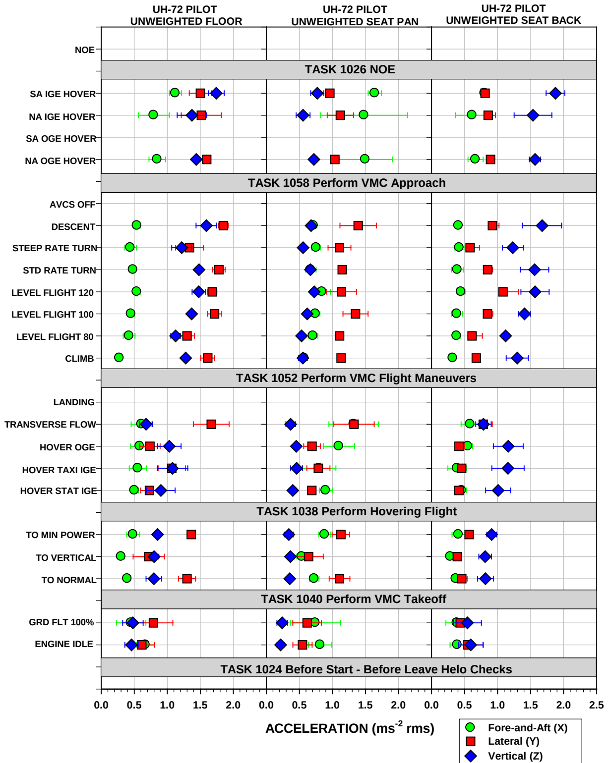
Figure A-7. UH-72 Mean Overall Unweighted Accelerations \pm One Standard Deviation at the Pilot Station
