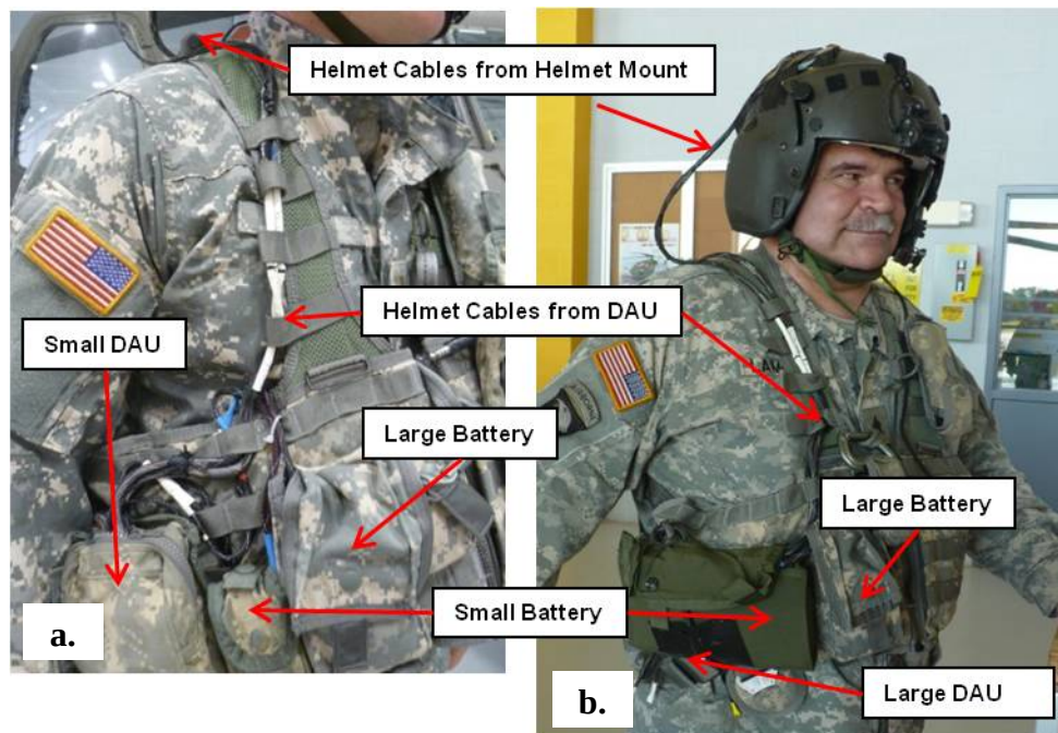
Figure 3. DAU and battery packs carried in survival vest at a. Pilot Station and b. Crew Chief Station
