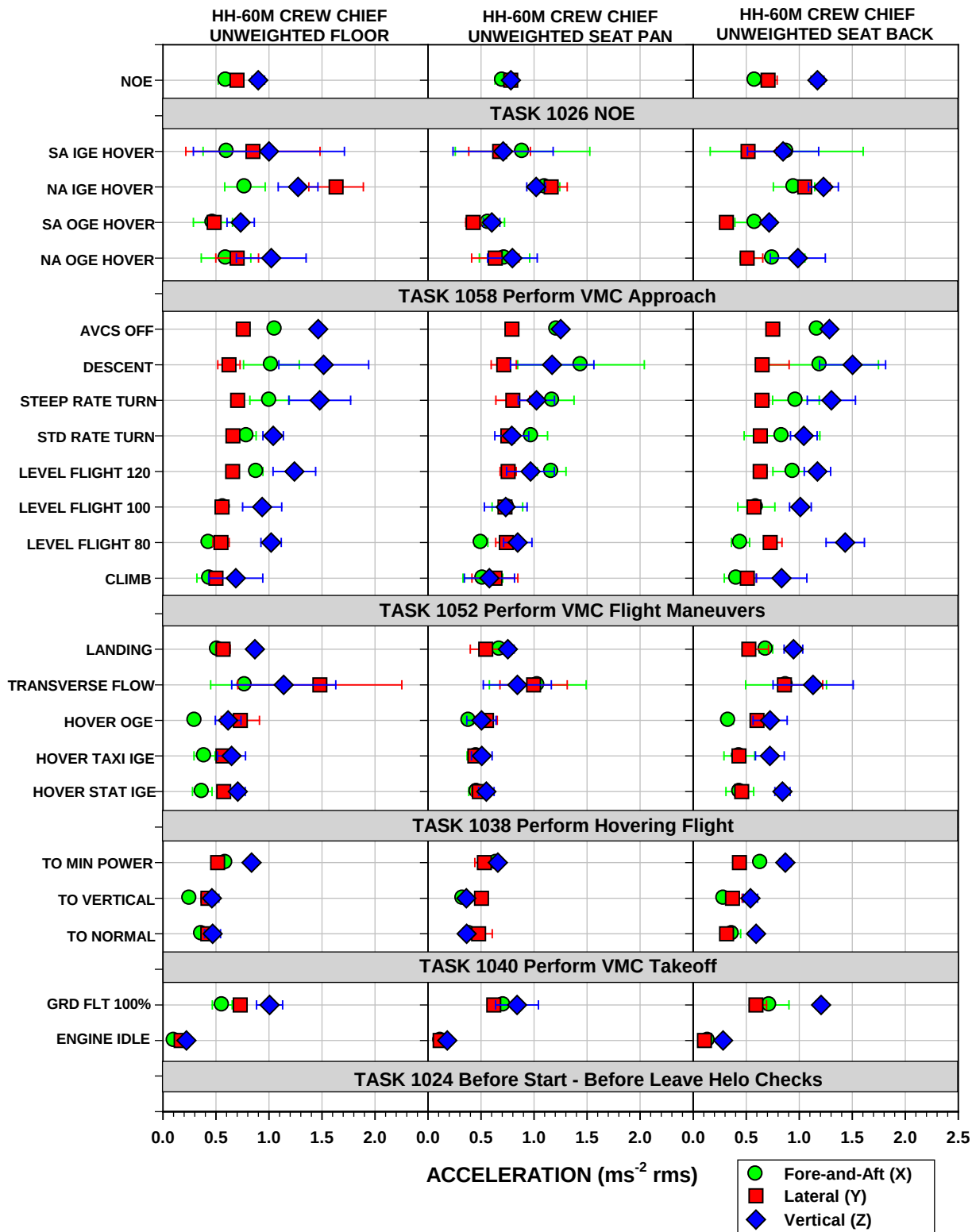
Figure A-15. HH-60M Mean Overall Unweighted Accelerations \pm One Standard Deviation at the Crew Chief Station
