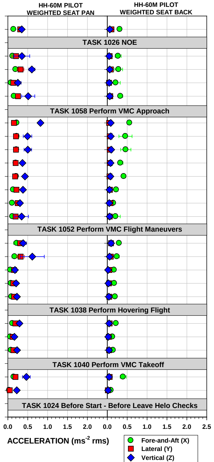
Figure A-17. HH-60M Mean Overall Weighted Accelerations ± One Standard Deviation at the Pilot Station
