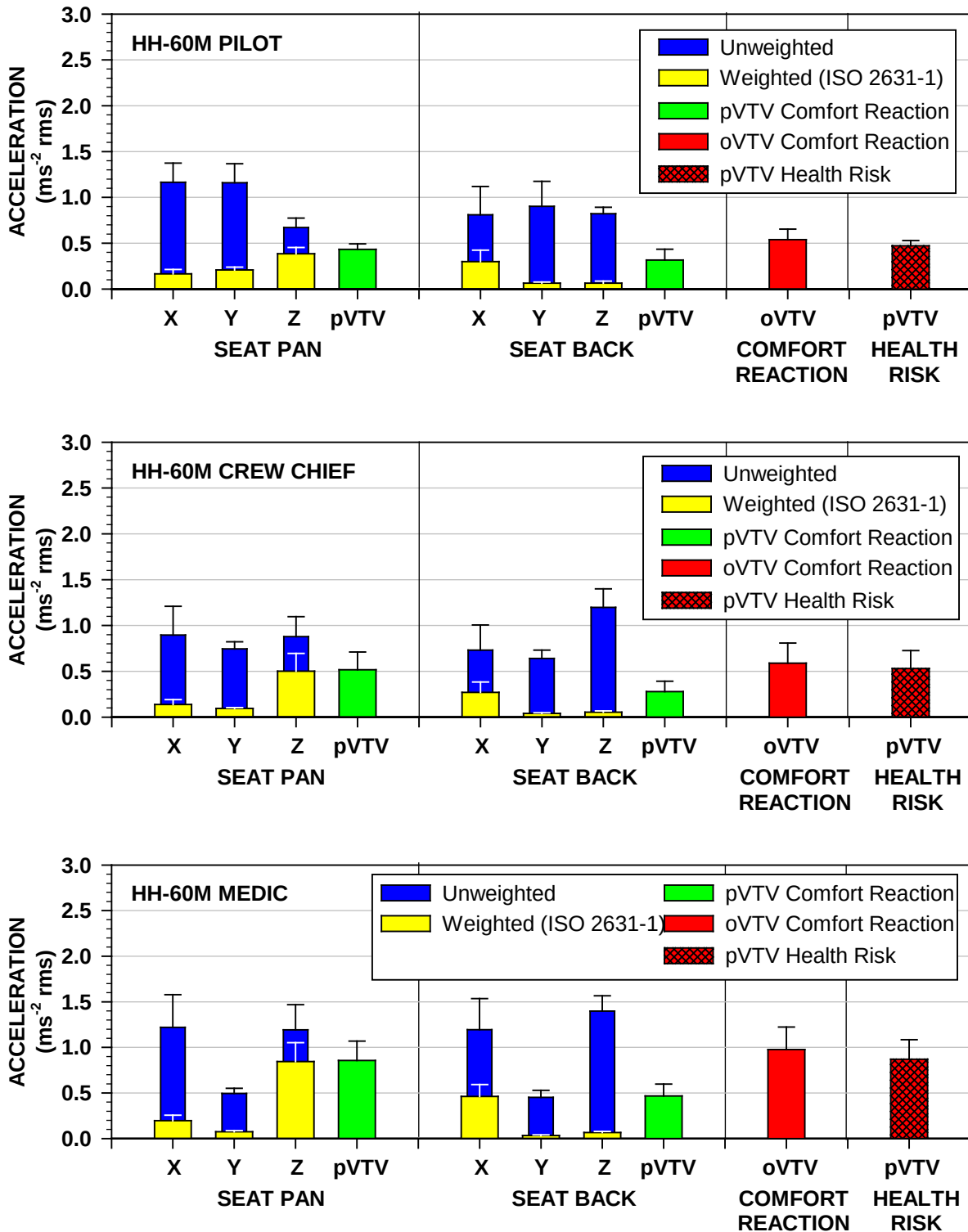
Figure A-20. HH-60M Mean Overall Unweighted and Weighted Accelerations, pVTVs, and oVTVs + One Standard Deviation for Level Flight
