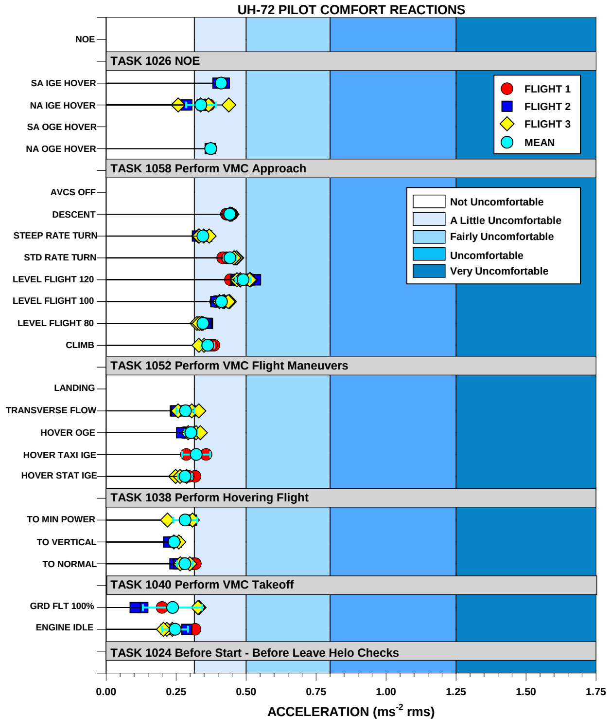
Figure A-21. ISO Comfort Reactions and oVTVs ± One Standard Deviation at the UH-72 Pilot Station
