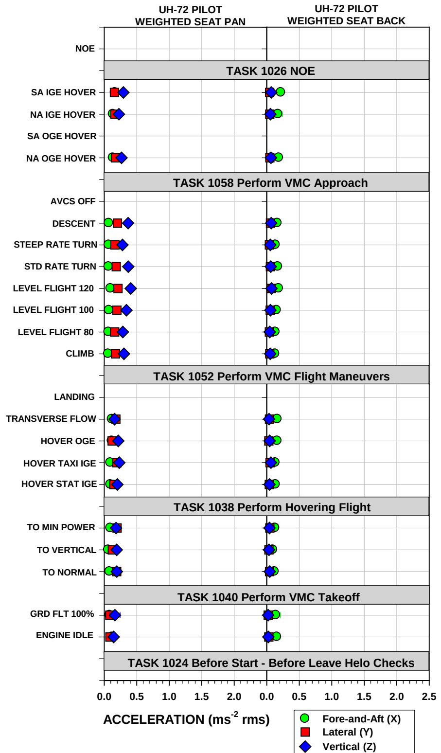
Figure A-10. UH-72 Mean Overall Weighted Accelerations ± One Standard Deviation at the Pilot Station
