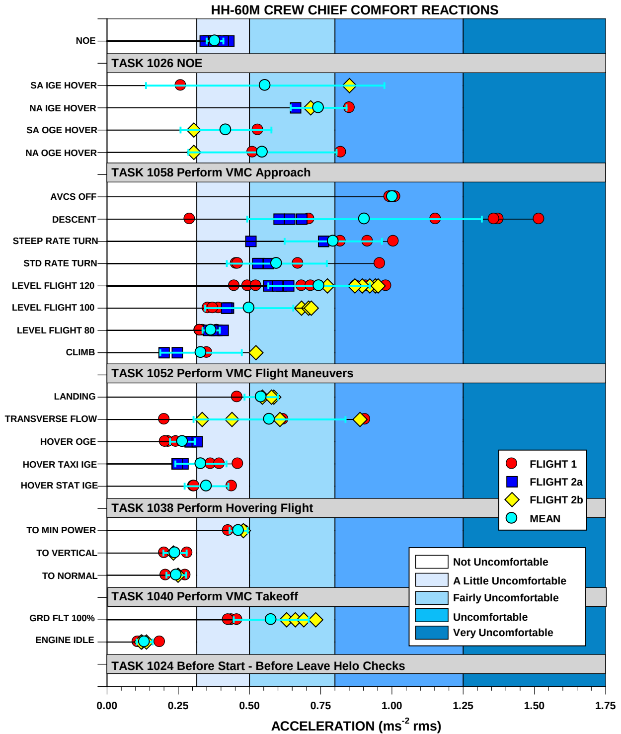
Figure A-25. ISO Comfort Reactions and oVTVs ± One Standard Deviation at the HH-60M Crew Chief Station
