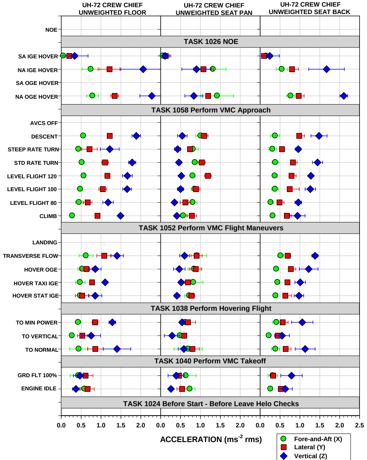
Figure A-8. UH-72 Mean Overall Unweighted Accelerations ± One Standard Deviation at the Crew Chief Station
