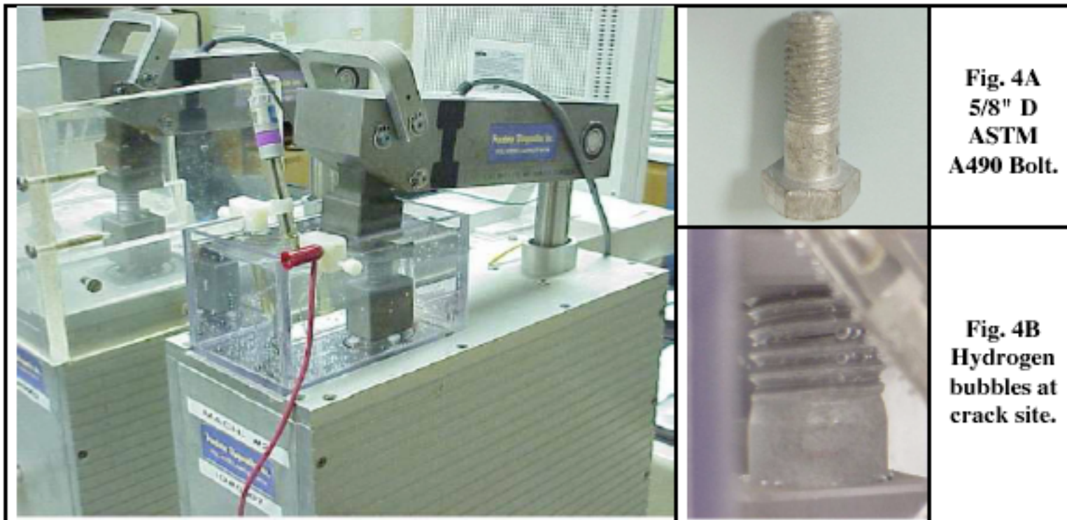
Fig. 4C Fracture Diagnostics International RSL™ (Bend) Test Machine for determination of environmental threshold stress for crack initiation of a zinc coated 5/8" D A490 bolts in hydrogen charging environment.
