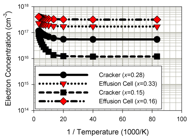
Fig. 5. (Color online) As-grown electron concentration vs temperature for MCS samples grown with both Se sources.
