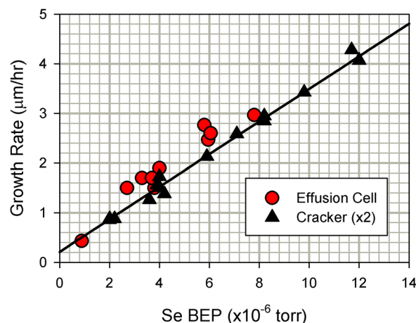
FIG. 2. (Color online) Growth rate vs Se BEP for both the effusion cell ( \text{Se}_6 ) and the cracker source ( \text{Se}_2 ).
