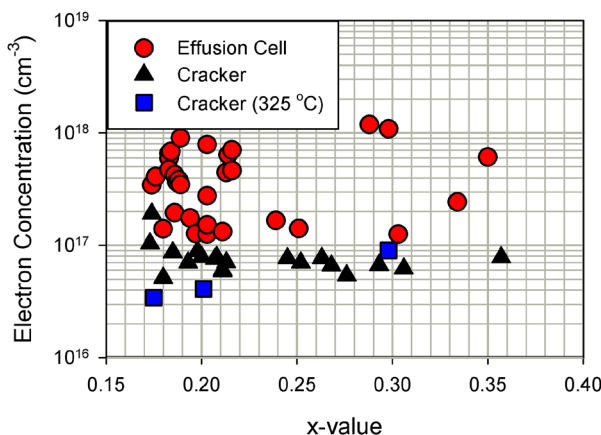
Fig. 6. (Color online) As-grown electron concentration at 77 K vs x -value for the effusion cell ( \text{Se}_6 ), the cracker source at typical operating temperatures ( \text{Se}_2 ), and cracker source with the cracking zone temperature at 325 °C ( \text{Se}_6 ).
