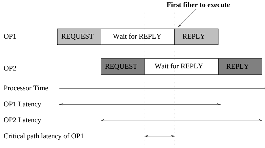
Figure 4.14: Definition of critical path latency.
