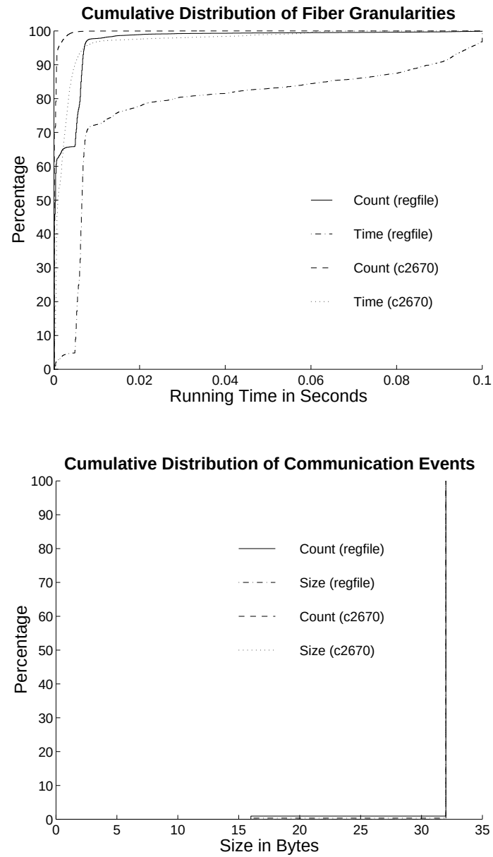
Figure 2.15: Distribution of fibers and communication events for CSWEC. The resolution used for profiling the fiber granularity is 100 microseconds, and the resolution for the communication event size is 16 bytes.
