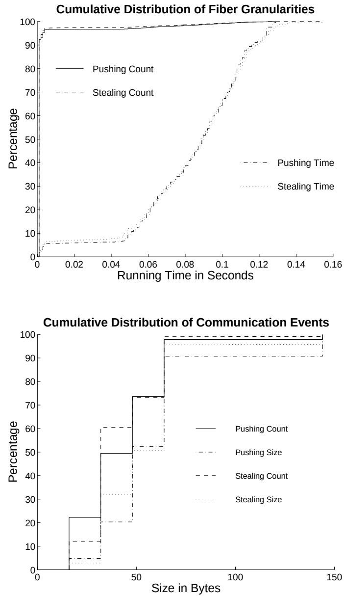
Figure 2.9: Distribution of fibers and communication events for Eigenvalue. The resolution used for profiling the fiber granularity is 1 milliseconds, and the resolution for the communication event size is 16 bytes.
