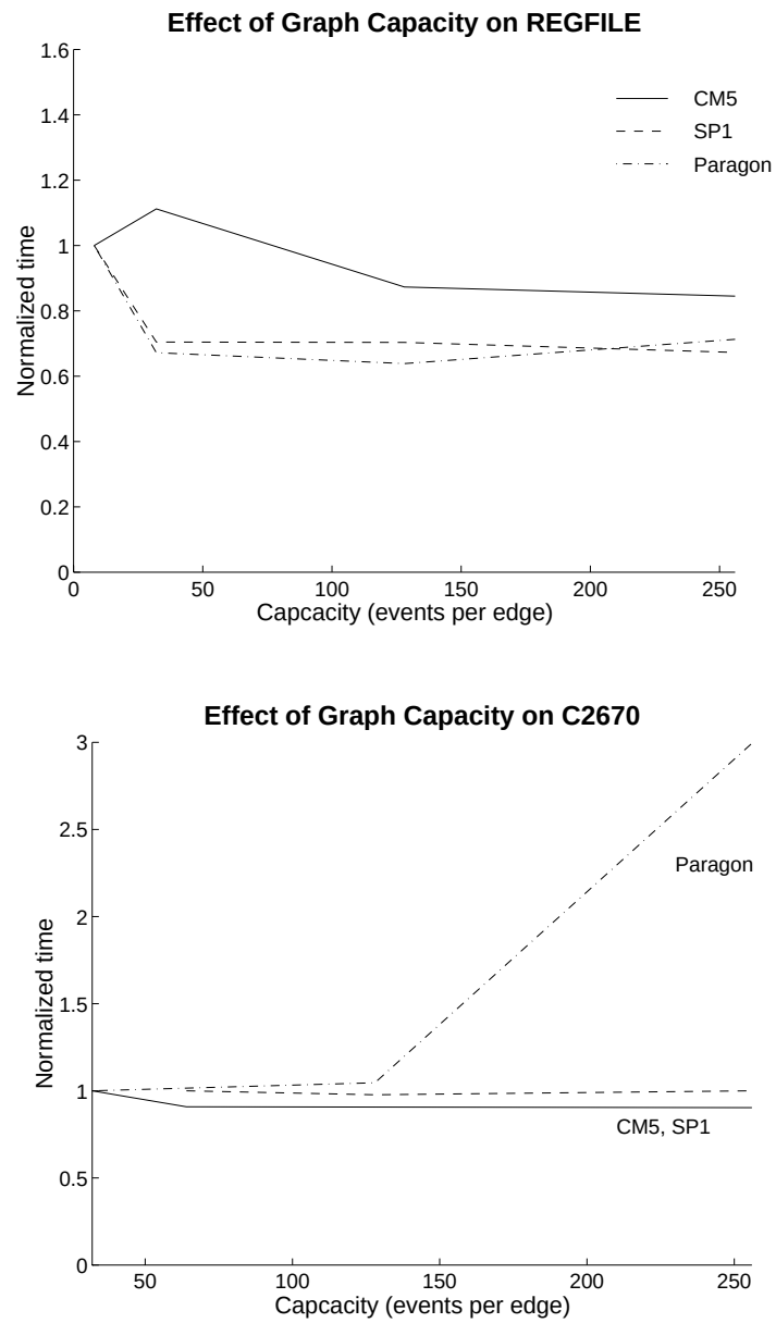
Figure 5.10: Impact of graph capacity on the performance of the CSWEC program. All running times are normalized with respect to the running time with the least capacity.
