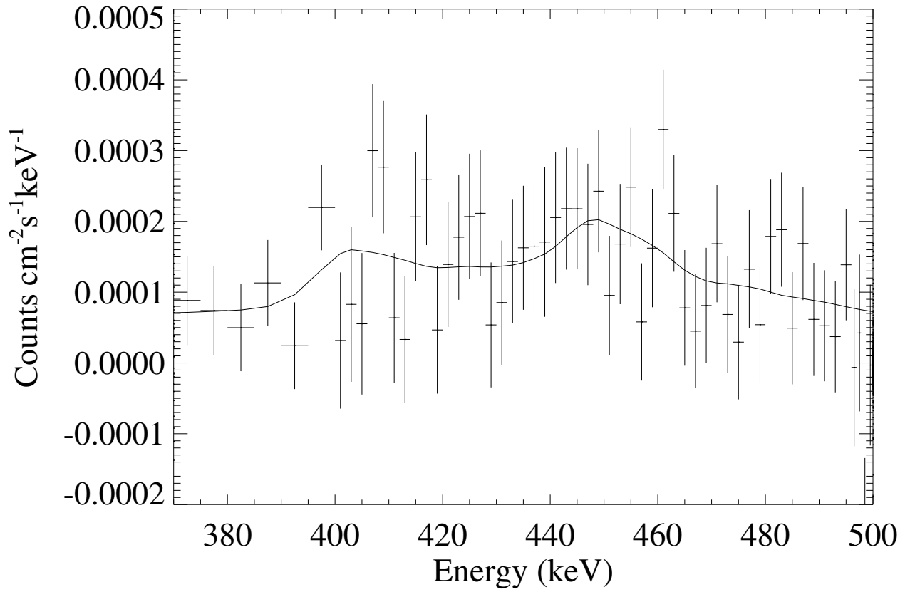
Fig. 3.— Count spectrum of the \alpha - ^4\text{He} line measured by RHESSI derived by subtracting the best-fitting bremsstrahlung and other components found to contribute to the background-corrected spectrum. The curve shows the RHESSI response to the line shape derived for an \alpha -particle distribution that undergoes saturated pitch-angle scattering in the corona for magnetic loops perpendicular to the solar surface at a heliocentric angle of 73^\circ .
