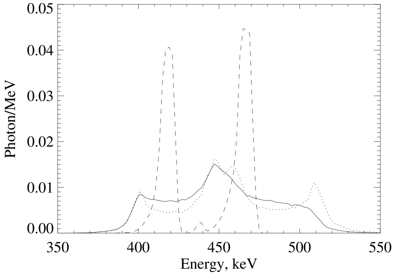
Fig. 2.— Comparison of the calculated \alpha - ^4\text{He} line shapes for a flare at a heliocentric angle of 73^\circ . Solid curve, downward-isotropic distribution (similar to one for \alpha particles undergoing saturated pitch angle scattering in the corona). Dotted curve, fan-beam distribution. Dashed curve, downward beam.
