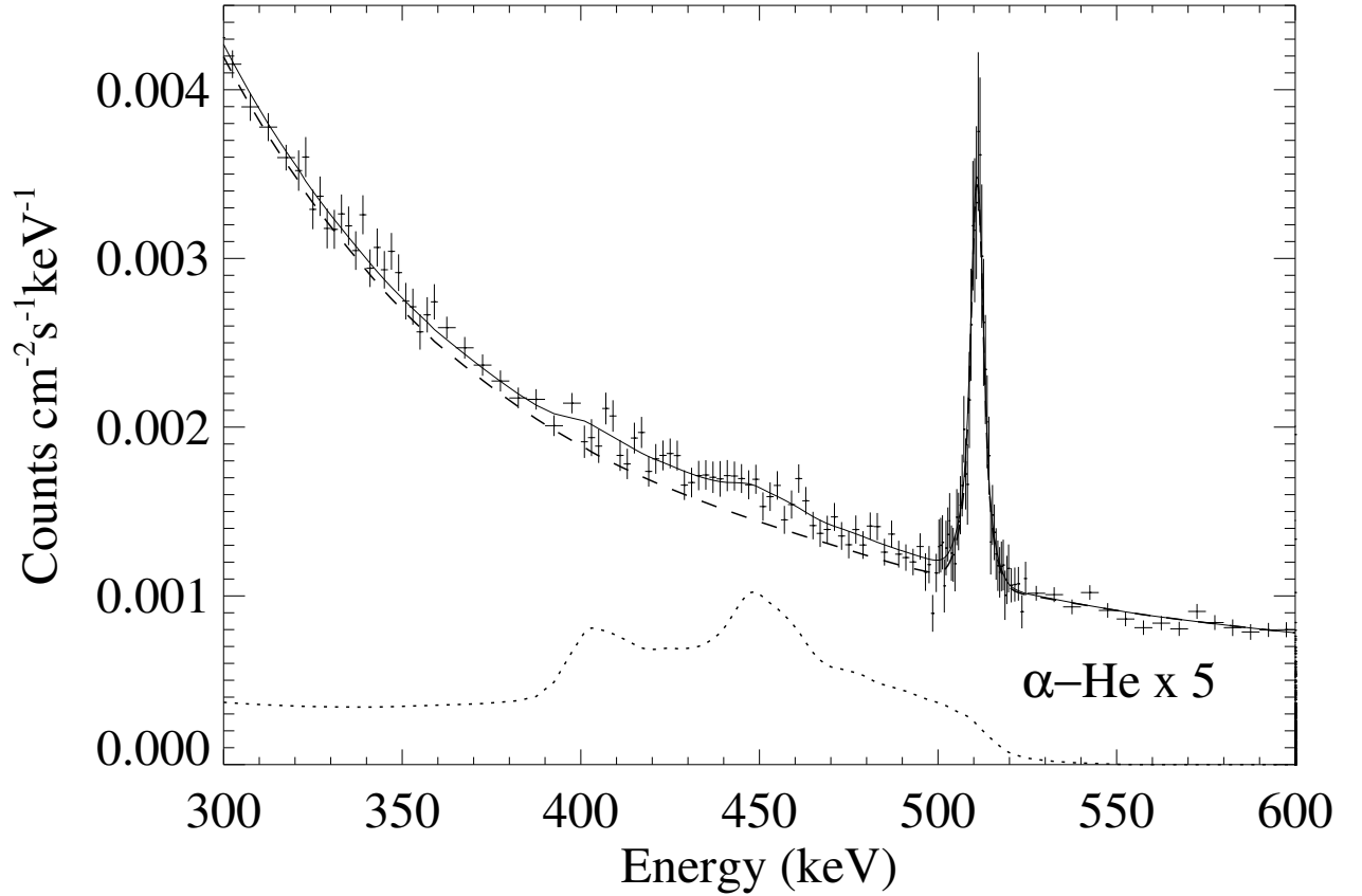
Fig. 1.— Background-corrected count spectrum accumulated from 00:27:20 to 00:43:20 UT. Solid curve is the best fit to the data. Dotted curve shows the RHESSI response to the best-fit \alpha - 4 He line model for an \alpha -particle distribution that undergoes saturated pitch-angle scattering in the corona, multiplied by a factor of 5 for clarity. Dashed curve shows the response to the fitted bremsstrahlung, annihilation, and nuclear- line components (excluding the \alpha - 4 He lines).
