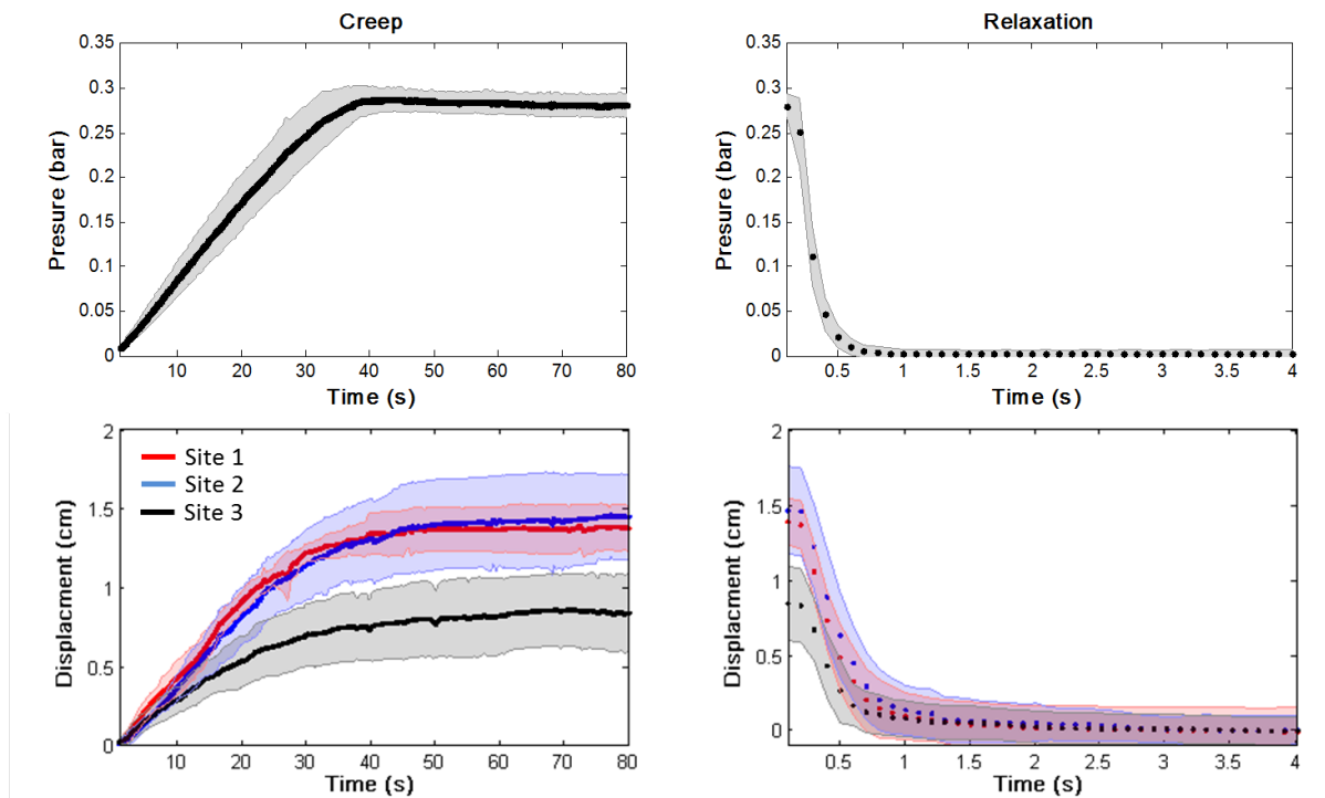
Figure 1 Top: Average pressure loading from all animals and all sites (27 trials), shading shows standard deviation. Bottom: Average displacement data from all animals at each site (9 trials each), shading shows standard deviation.
